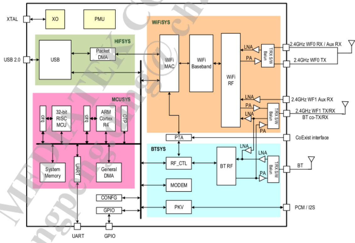
Figure 1 WF-M38G-UTH1 Block Diagram
