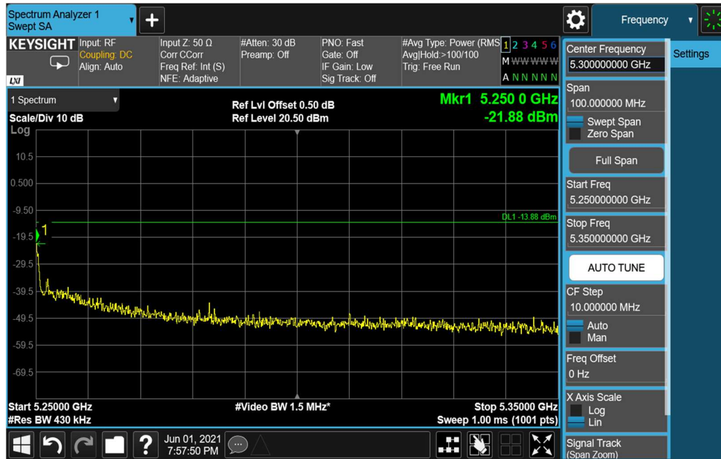
11n20 5240 Ant 0
