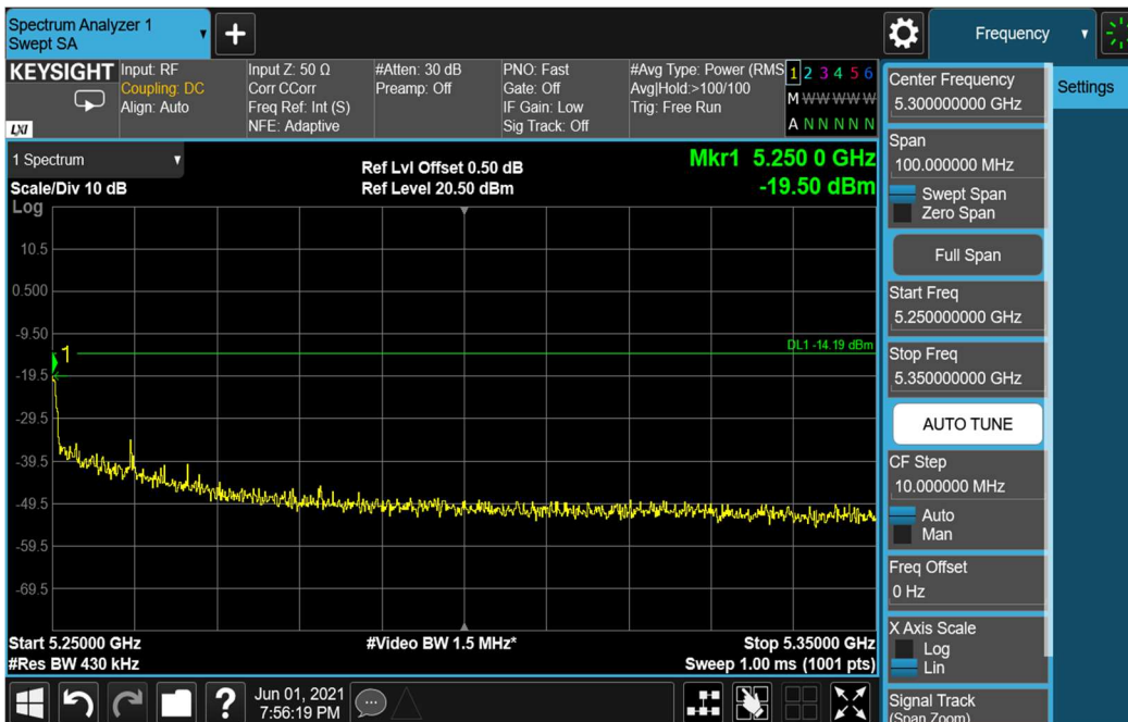
11n20 5240 Ant 0
