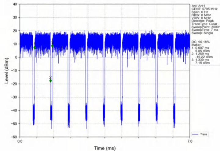
802.11ac(VHT40)_HCH_5795MHz_Ant1_NTNV
