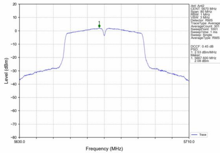
802.11ac(VHT40)_HCH_5670MHz_MIMO_NTNV
