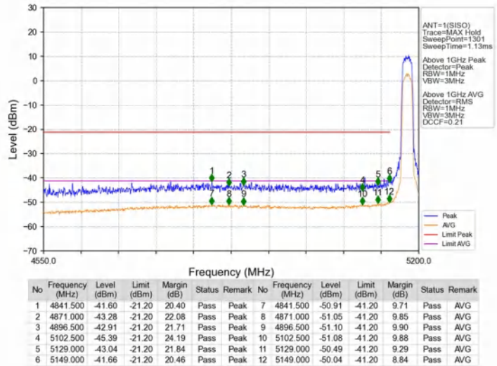
802.11a_LCH_5180MHz_Ant1_NTNV
