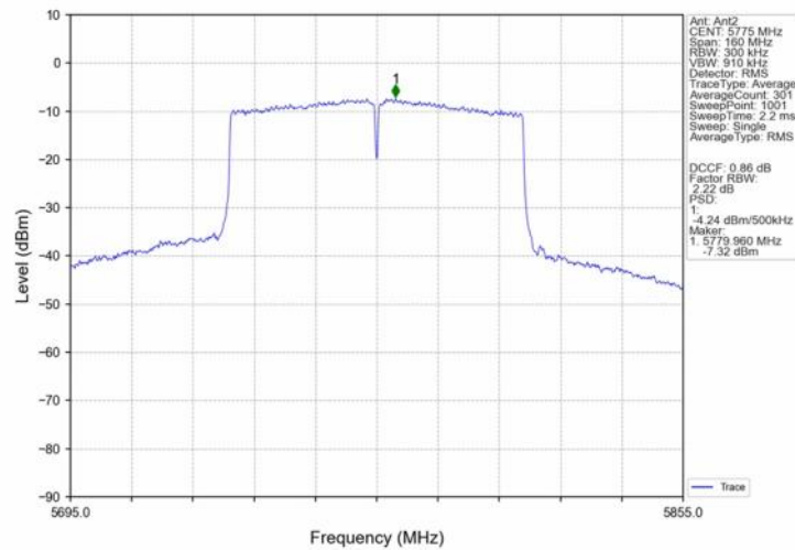
802.11ac(VHT80)_MCH_5775MHz_Ant2_NTNV
