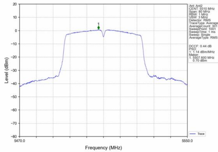
802.11ac(VHT40)_LCH_5510MHz_MIMO_NTNV
