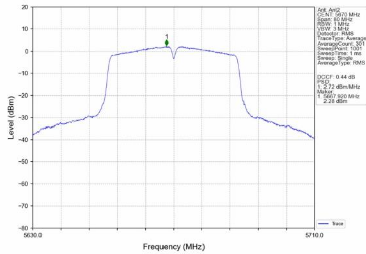
802.11n(HT40)_HCH_5670MHz_MIMO_NTNV
