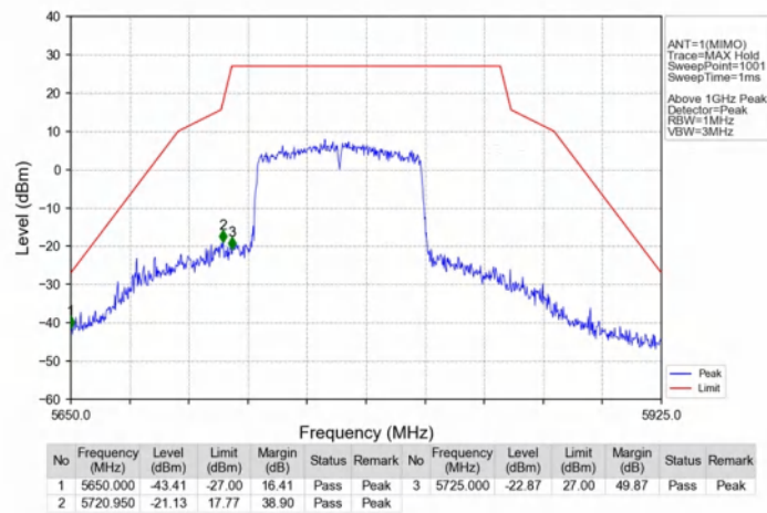
802.11ac(VHT80)_MCH_5775MHz_Ant1_NTNV
