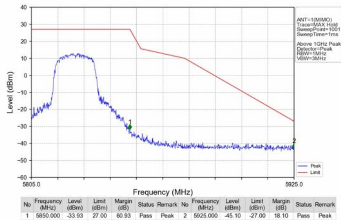
802.11ac(VHT20)_HCH_5825MHz_Ant1_NTNV
