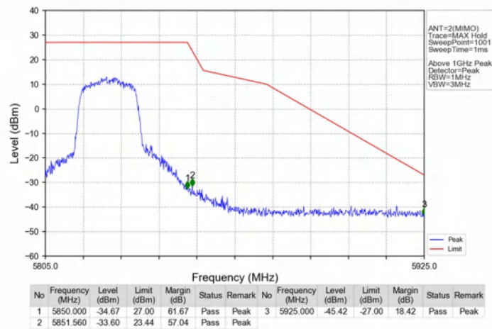
802.11ac(VHT20)_HCH_5825MHz_Ant2_NTNV
