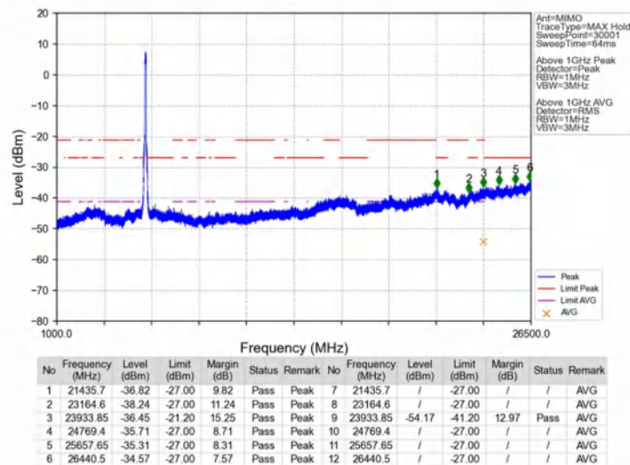
802.11ac(VHT80)_MCH_5775MHz_MIMO_NTNV
