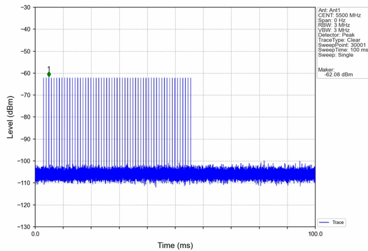
Signal Calibration 802.11n(HT20) 2C 5500MHz RadarType1 Trial0
