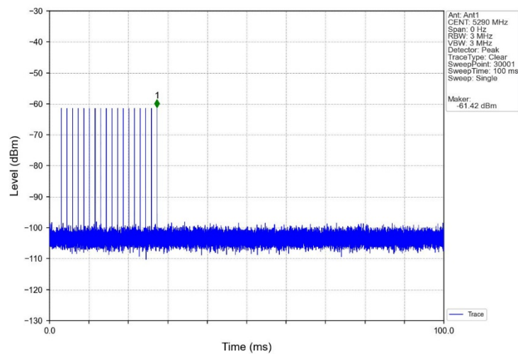
Signal Calibration 802.11ac(HT80) 2A 5290MHz RadarType1 Trial0
