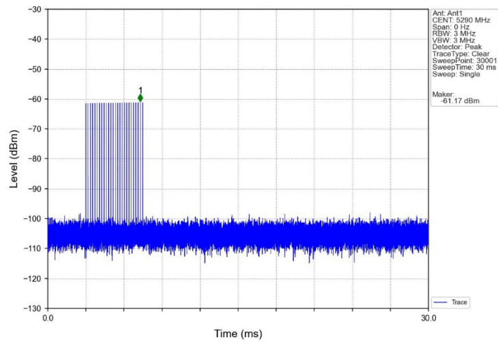
Signal Calibration_802.11ac(HT80)_2A_5290MHz_RadarType3_Trial0
