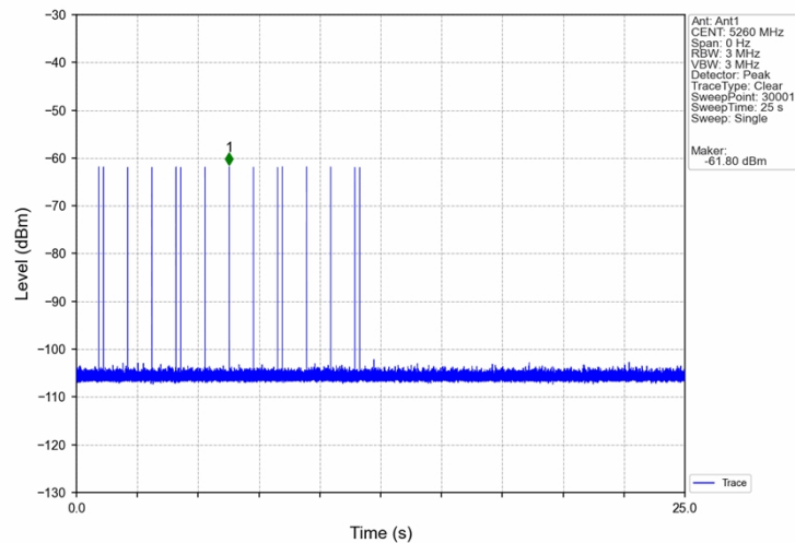
Signal Calibration_802.11n(HT20)_2A_5260MHz_RadarType5_Trial0
