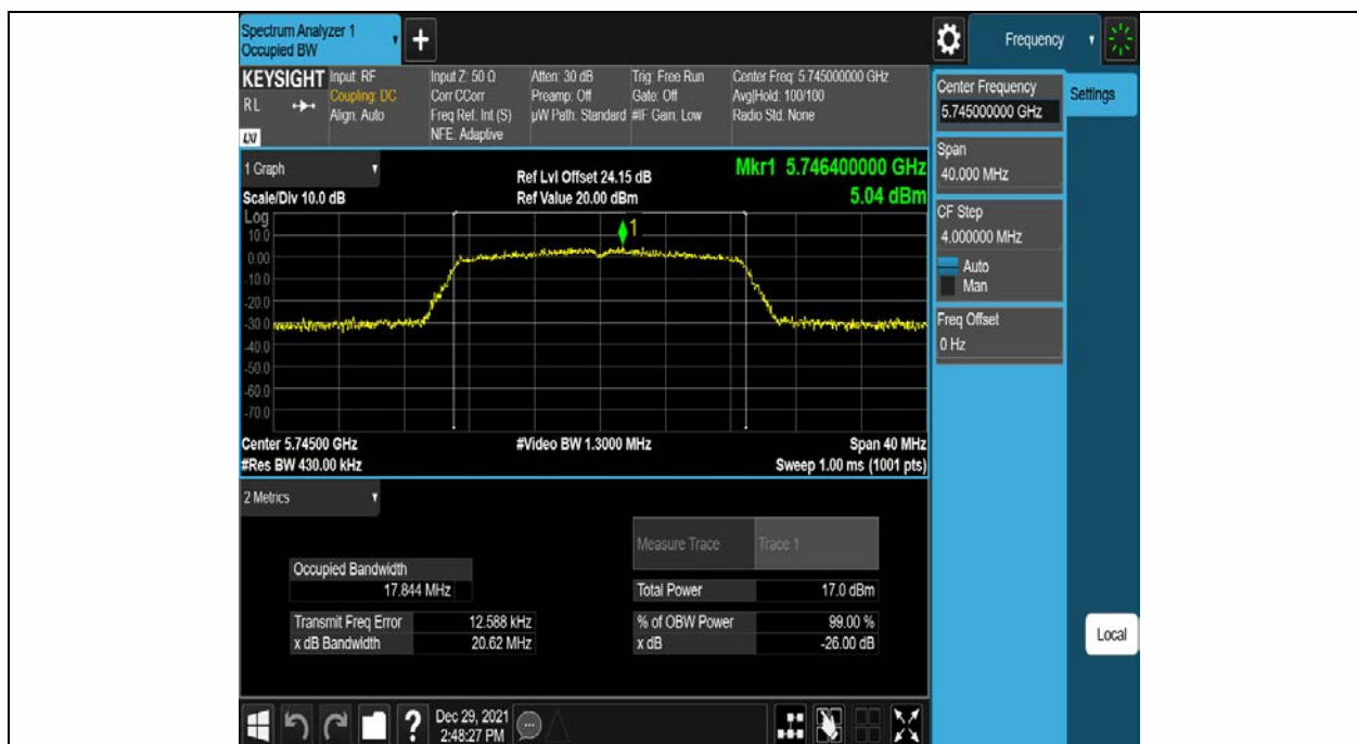
11N20SISO Ant1 5745
