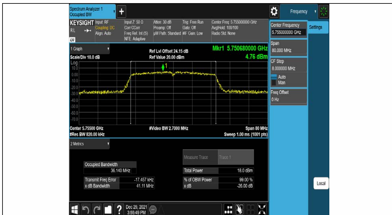
11AC40SISO Ant1 5755
