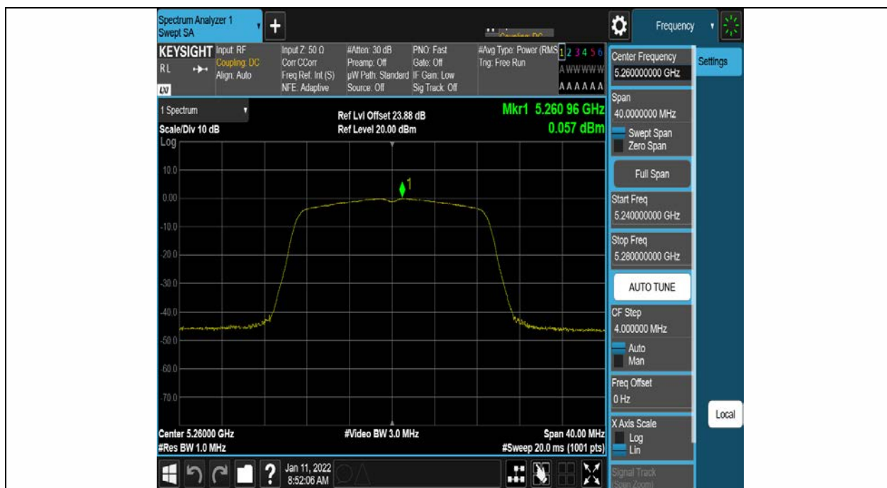
11N20SISO Ant1 5260
