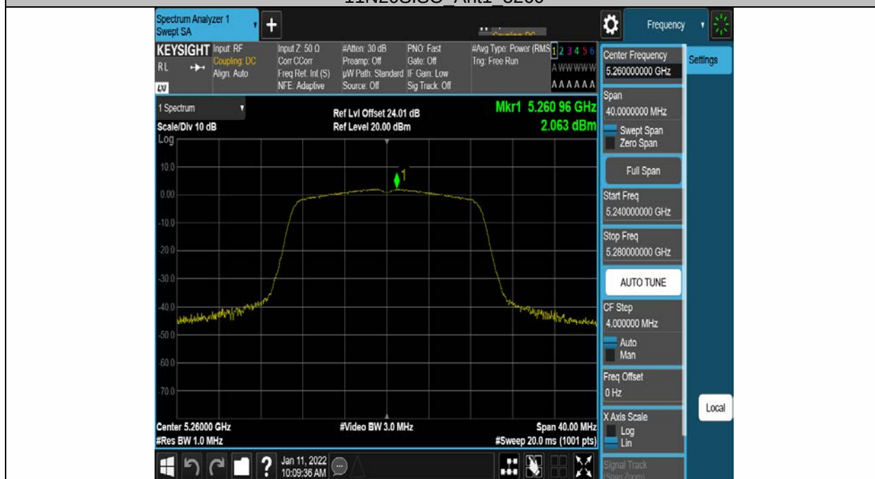
11N20SISO Ant2 5260
