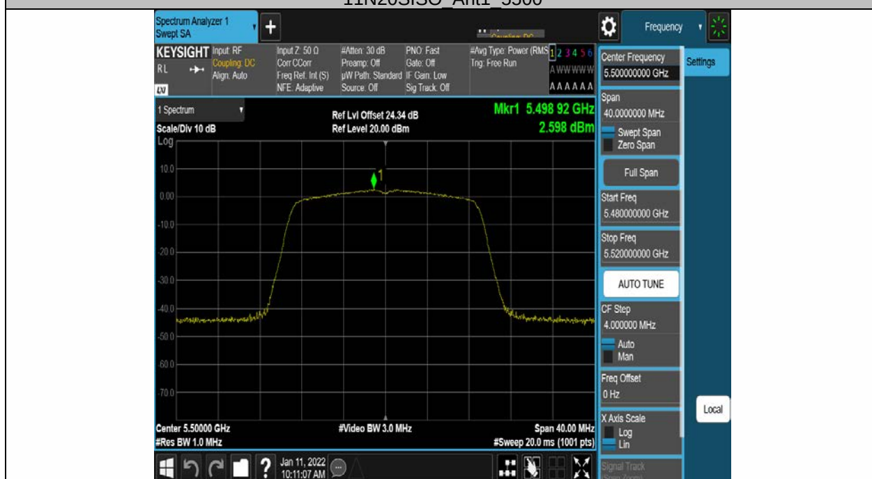
11N20SISO Ant2 5500
