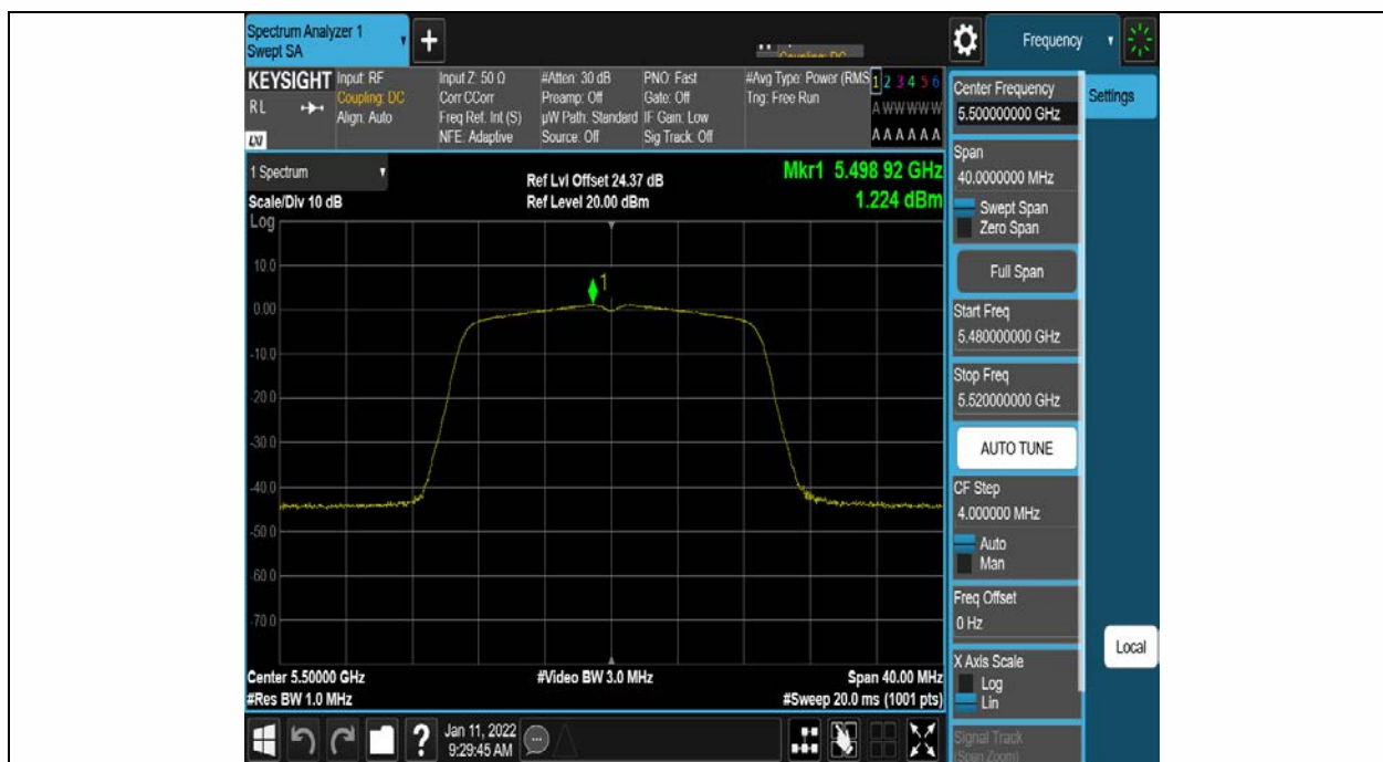
11AC20SISO Ant1 5500
