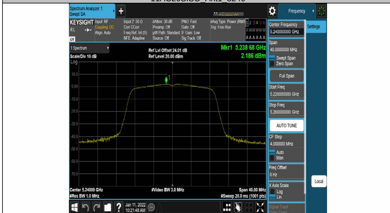
11AC20SISO Ant2 5240
