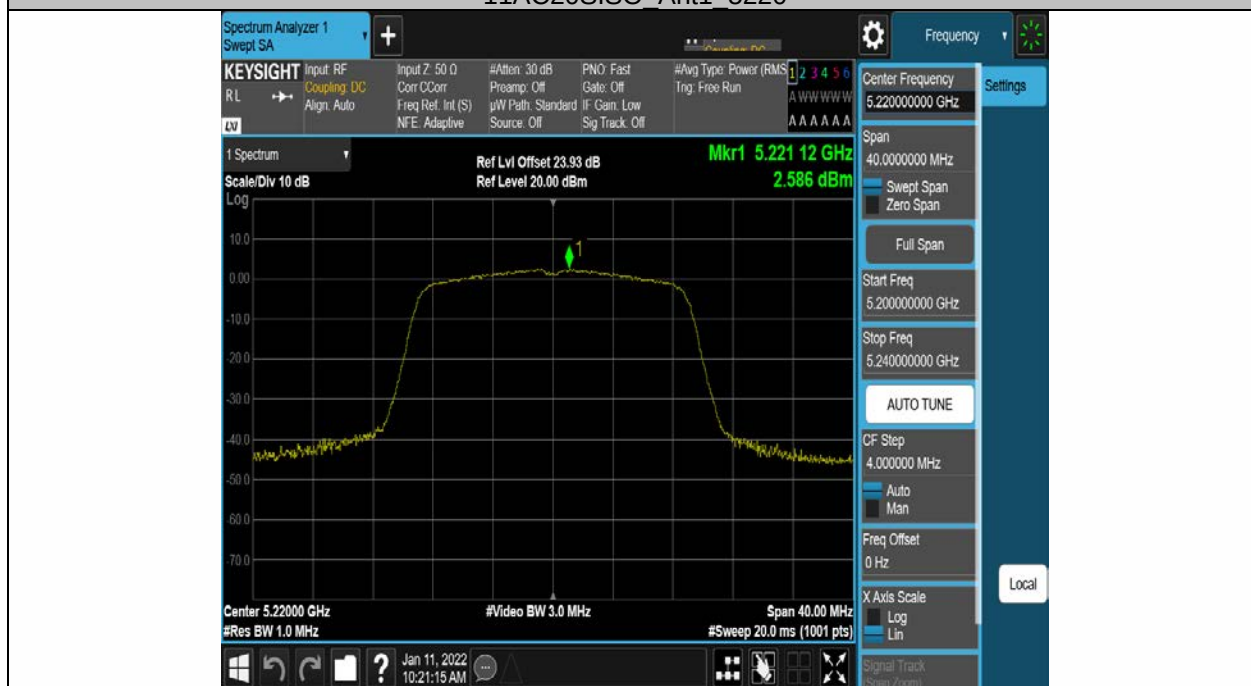
11AC20SISO Ant2 5220
