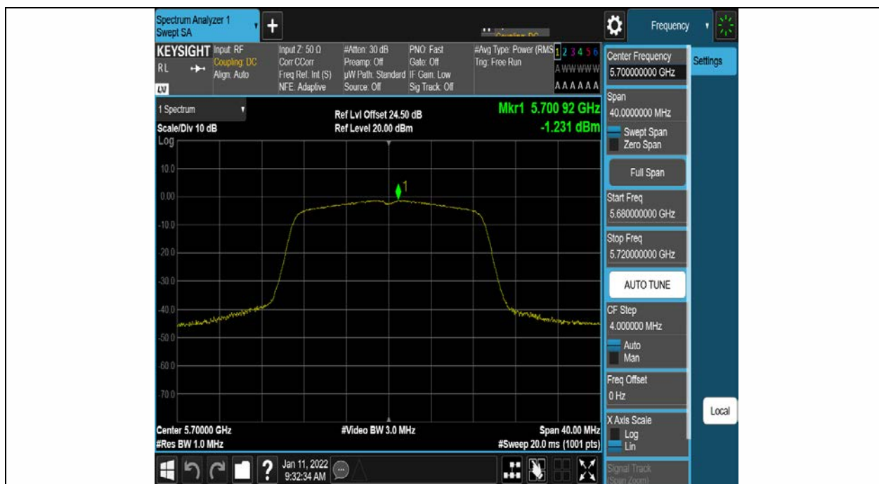
11AC20SISO Ant1 5700
