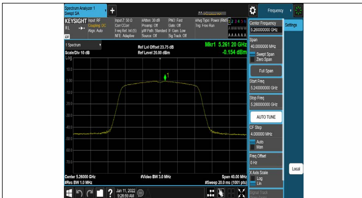
11AC20SISO Ant1 5260
