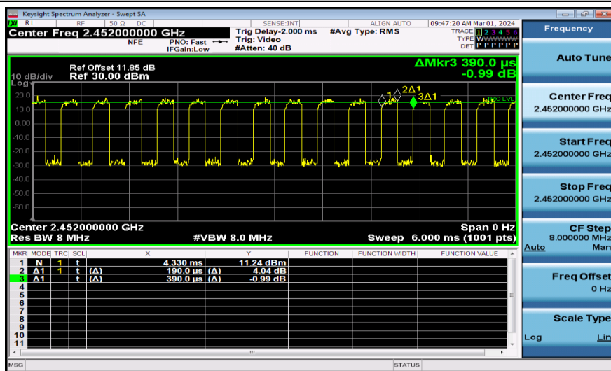
NTNV-11AX40MIMO-Ant2-2452
