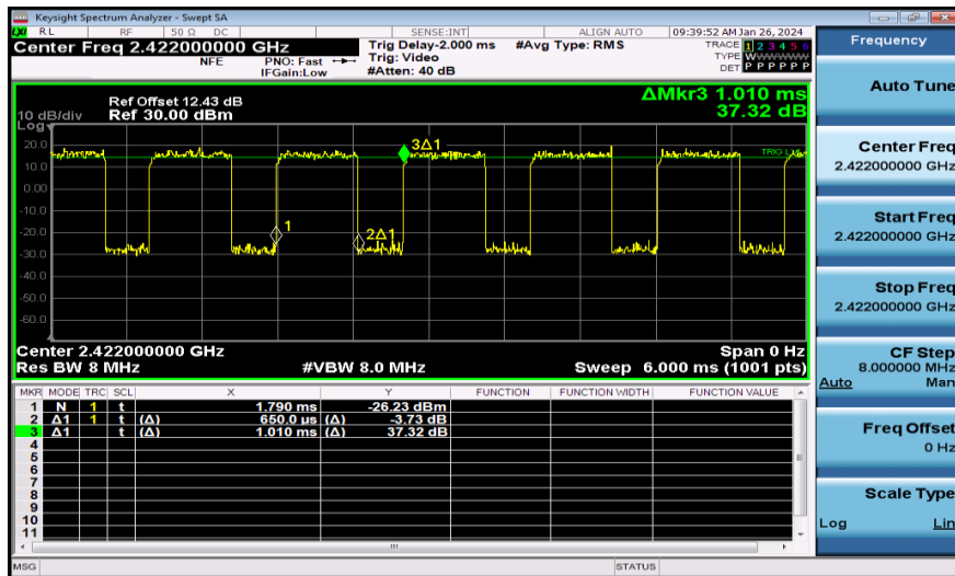
NTNV-11N40MIMO-Ant2-2422
