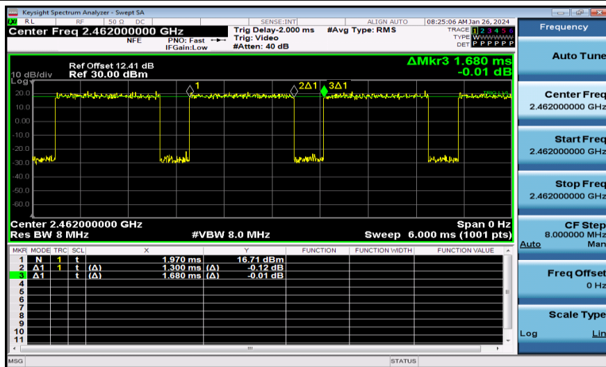
NTNV-11N20MIMO-Ant2-2462
