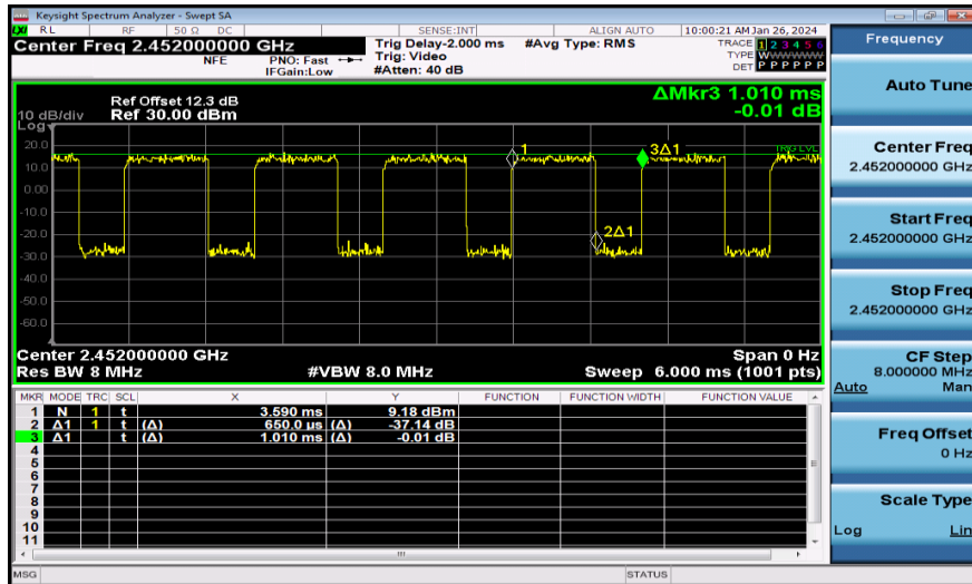
NTNV-11N40MIMO-Ant1-2452
