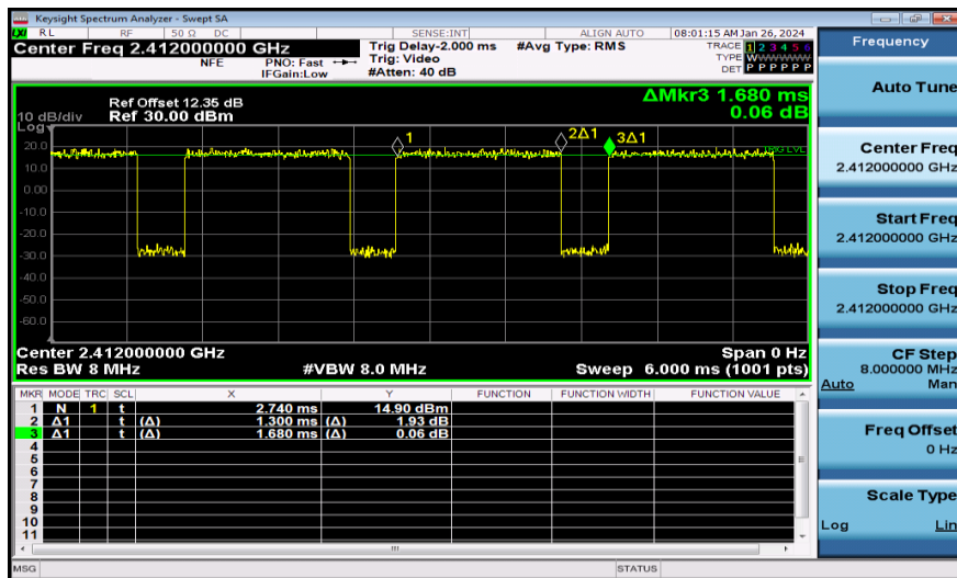
NTNV-11N20MIMO-Ant1-2412
