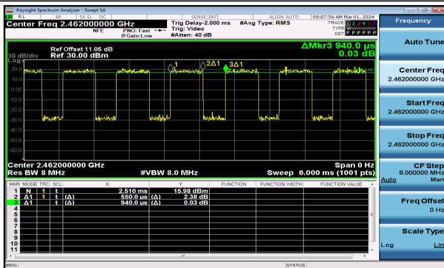
NTNV-11AX20MIMO-Ant2-2462
