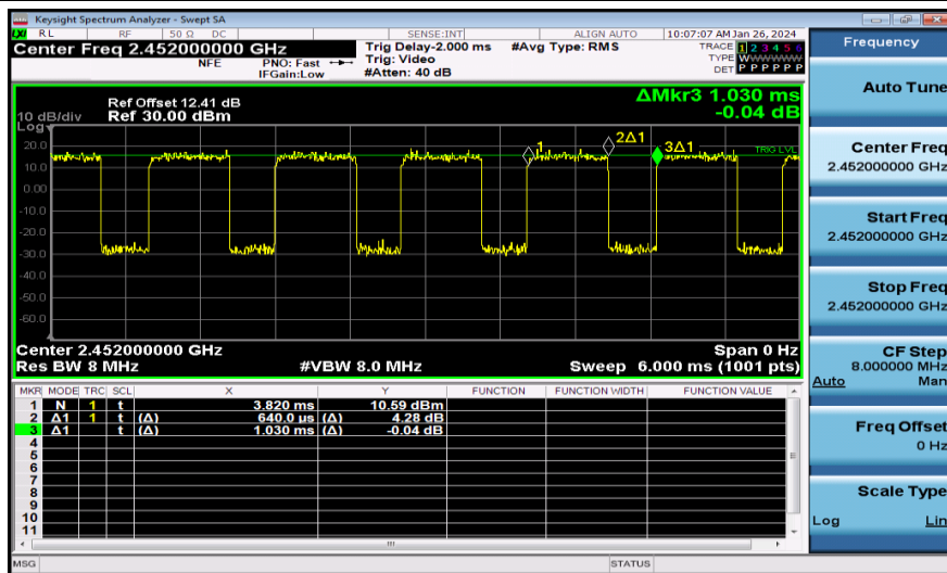
NTNV-11N40MIMO-Ant2-2452
