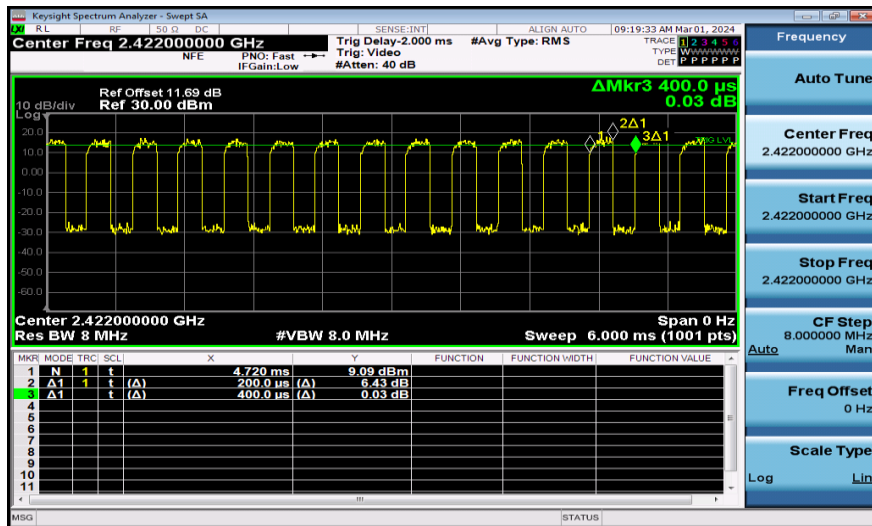
NTNV-11AX40MIMO-Ant2-2422
