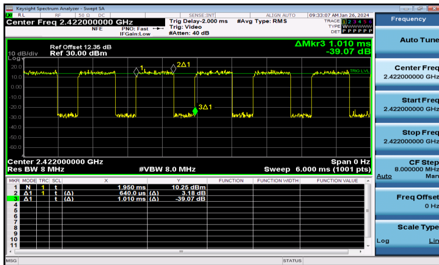
NTNV-11N40MIMO-Ant1-2422
