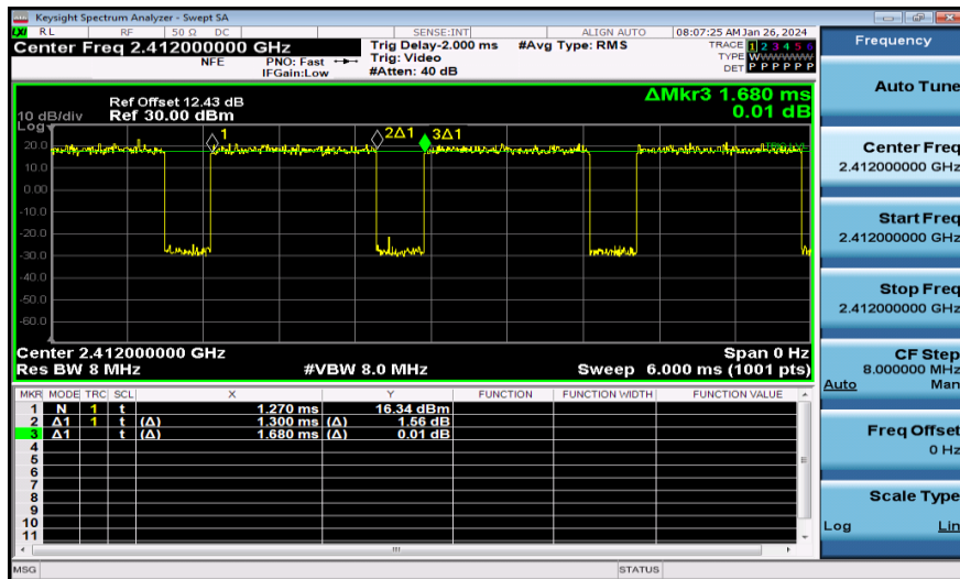
NTNV-11N20MIMO-Ant2-2412
