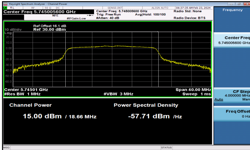
11AC20MIMO-Ant1-5745-PASS
