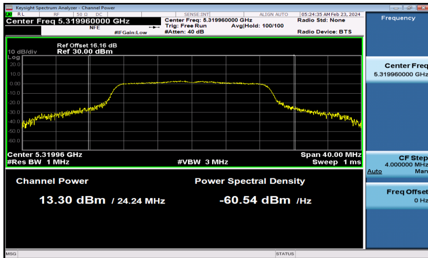
11AC20MIMO-Ant1-5320-PASS
