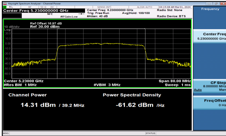
11AX40MIMO-Ant2-5230-PASS
