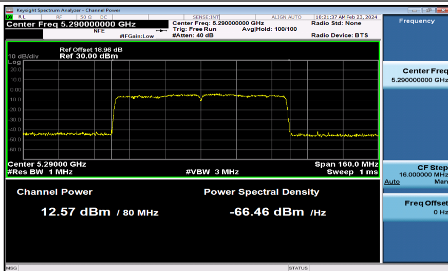
11AC80MIMO-Ant1-5290-PASS
