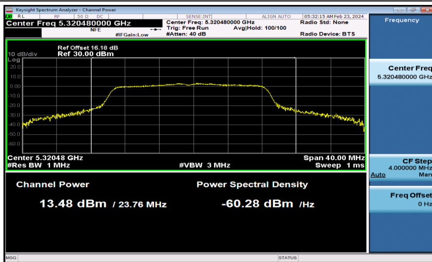
11AC20MIMO-Ant2-5320-PASS
