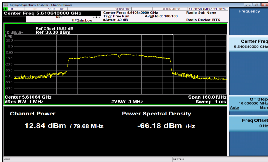
11AC80MIMO-Ant2-5610-PASS
