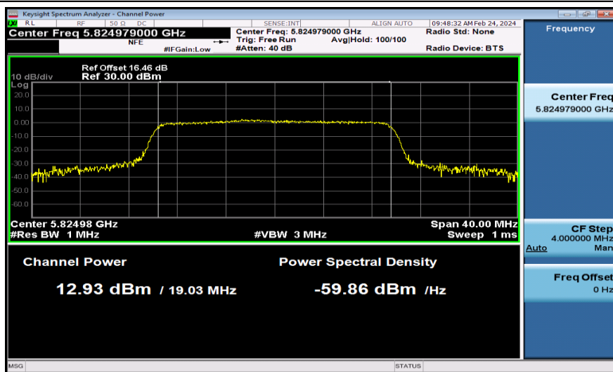
11AX20MIMO-Ant1-5825-PASS
