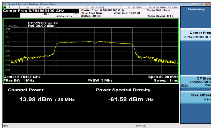
11AC40MIMO-Ant2-5755-PASS
