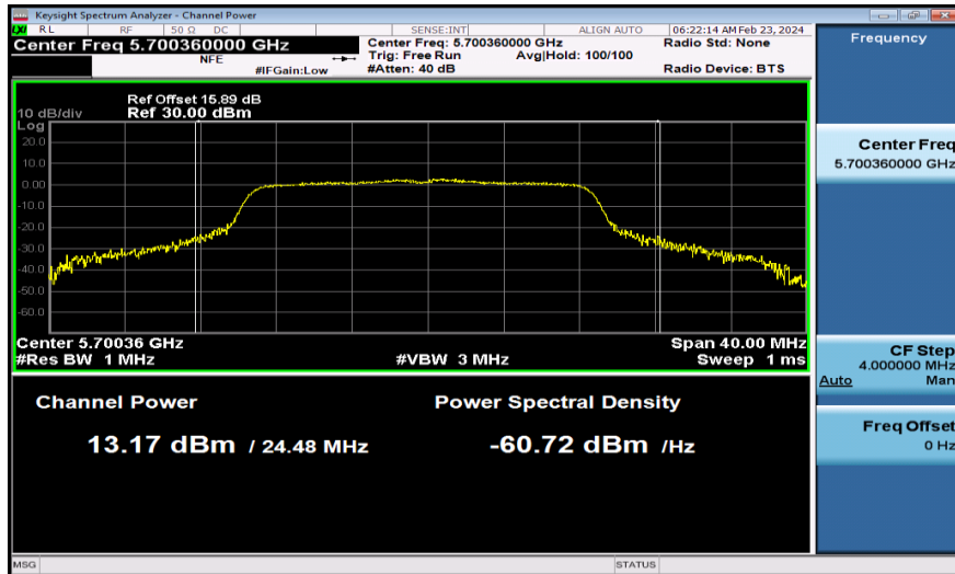
11AC20MIMO-Ant1-5700-PASS
