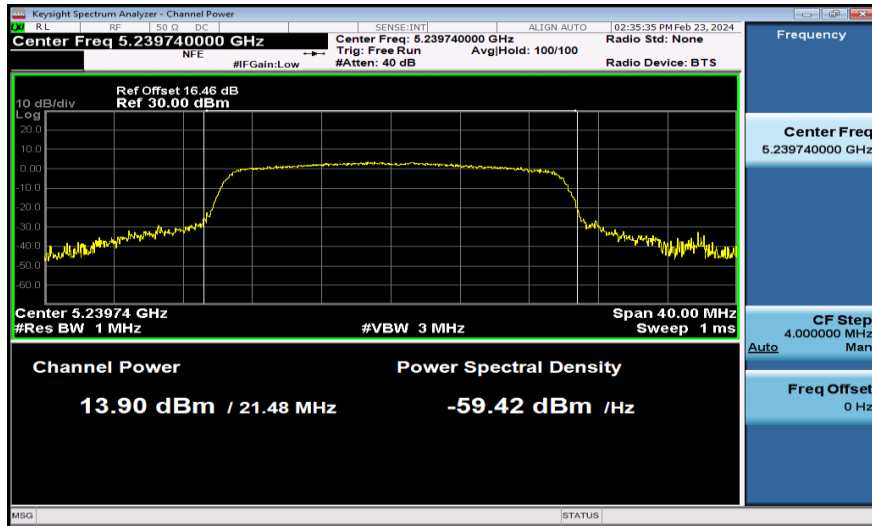
11AX20MIMO-Ant2-5240-PASS
