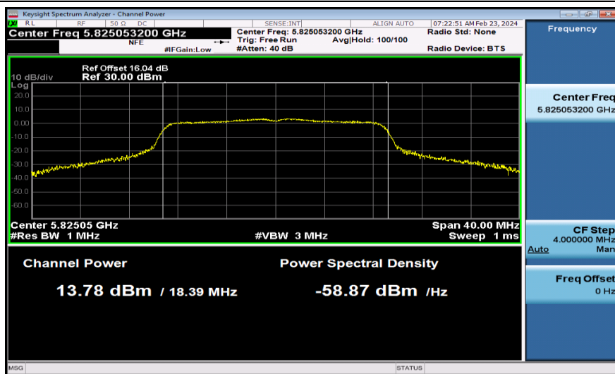
11AC20MIMO-Ant2-5825-PASS
