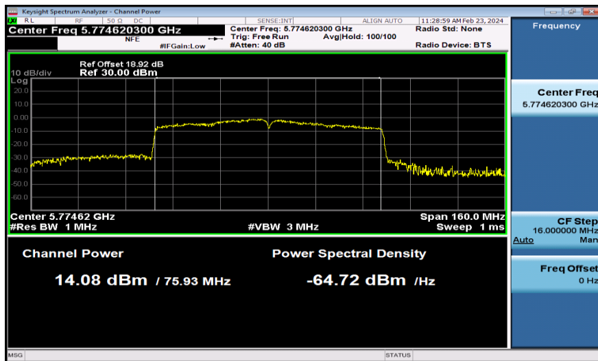
11AC80MIMO-Ant2-5775-PASS
