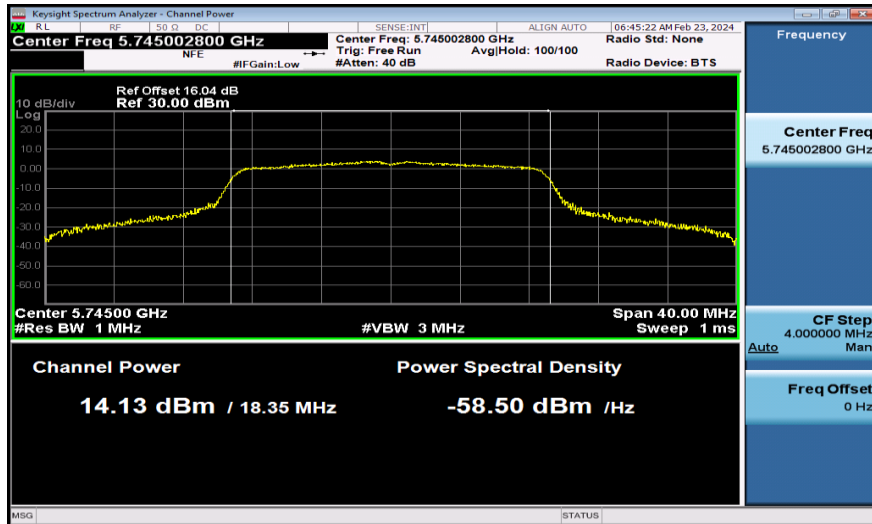
11AC20MIMO-Ant2-5745-PASS
