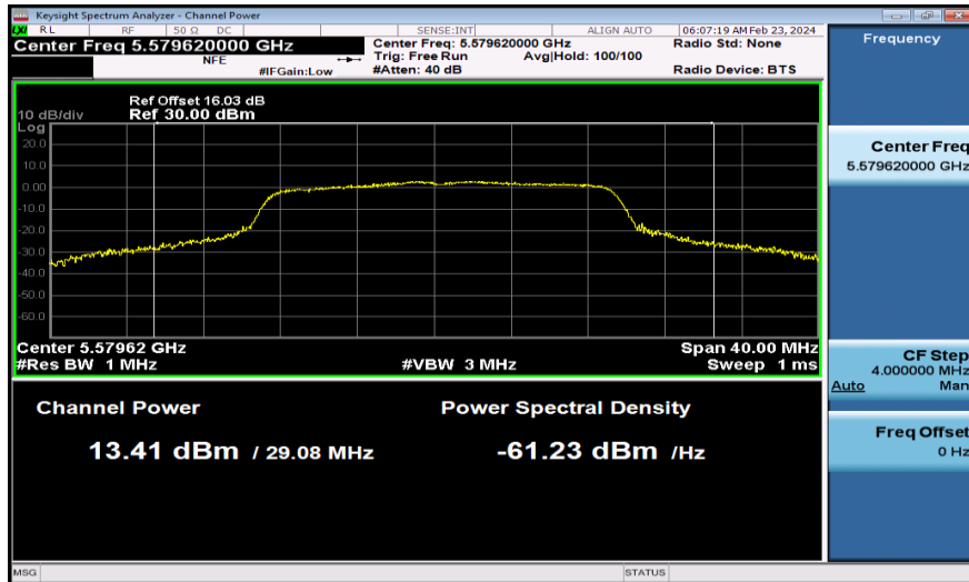
11AC20MIMO-Ant2-5580-PASS
