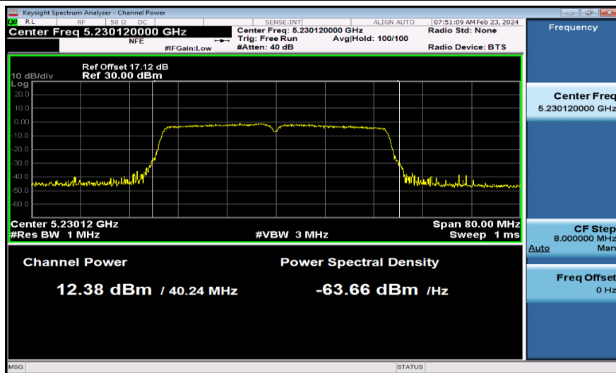
11AC40MIMO-Ant1-5230-PASS
