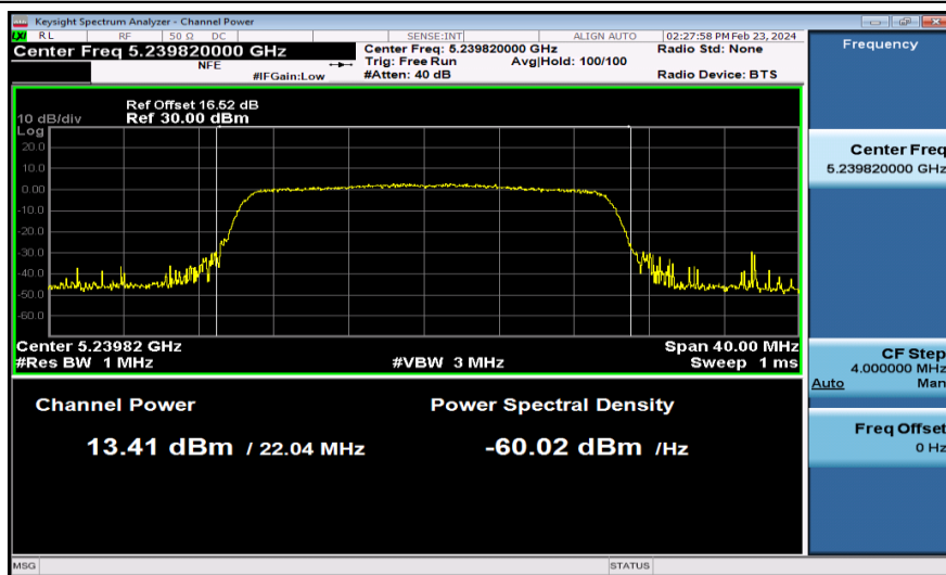
11AX20MIMO-Ant1-5240-PASS
