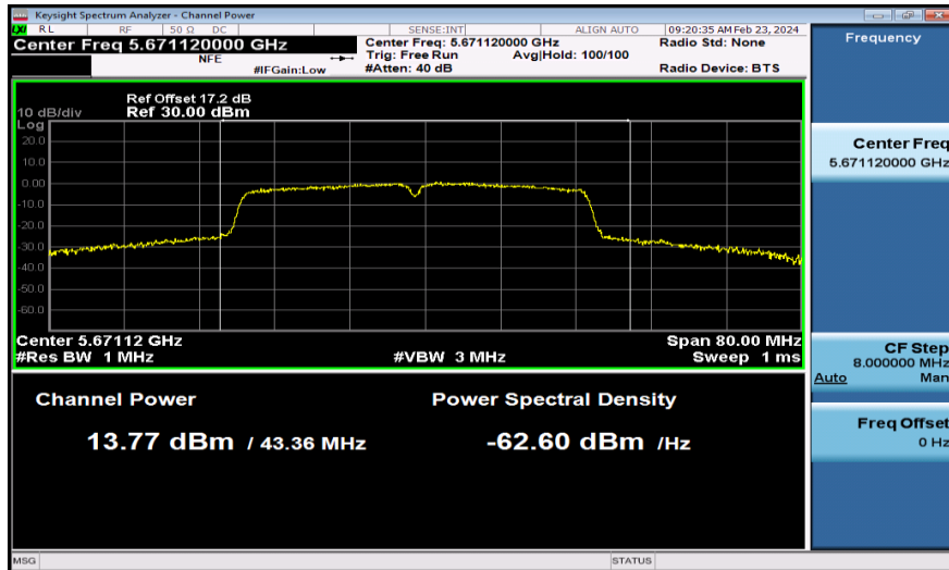
11AC40MIMO-Ant2-5670-PASS
