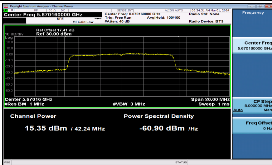
11AX40MIMO-Ant2-5670-PASS
