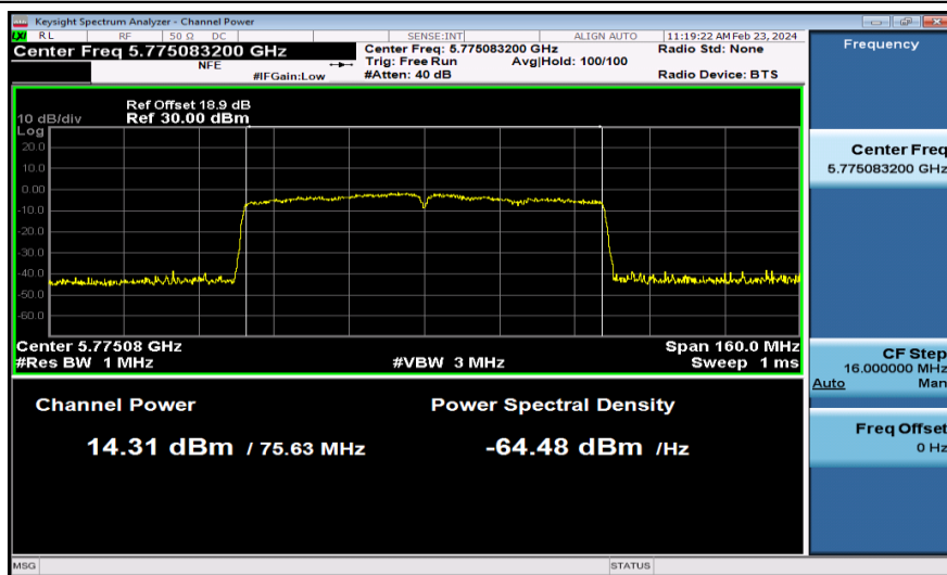
11AC80MIMO-Ant1-5775-PASS
