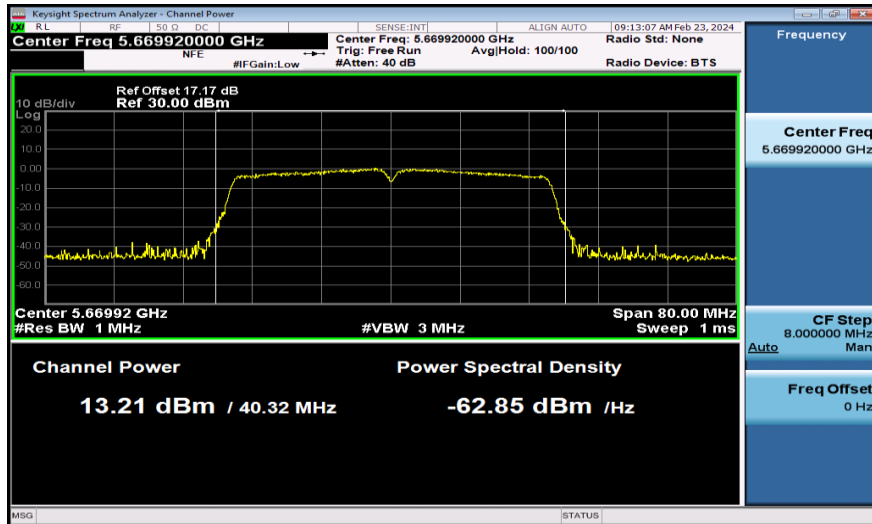
11AC40MIMO-Ant1-5670-PASS
