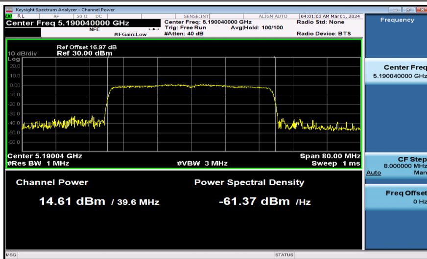
11AX40MIMO-Ant2-5190-PASS
