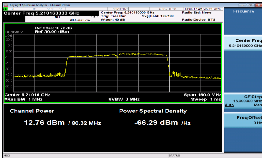
11AC80MIMO-Ant1-5210-PASS
