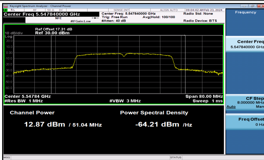
11AC40MIMO-Ant2-5550-PASS
