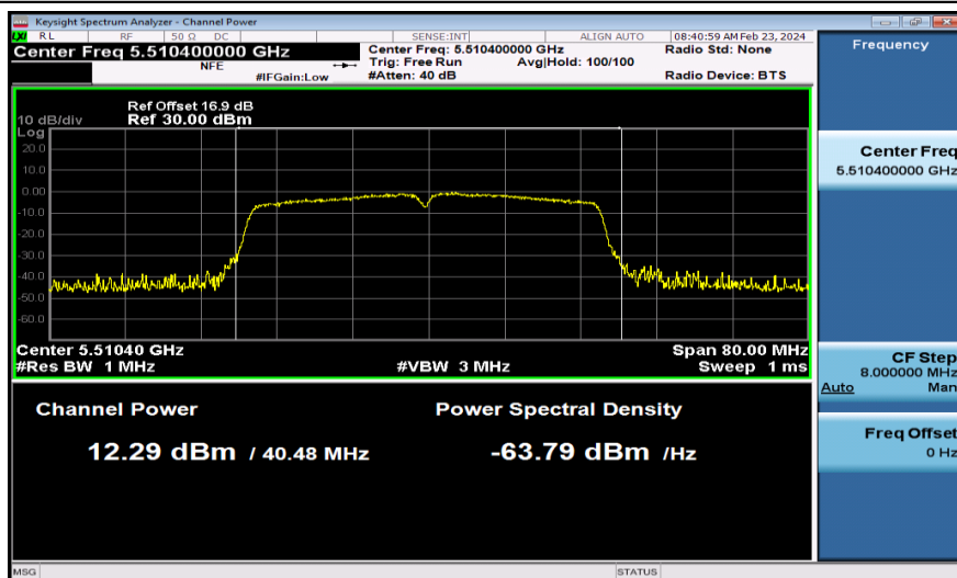
11AC40MIMO-Ant1-5510-PASS
