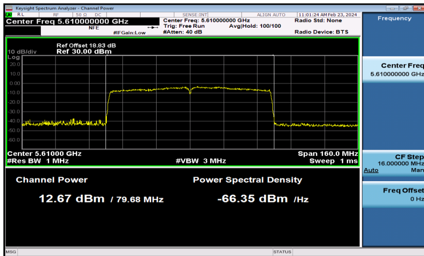
11AC80MIMO-Ant1-5610-PASS
