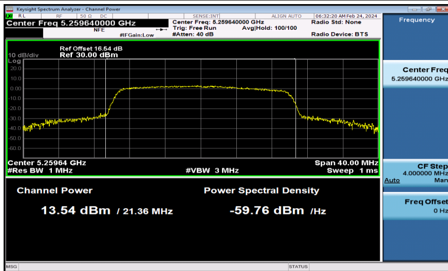
11AX20MIMO-Ant2-5260-PASS
