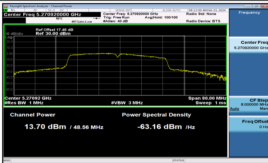
11AC40MIMO-Ant2-5270-PASS
