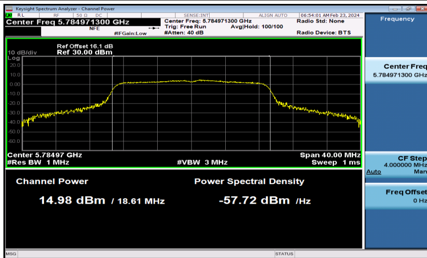
11AC20MIMO-Ant1-5785-PASS
