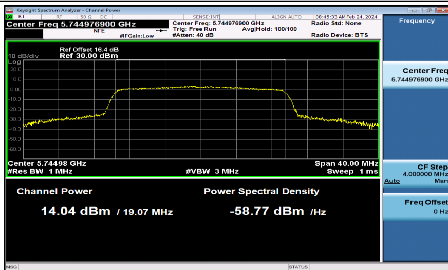
11AX20MIMO-Ant2-5745-PASS
