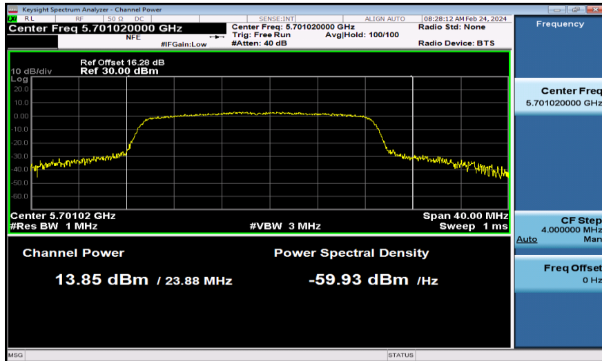
11AX20MIMO-Ant2-5700-PASS
