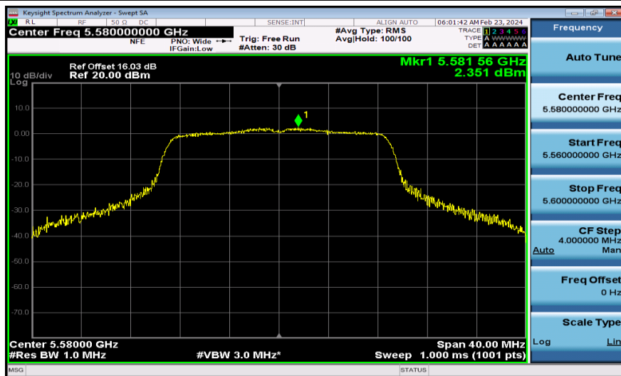
11AC20MIMO-Ant1-5580-PASS
