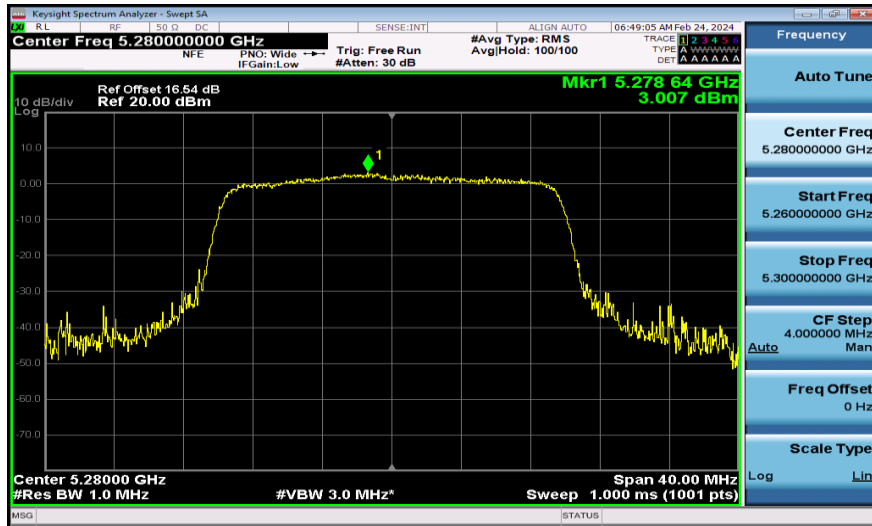
11AX20MIMO-Ant2-5280-PASS
