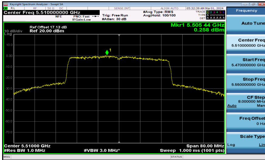
11AX40MIMO-Ant2-5510-PASS
