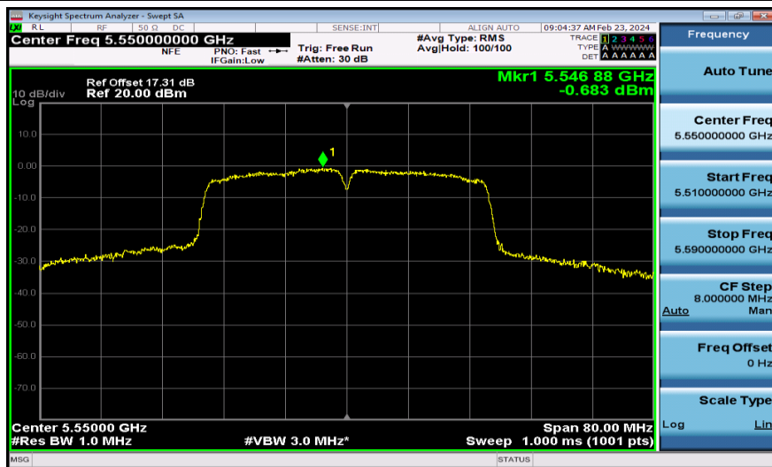
11AC40MIMO-Ant2-5550-PASS
