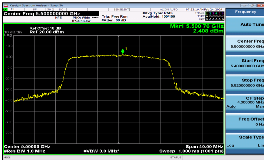
11AX20MIMO-Ant2-5500-PASS
