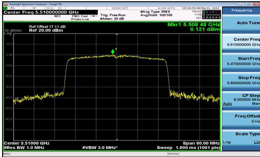
11AX40MIMO-Ant1-5510-PASS
