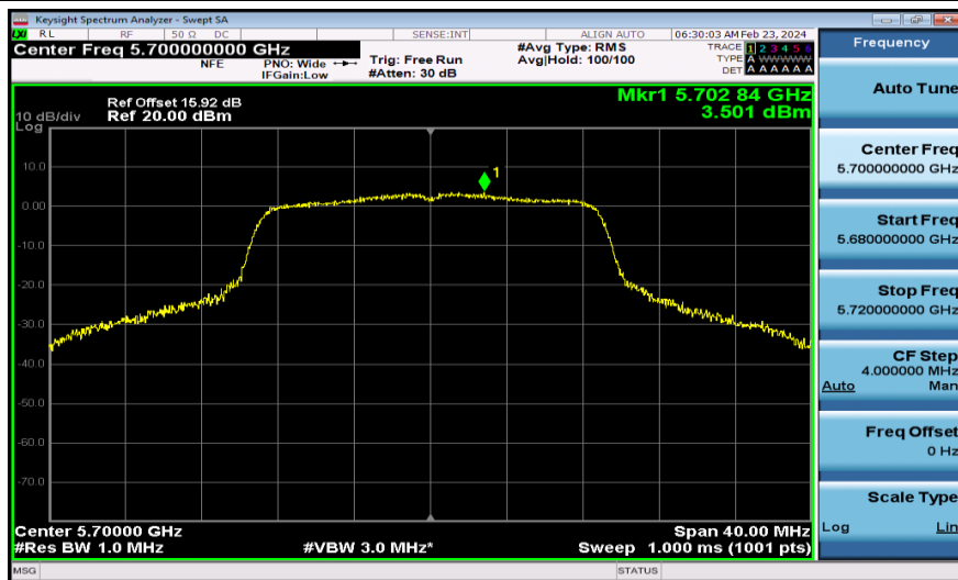
11AC20MIMO-Ant2-5700-PASS
