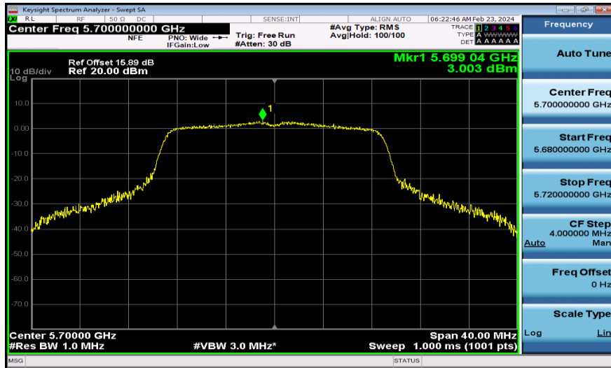
11AC20MIMO-Ant1-5700-PASS
