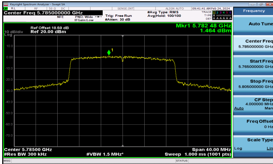
11AX20MIMO-Ant2-5785-PASS
