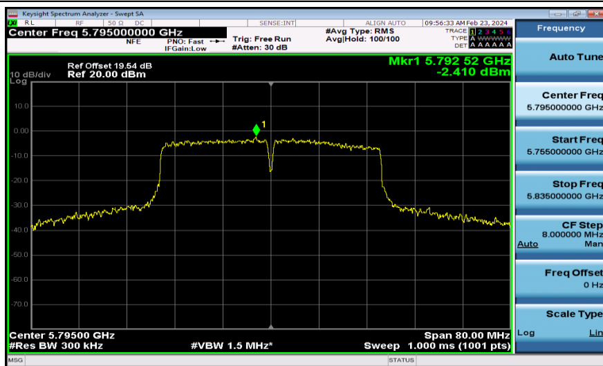
11AC40MIMO-Ant2-5795-PASS
