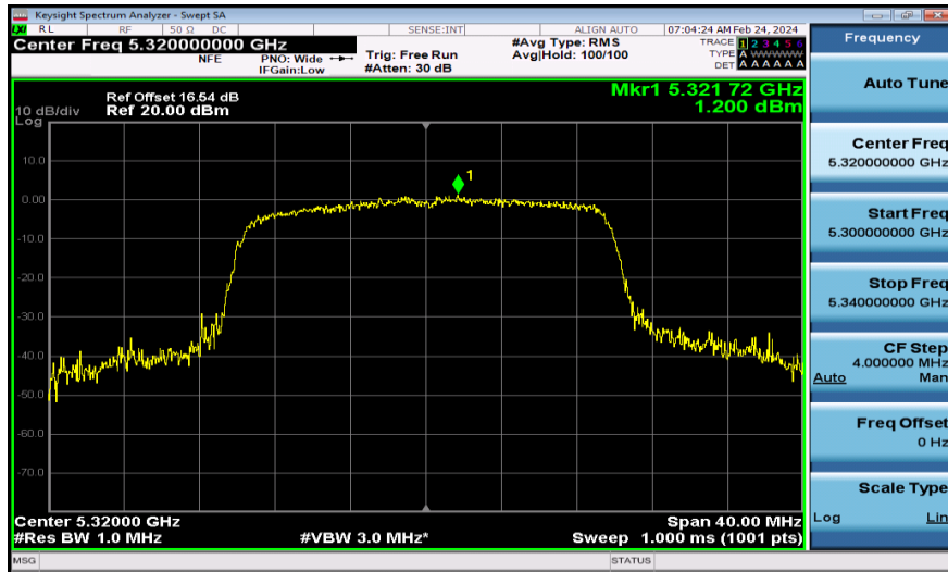
11AX20MIMO-Ant2-5320-PASS
