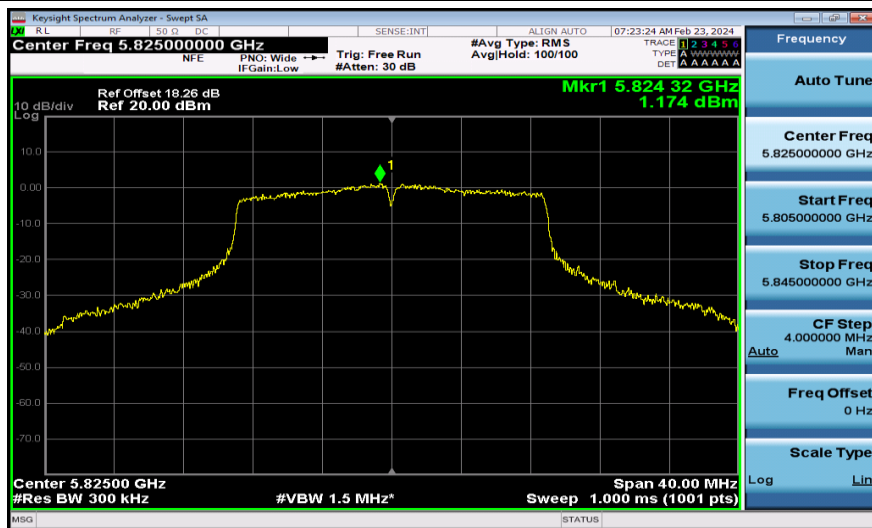
11AC20MIMO-Ant2-5825-PASS
