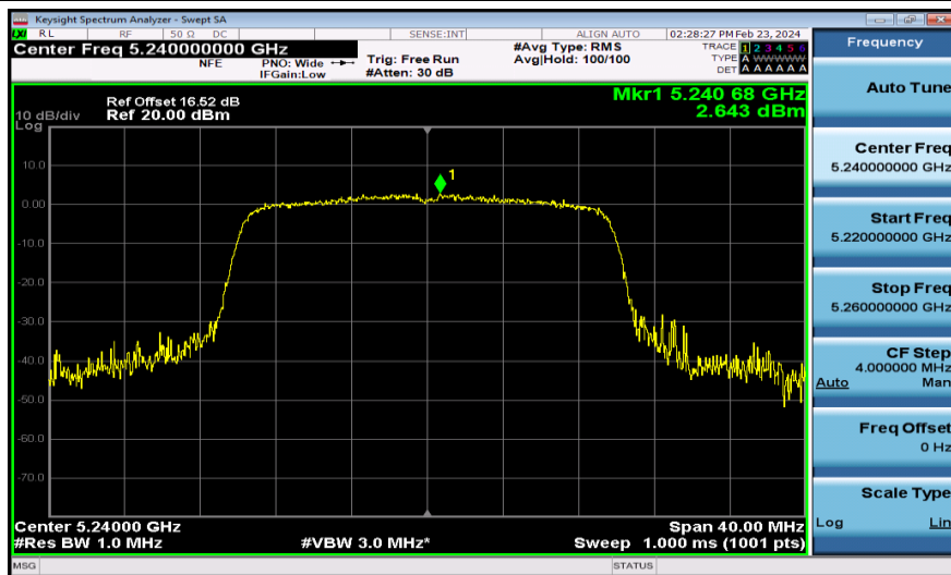
11AX20MIMO-Ant1-5240-PASS
