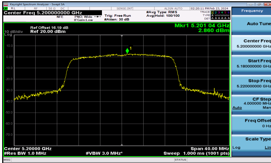
11AX20MIMO-Ant2-5200-PASS
