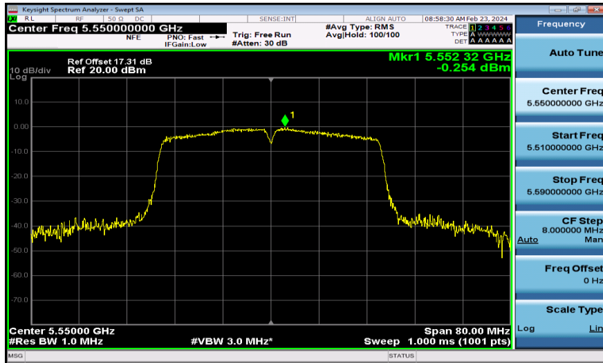
11AC40MIMO-Ant1-5550-PASS
