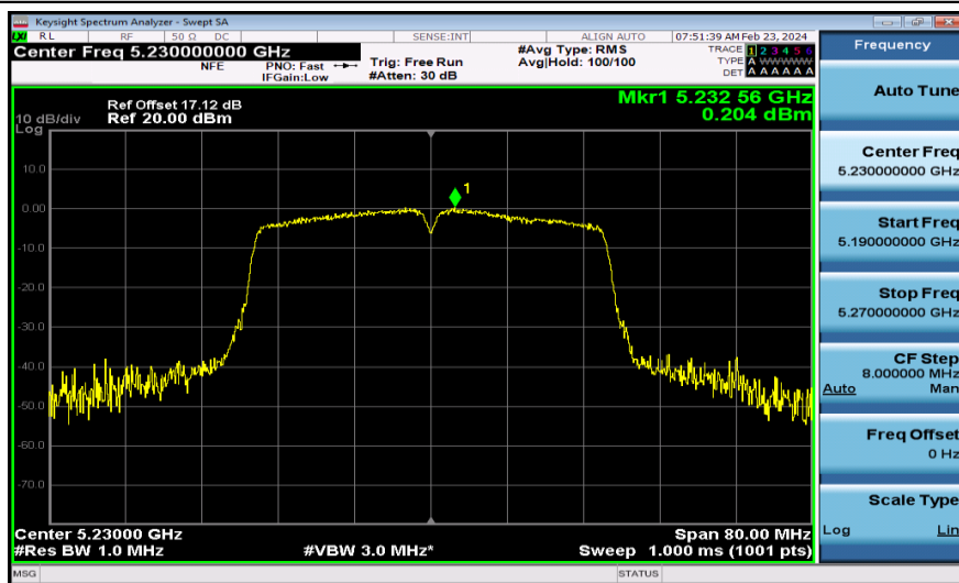
11AC40MIMO-Ant1-5230-PASS
