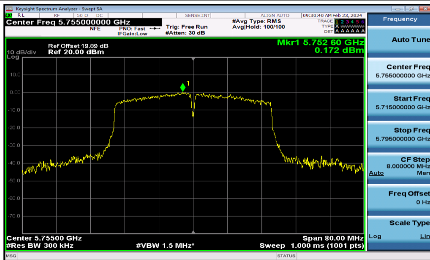
11AC40MIMO-Ant1-5755-PASS
