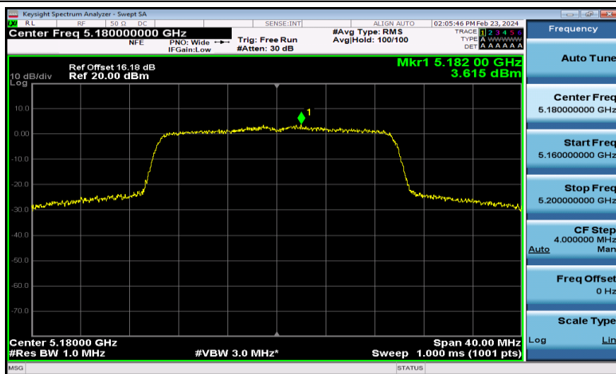
11AX20MIMO-Ant2-5180-PASS
