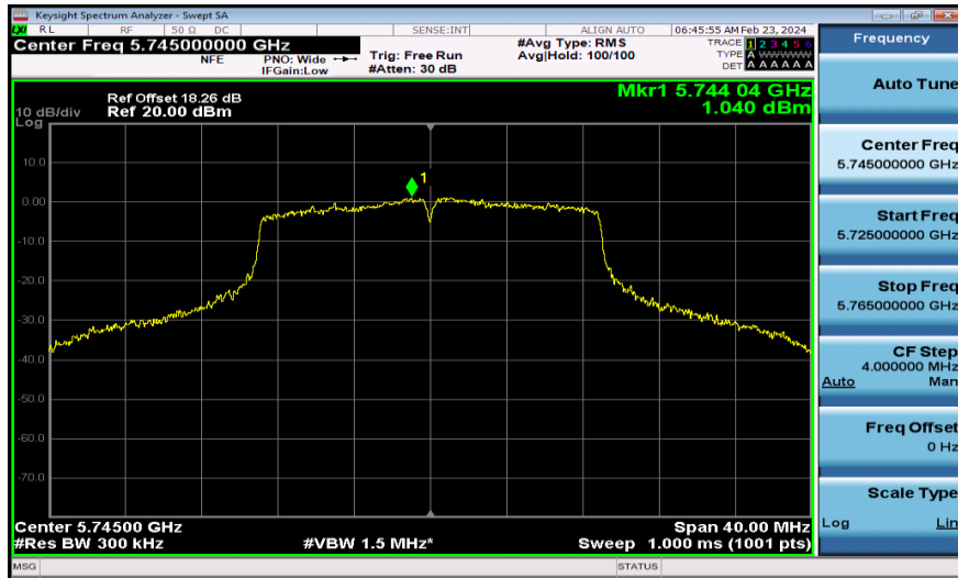
11AC20MIMO-Ant2-5745-PASS
