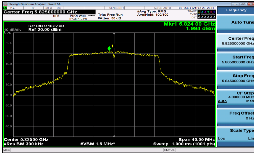
11AC20MIMO-Ant1-5825-PASS
