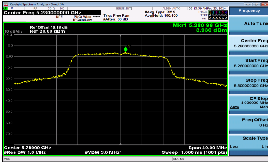
11AC20MIMO-Ant2-5280-PASS
