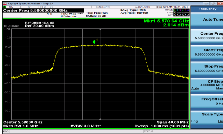
11AX20MIMO-Ant2-5580-PASS
