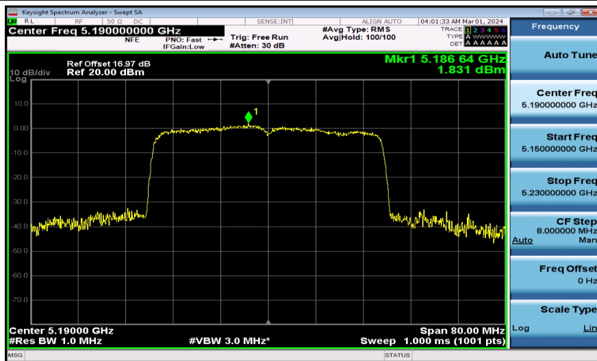
11AX40MIMO-Ant2-5190-PASS
