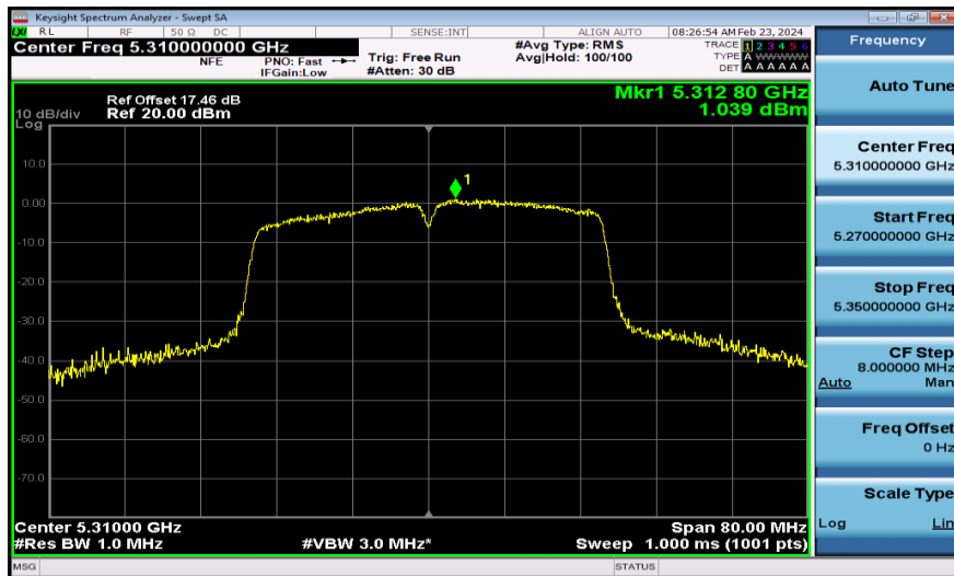
11AC40MIMO-Ant2-5310-PASS
