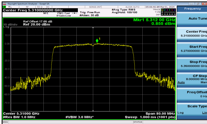
11AX40MIMO-Ant1-5310-PASS
