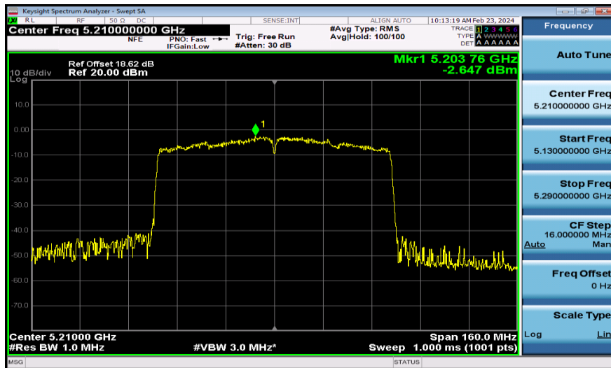
11AC80MIMO-Ant2-5210-PASS
