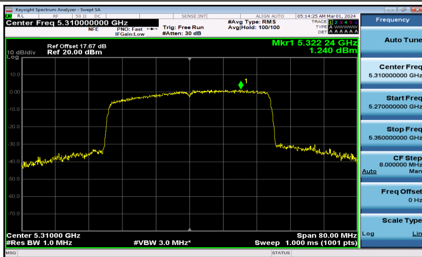
11AX40MIMO-Ant2-5310-PASS
