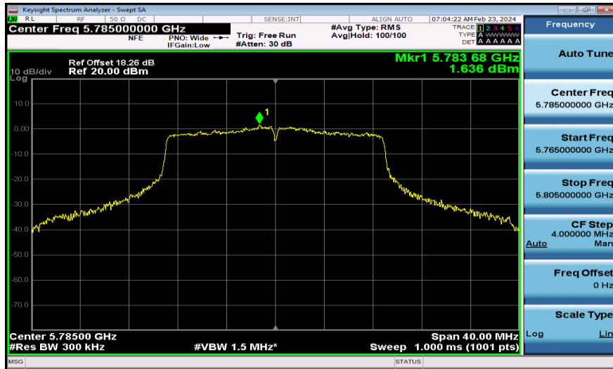
11AC20MIMO-Ant2-5785-PASS
