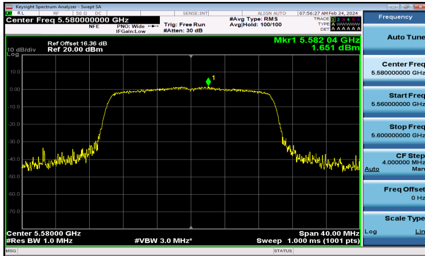
11AX20MIMO-Ant1-5580-PASS
