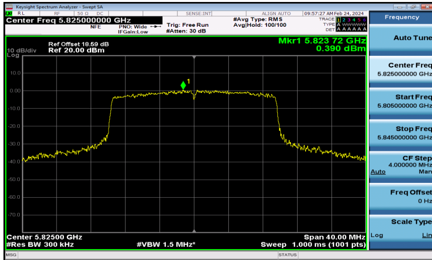
11AX20MIMO-Ant2-5825-PASS
