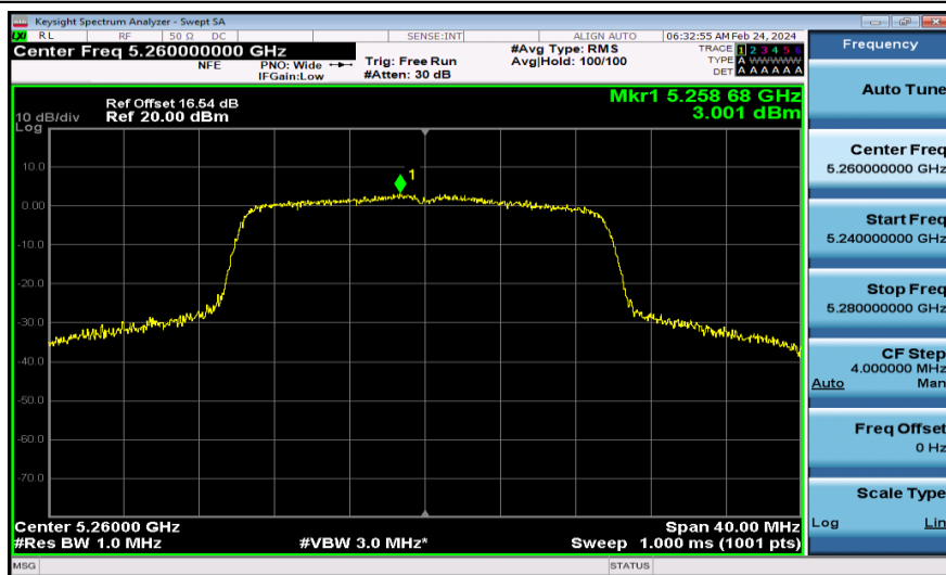
11AX20MIMO-Ant2-5260-PASS
