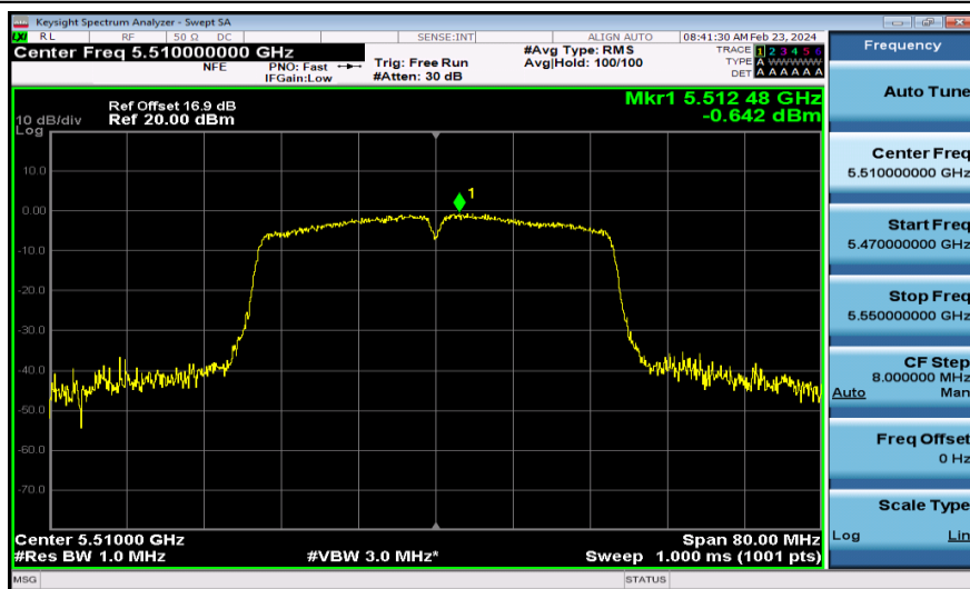
11AC40MIMO-Ant1-5510-PASS
