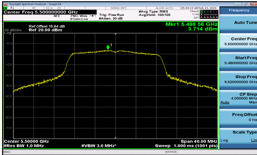
11AC20MIMO-Ant2-5500-PASS
