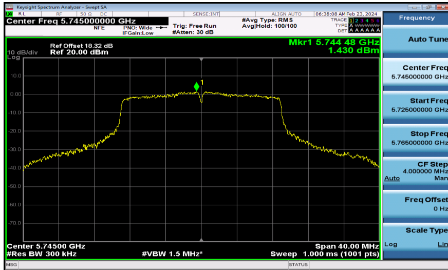
11AC20MIMO-Ant1-5745-PASS
