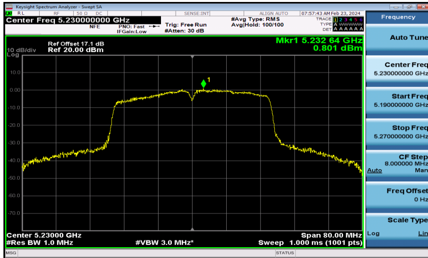
11AC40MIMO-Ant2-5230-PASS
