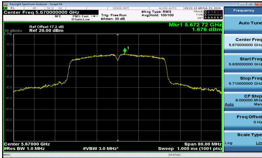
11AC40MIMO-Ant2-5670-PASS
