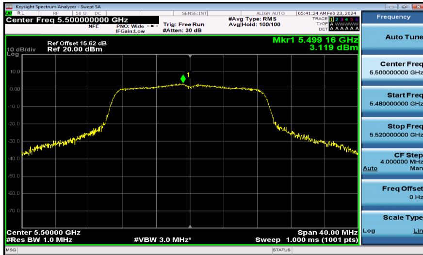
11AC20MIMO-Ant1-5500-PASS
