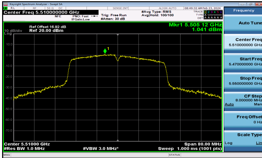
11AC40MIMO-Ant2-5510-PASS
