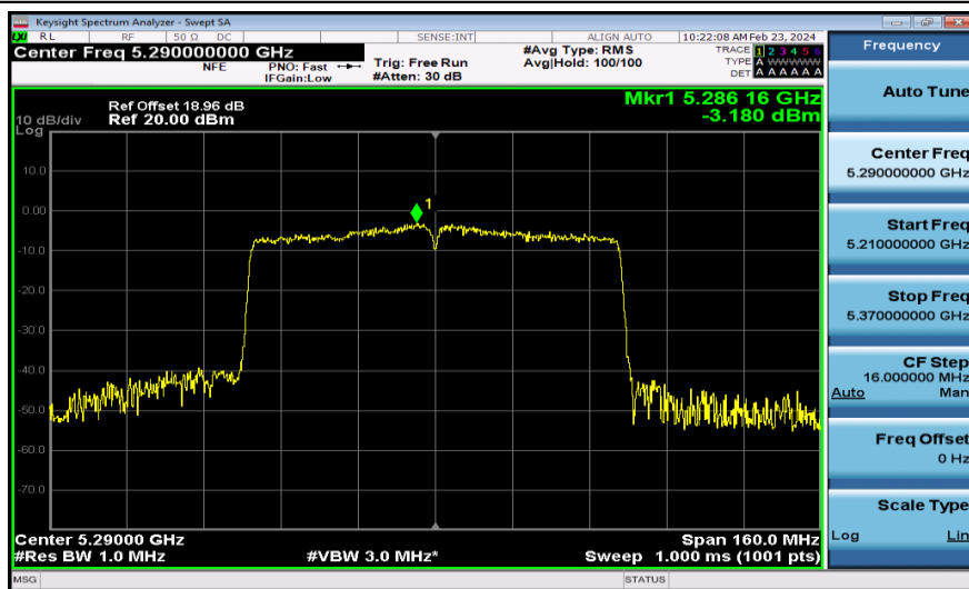
11AC80MIMO-Ant1-5290-PASS
