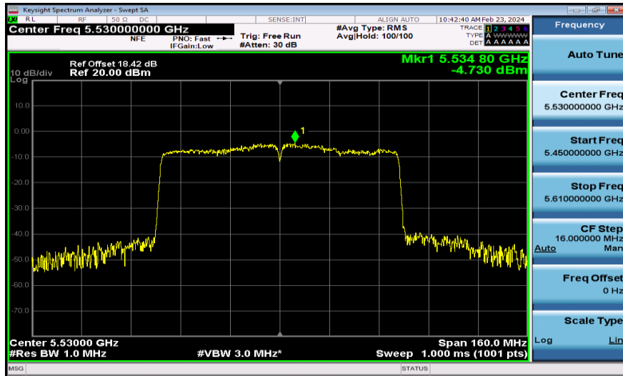
11AC80MIMO-Ant1-5530-PASS
