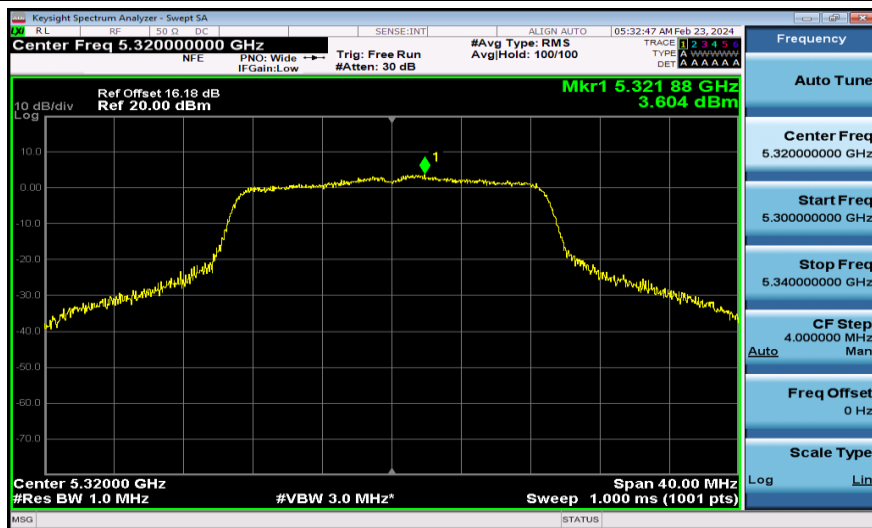
11AC20MIMO-Ant2-5320-PASS
