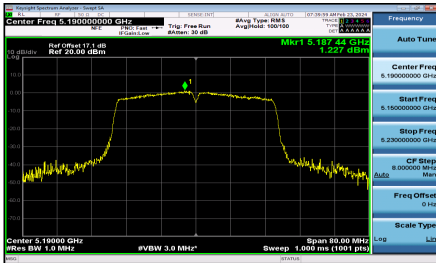
11AC40MIMO-Ant2-5190-PASS
