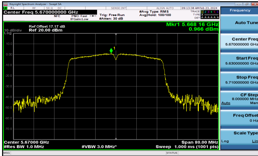
11AC40MIMO-Ant1-5670-PASS
