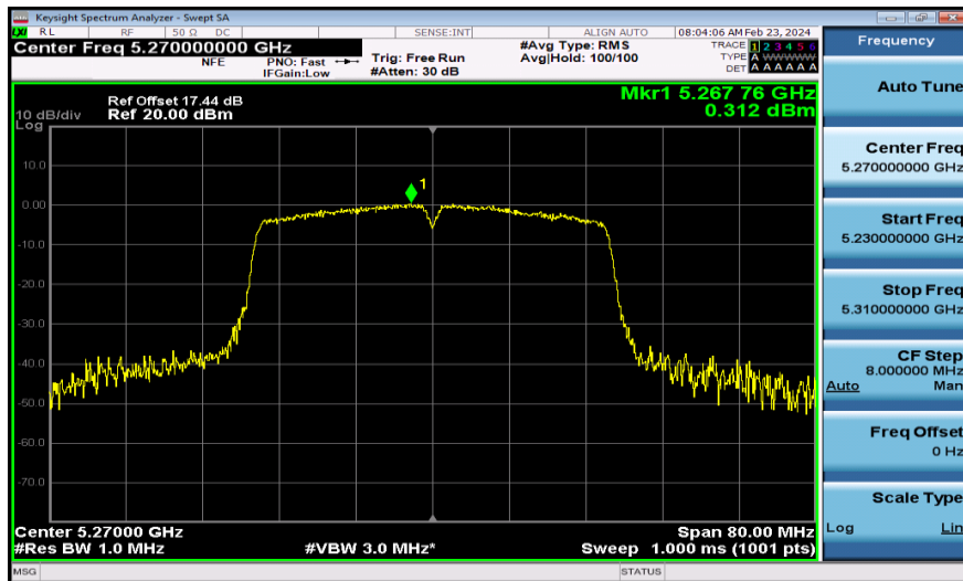
11AC40MIMO-Ant1-5270-PASS
