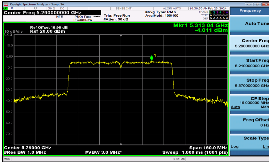
11AC80MIMO-Ant2-5290-PASS
