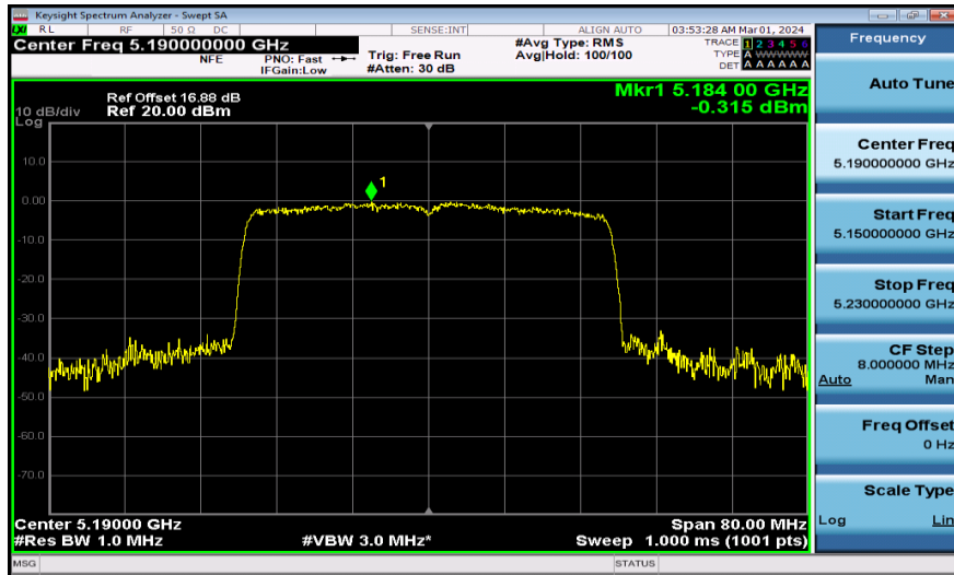
11AX40MIMO-Ant1-5190-PASS
