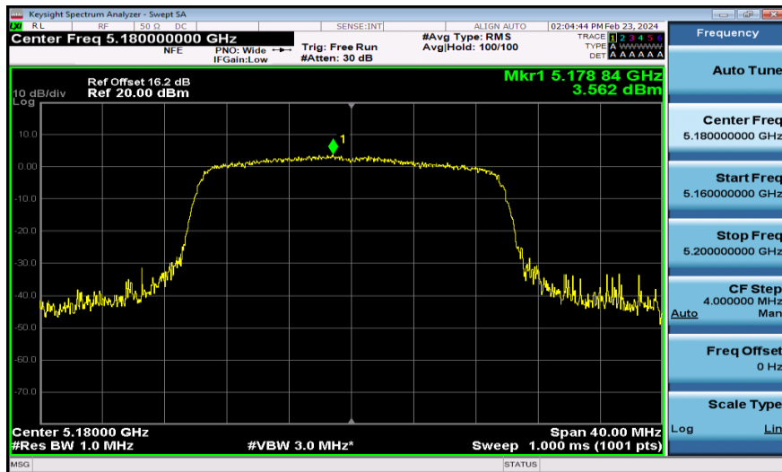
11AX20MIMO-Ant1-5180-PASS
