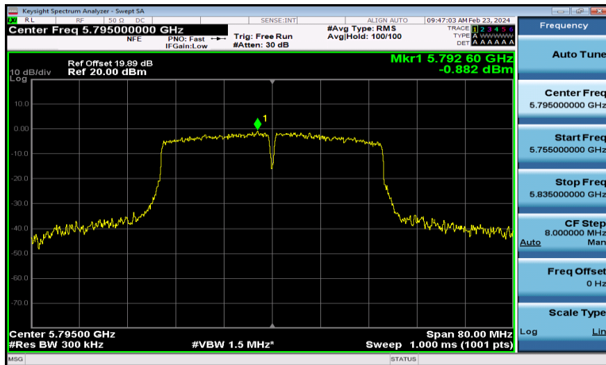
11AC40MIMO-Ant1-5795-PASS
