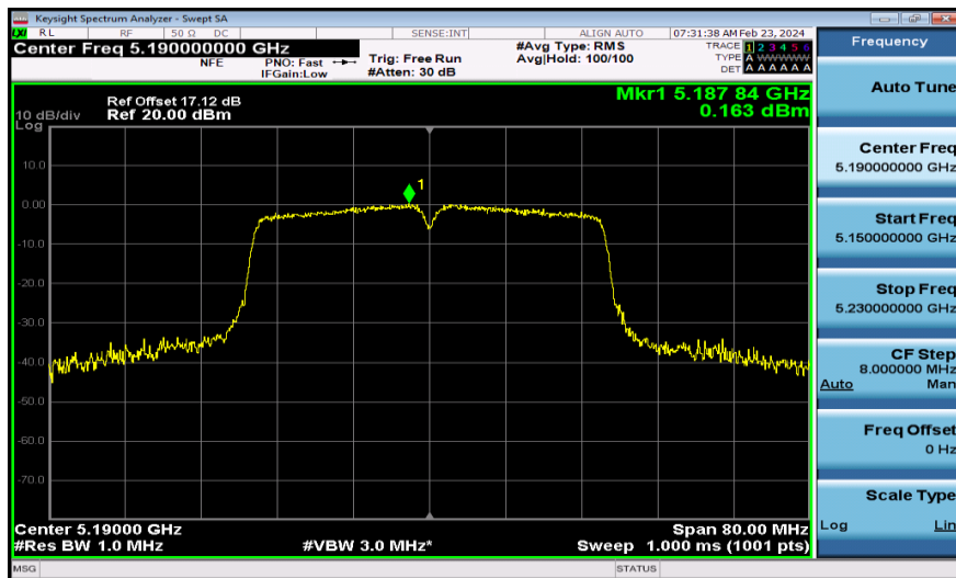
11AC40MIMO-Ant1-5190-PASS
