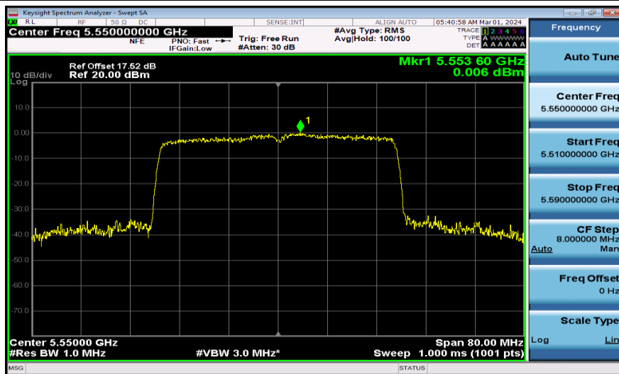
11AX40MIMO-Ant1-5550-PASS
