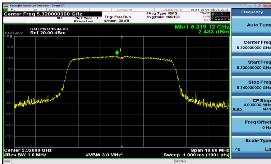
11AX20MIMO-Ant1-5320-PASS
