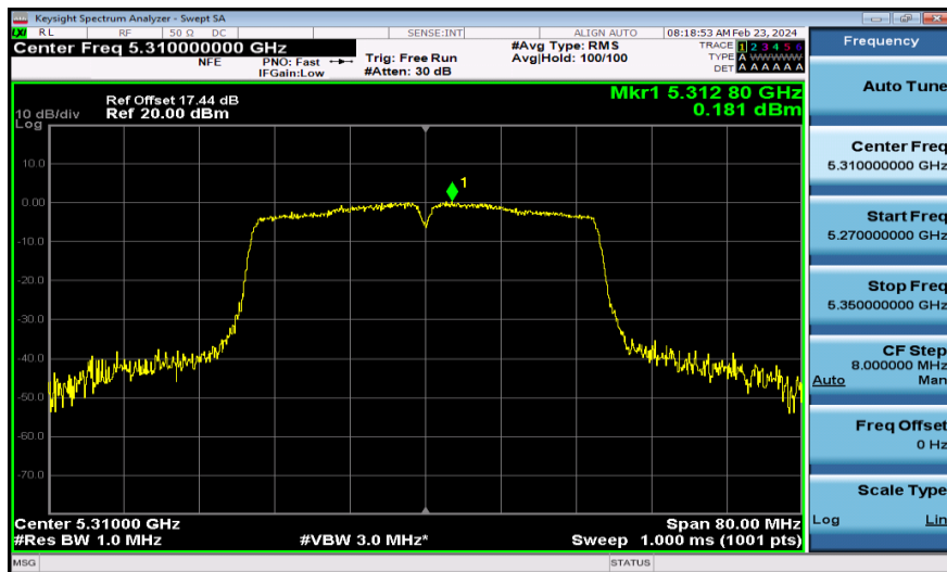
11AC40MIMO-Ant1-5310-PASS
