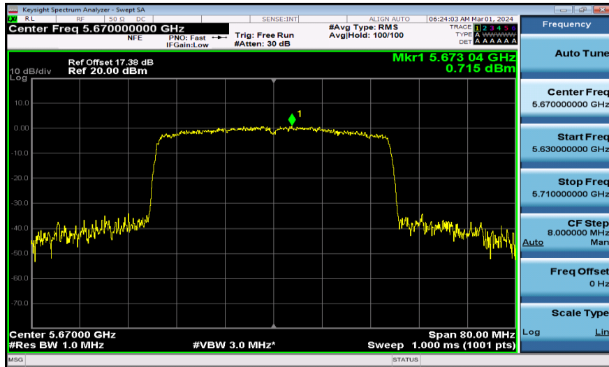
11AX40MIMO-Ant1-5670-PASS
