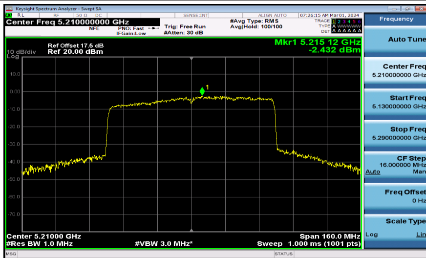
11AX80MIMO-Ant2-5210-PASS
