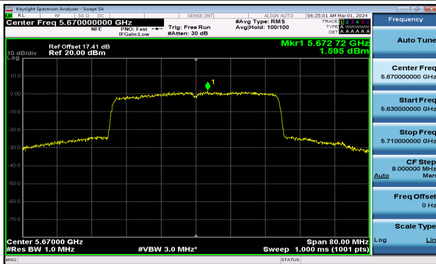
11AX40MIMO-Ant2-5670-PASS
