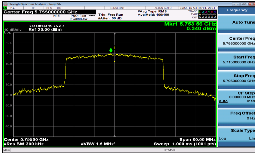
11AX40MIMO-Ant2-5755-PASS
