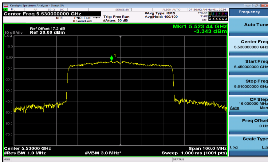
11AX80MIMO-Ant1-5530-PASS
