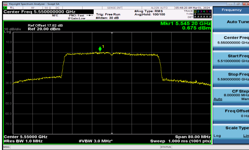
11AX40MIMO-Ant2-5550-PASS
