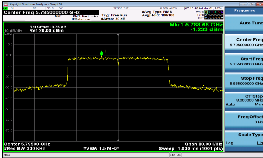
11AX40MIMO-Ant2-5795-PASS
