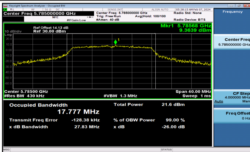
11A-Ant1-5785
