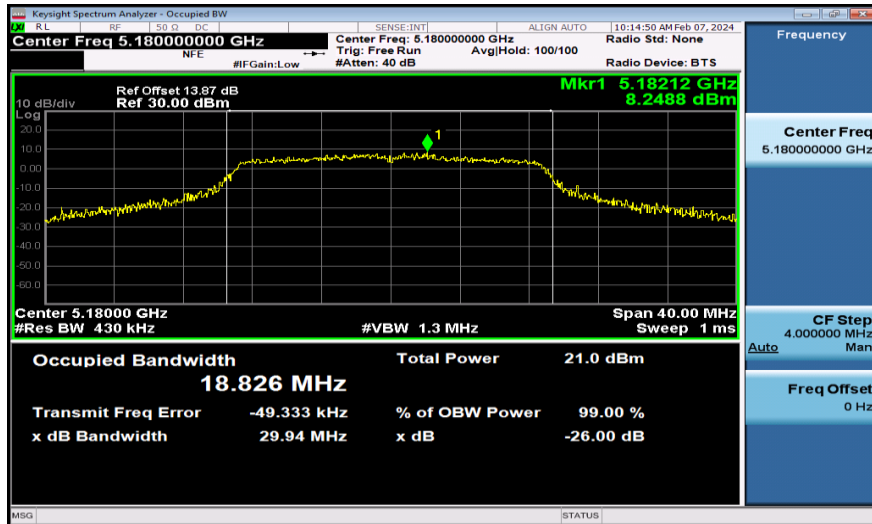
11N20MIMO-Ant1-5180
