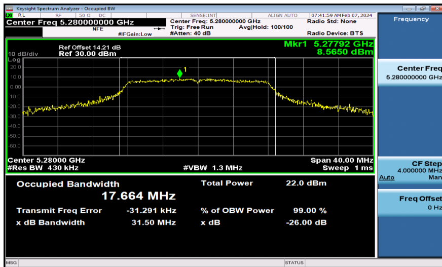
11A-Ant2-5280
