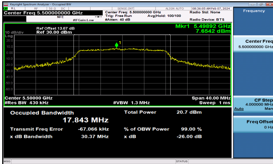
11A-Ant2-5500
