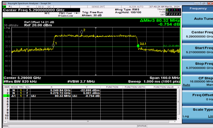
11AX80MIMO-Ant2-5290
