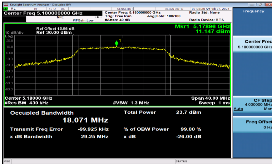
11A-Ant2-5180
