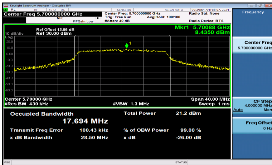
11A-Ant2-5700
