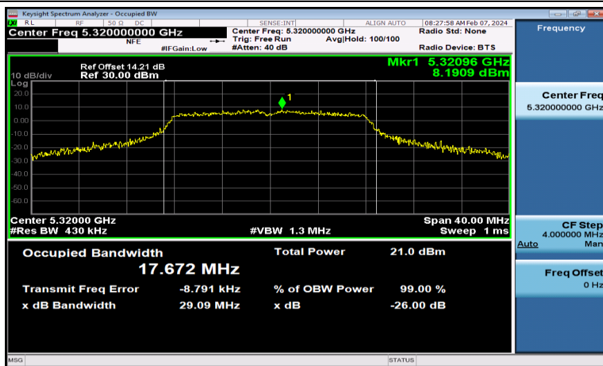
11A-Ant2-5320
