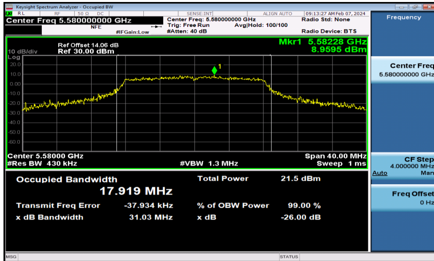
11A-Ant2-5580
