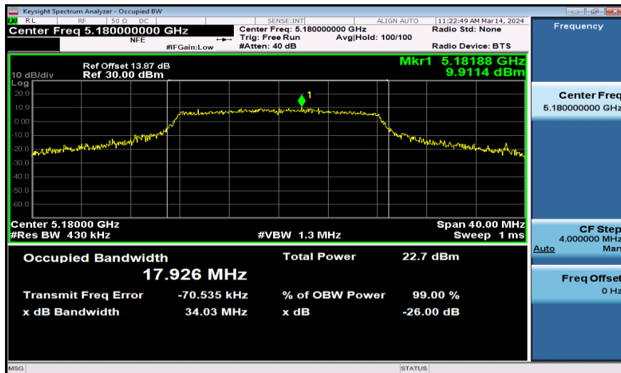
11A-Ant1-5180
