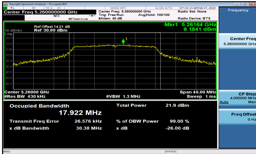
11A-Ant2-5260
