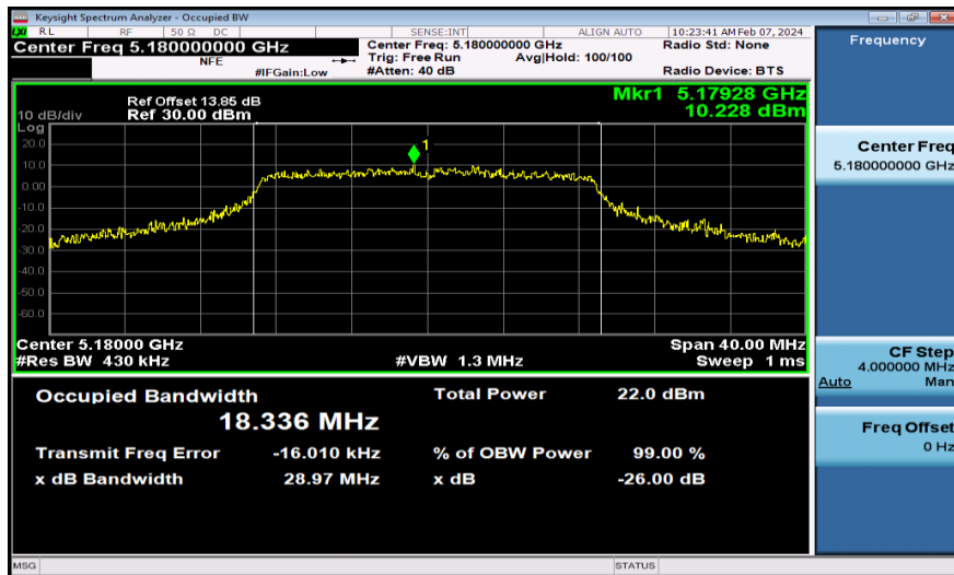
11N20MIMO-Ant2-5180
