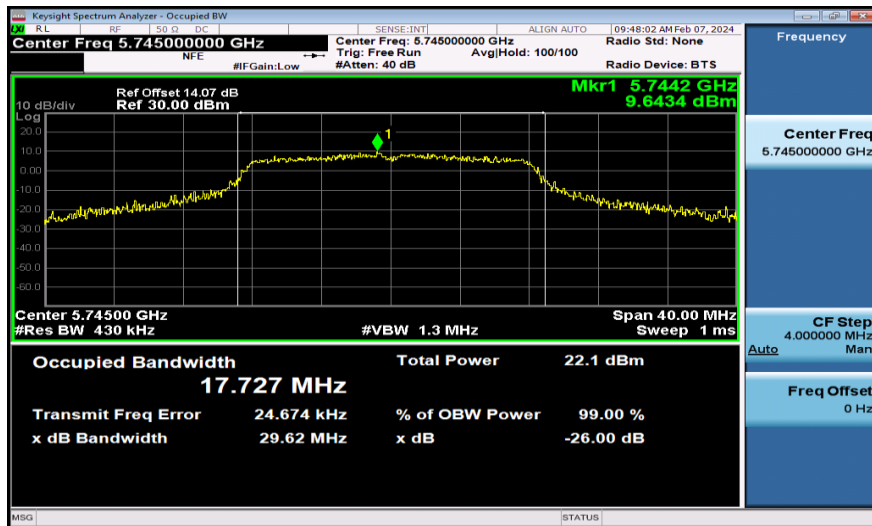
11A-Ant2-5745
