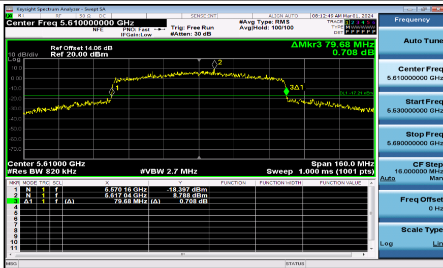
11AX80MIMO-Ant2-5610
