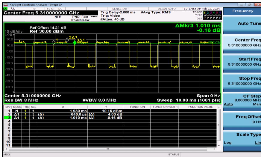
NTNV-11N40MIMO-Ant2-5310
