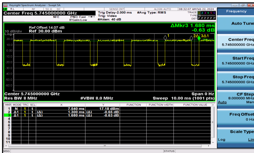
NTNV-11N20MIMO-Ant2-5745
