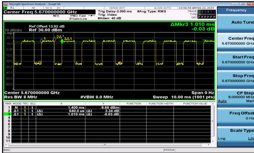
NTNV-11N40MIMO-Ant1-5670
