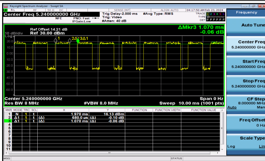
NTNV-11AC20MIMO-Ant2-5240
