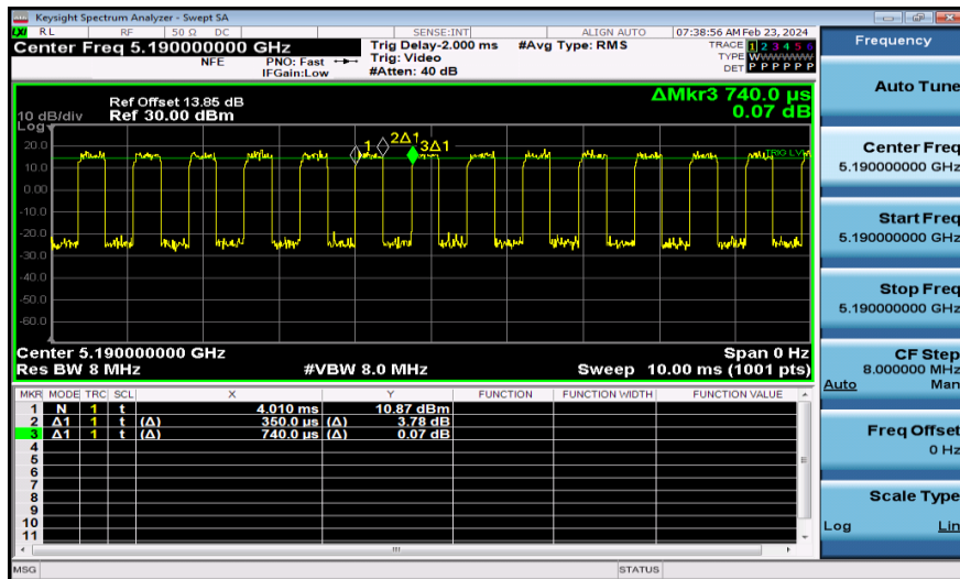
NTNV-11AC40MIMO-Ant2-5190
