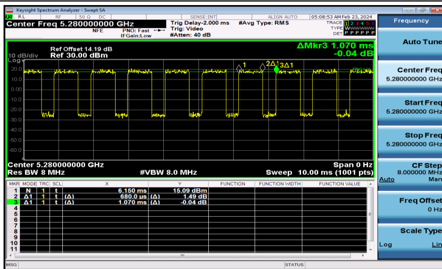
NTNV-11AC20MIMO-Ant1-5280
