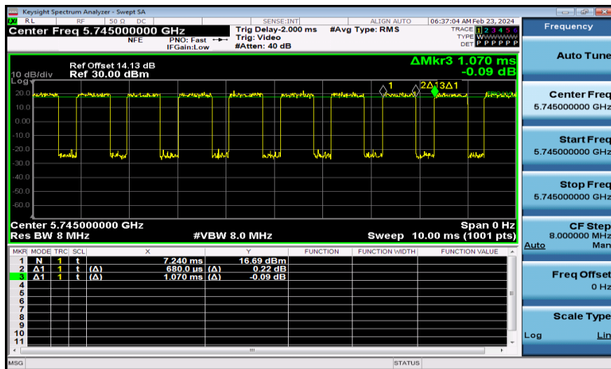
NTNV-11AC20MIMO-Ant1-5745
