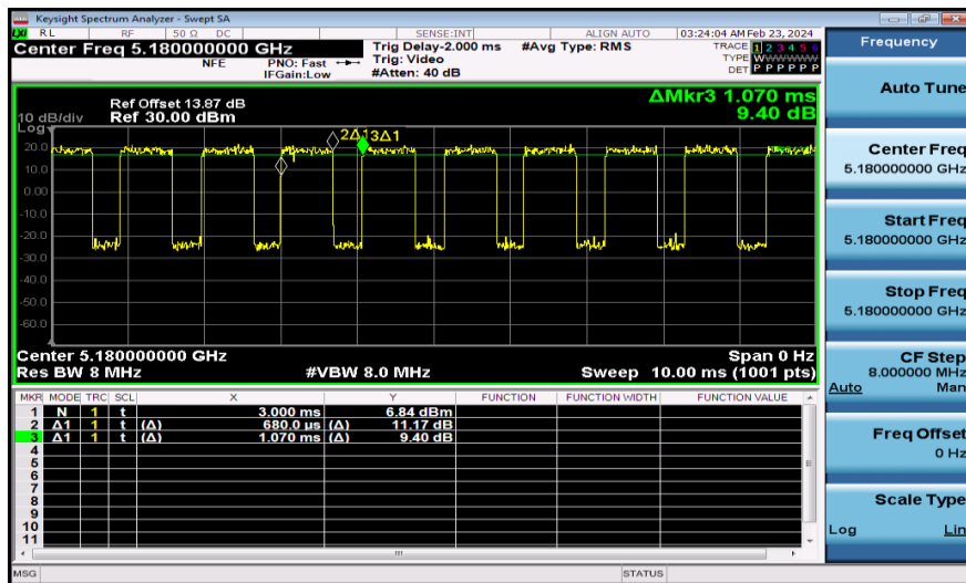
NTNV-11AC20MIMO-Ant1-5180
