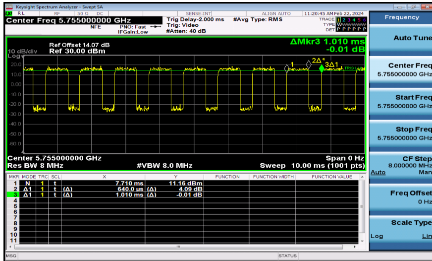
NTNV-11N40MIMO-Ant2-5755
