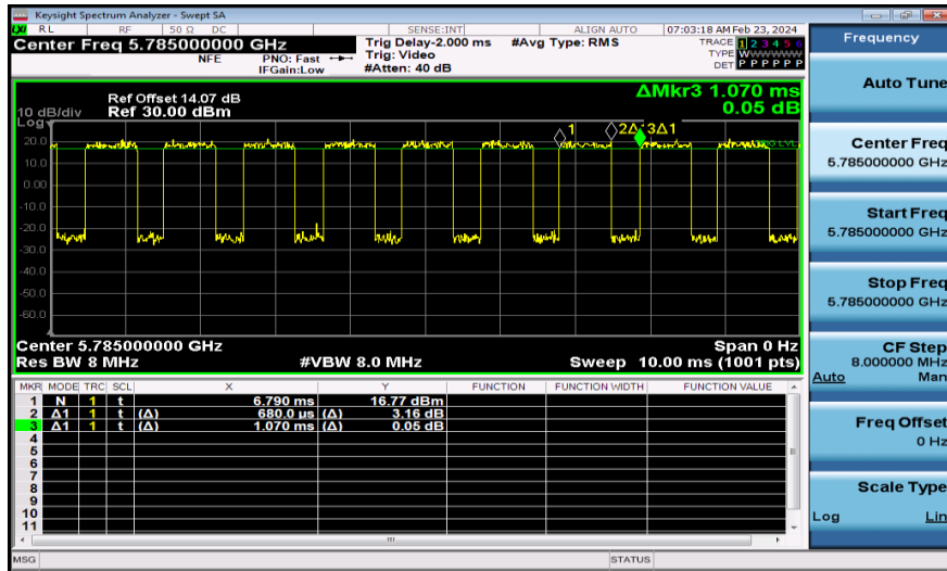
NTNV-11AC20MIMO-Ant2-5785
