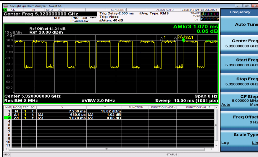
NTNV-11AC20MIMO-Ant2-5320
