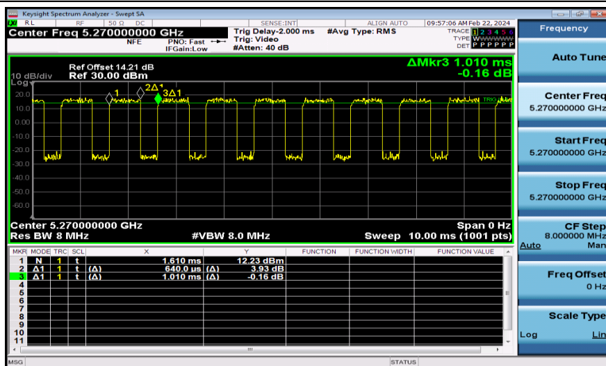
NTNV-11N40MIMO-Ant2-5270
