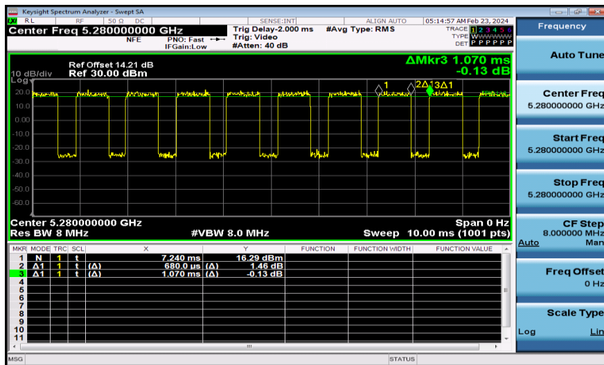
NTNV-11AC20MIMO-Ant2-5280
