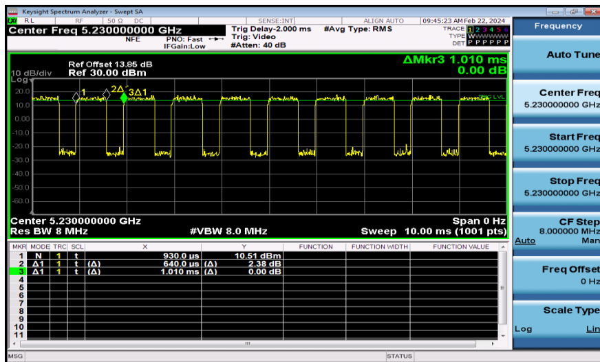
NTNV-11N40MIMO-Ant2-5230
