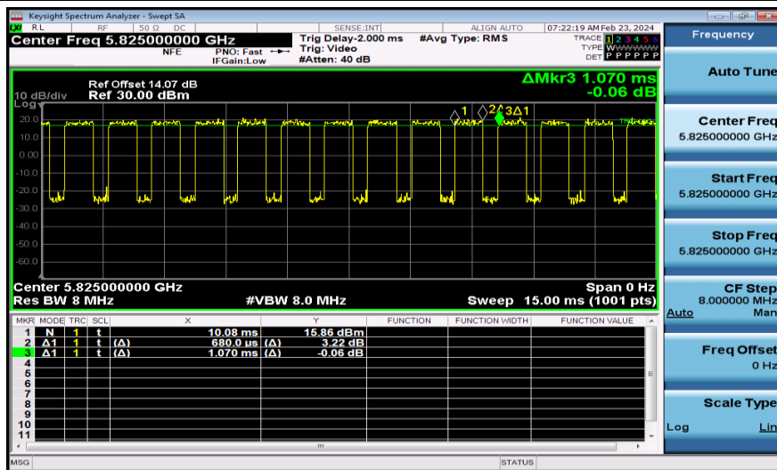
NTNV-11AC20MIMO-Ant2-5825
