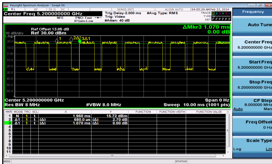
NTNV-11AC20MIMO-Ant2-5200
