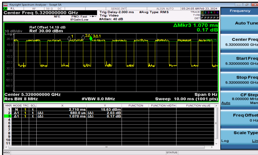
NTNV-11AC20MIMO-Ant1-5320
