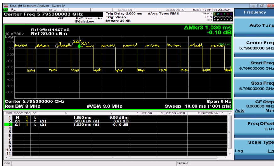
NTNV-11N40MIMO-Ant2-5795
