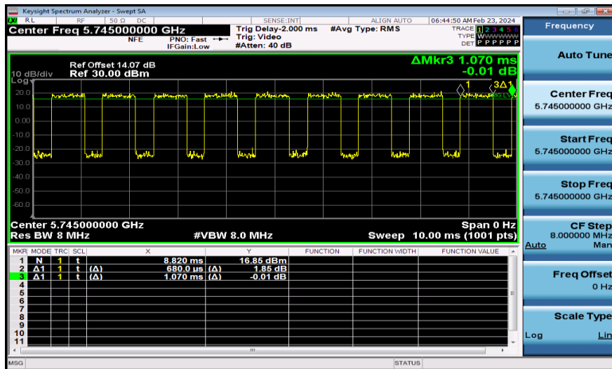
NTNV-11AC20MIMO-Ant2-5745
