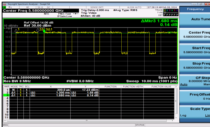
NTNV-11N20MIMO-Ant2-5580
