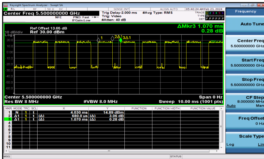
NTNV-11AC20MIMO-Ant1-5500
