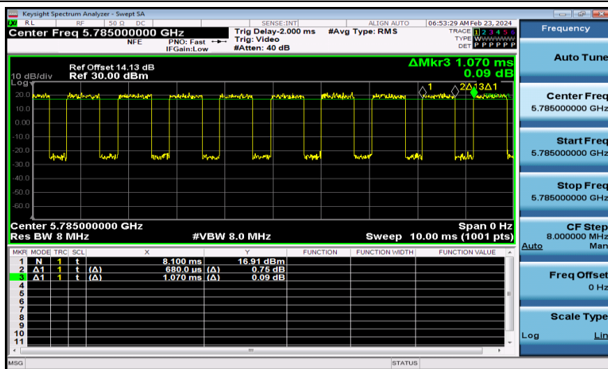
NTNV-11AC20MIMO-Ant1-5785
