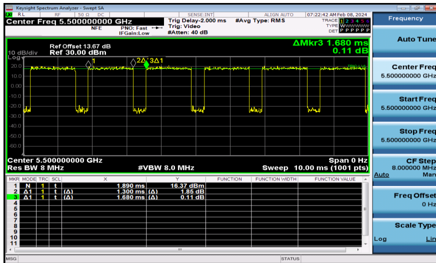
NTNV-11N20MIMO-Ant2-5500
