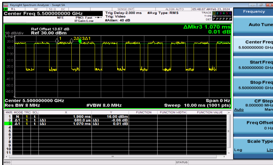
NTNV-11AC20MIMO-Ant2-5500
