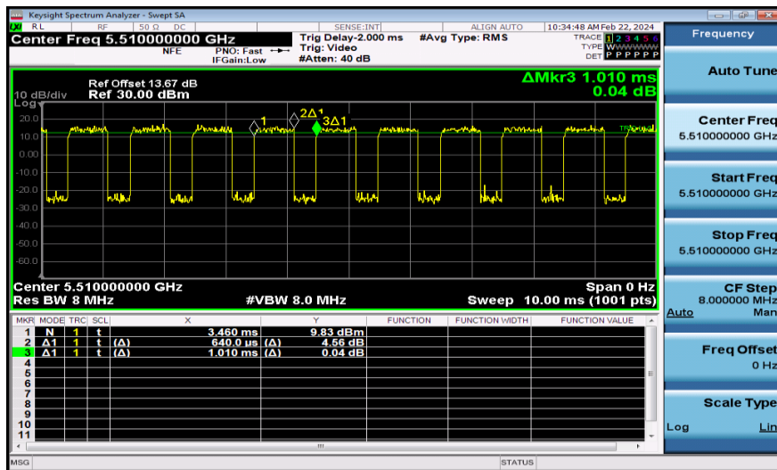
NTNV-11N40MIMO-Ant2-5510
