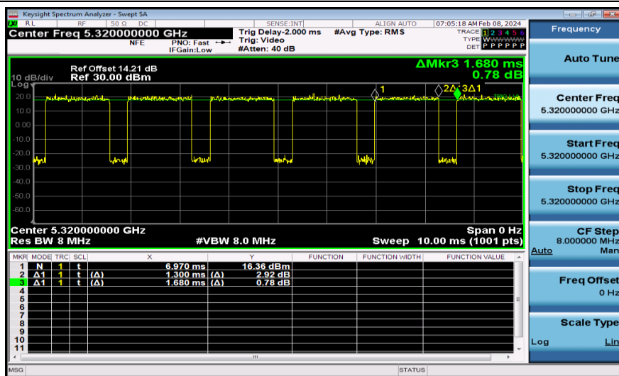
NTNV-11N20MIMO-Ant2-5320
