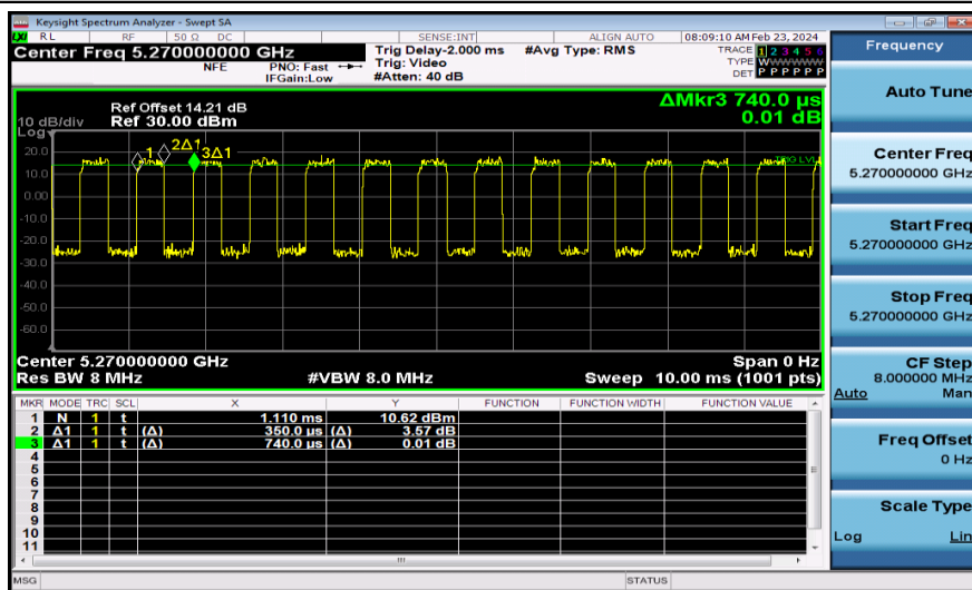
NTNV-11AC40MIMO-Ant2-5270
