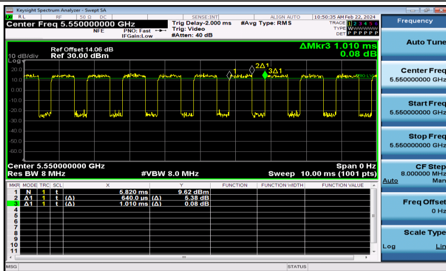
NTNV-11N40MIMO-Ant2-5550
