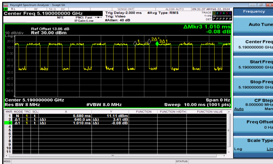
NTNV-11N40MIMO-Ant2-5190
