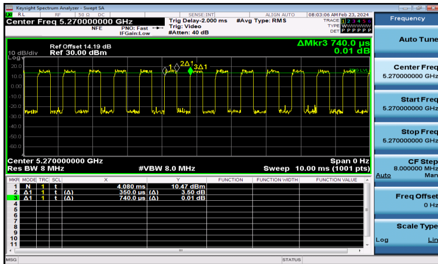
NTNV-11AC40MIMO-Ant1-5270
