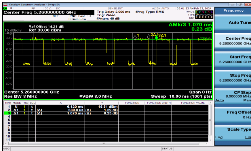
NTNV-11AC20MIMO-Ant2-5260
