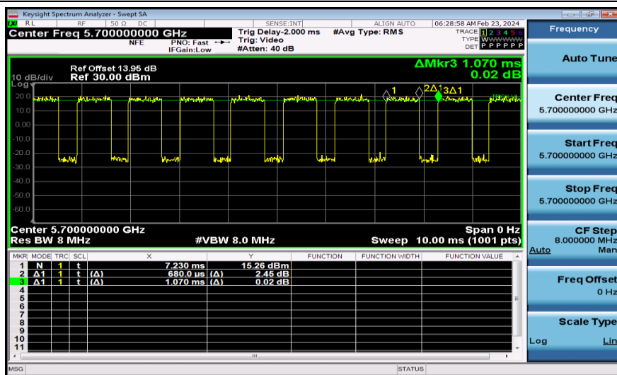
NTNV-11AC20MIMO-Ant2-5700
