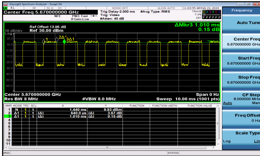
NTNV-11N40MIMO-Ant2-5670
