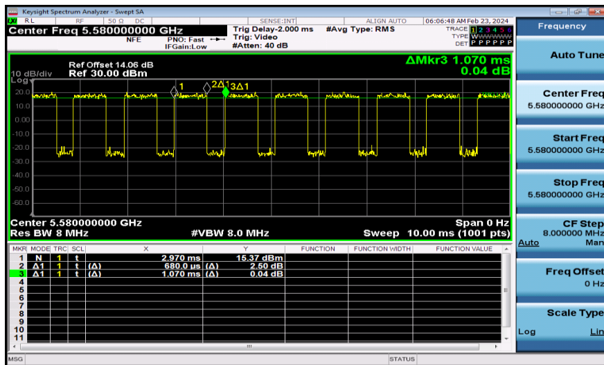
NTNV-11AC20MIMO-Ant2-5580
