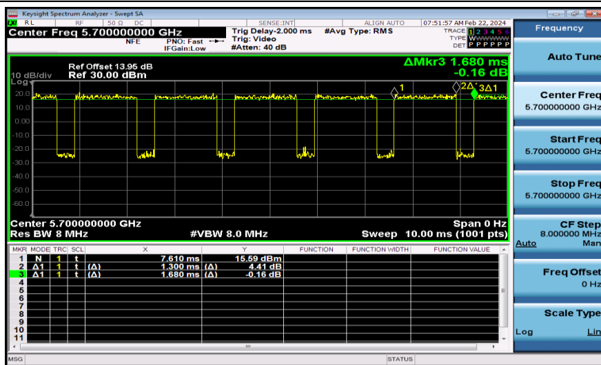
NTNV-11N20MIMO-Ant2-5700
