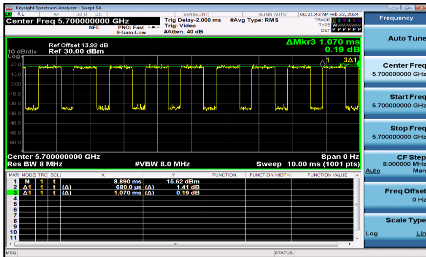
NTNV-11AC20MIMO-Ant1-5700
