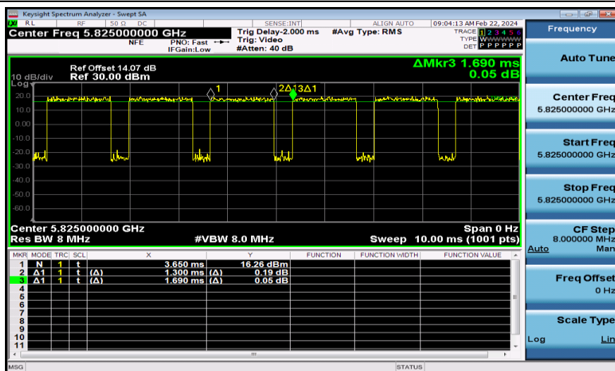
NTNV-11N20MIMO-Ant2-5825
