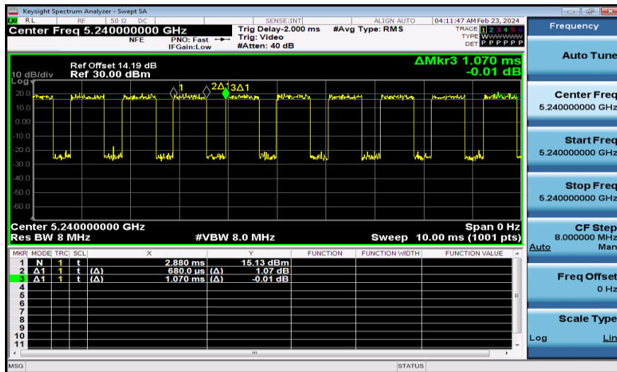
NTNV-11AC20MIMO-Ant1-5240
