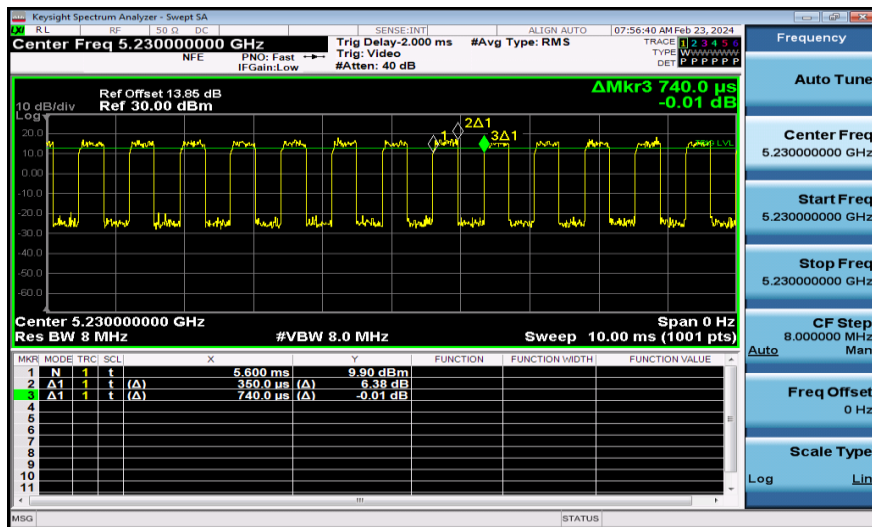
NTNV-11AC40MIMO-Ant2-5230
