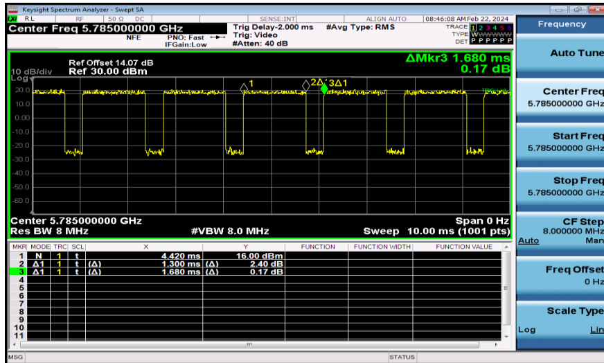
NTNV-11N20MIMO-Ant2-5785
