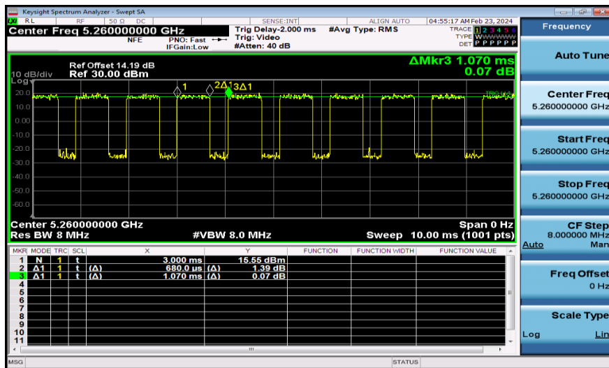
NTNV-11AC20MIMO-Ant1-5260
