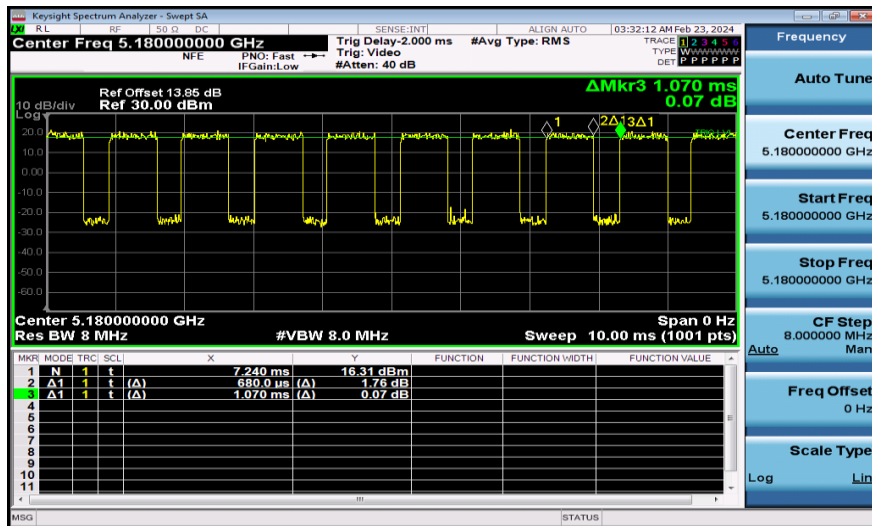
NTNV-11AC20MIMO-Ant2-5180
