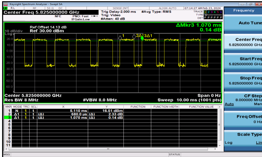
NTNV-11AC20MIMO-Ant1-5825
