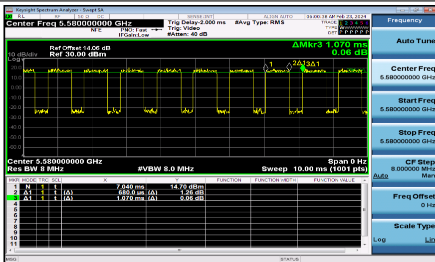
NTNV-11AC20MIMO-Ant1-5580
