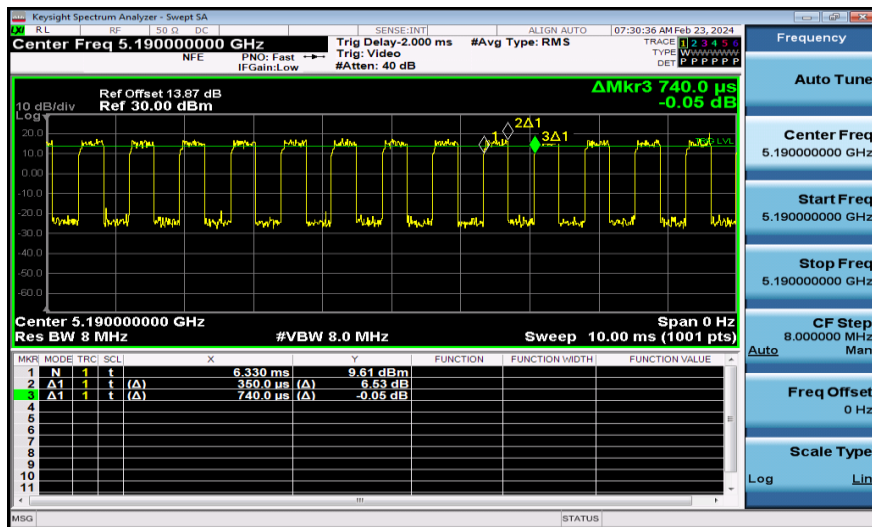
NTNV-11AC40MIMO-Ant1-5190
