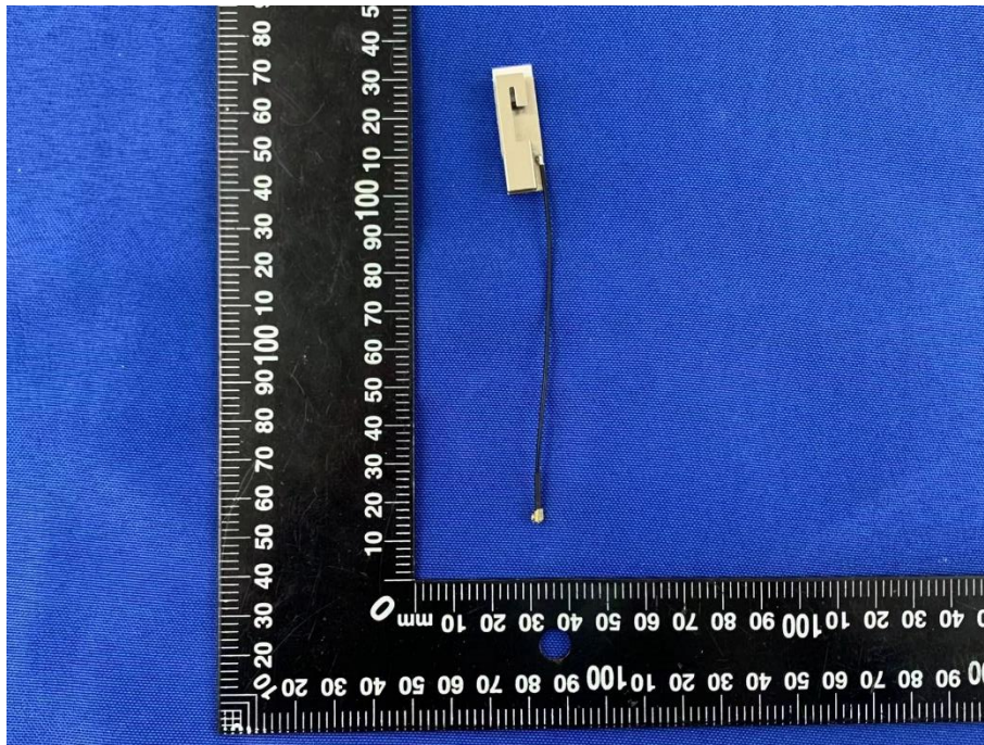
PIFA ANTENNA-85mm
