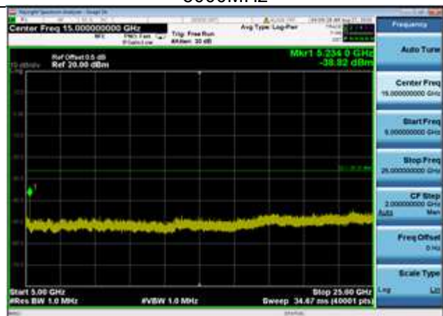
802.11g,2462MHz,Ant1,Plot 5,5000MHz~25000MHz
