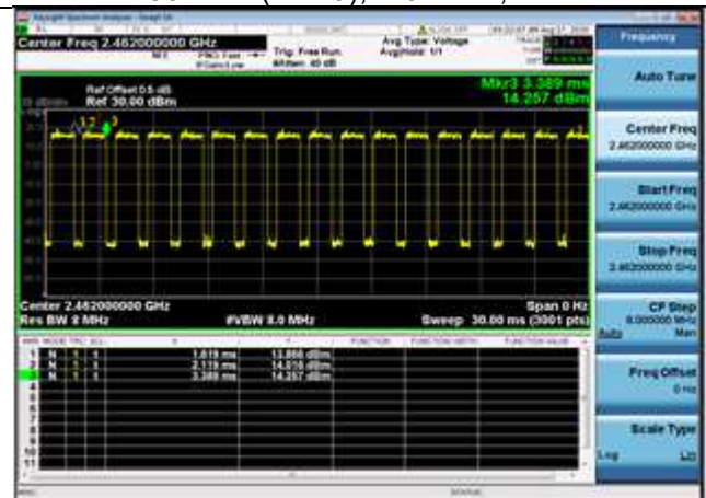
802.11n(HT20),2462MHz,Ant1
