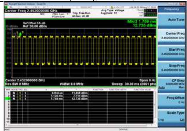
802.11n(HT40),2452MHz,Ant1
