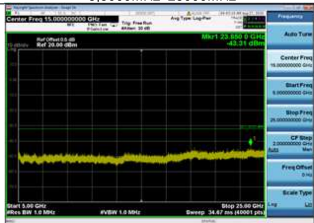
802.11n(HT40),2452MHz,Ant1,Plot 5,5000MHz~25000MHz
