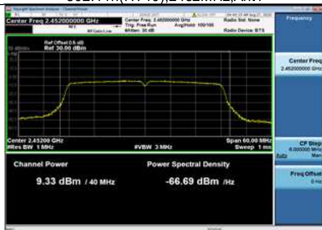
802.11n(HT40),2452MHz,Ant1
