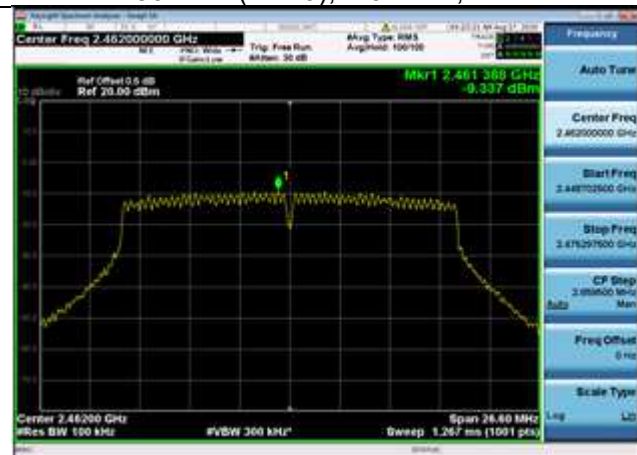
802.11n(HT20),2462MHz,Ant1
