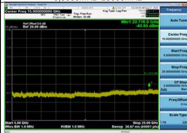
802.11n(HT40),2422MHz,Ant0,Plot 5,5000MHz~25000MHz
