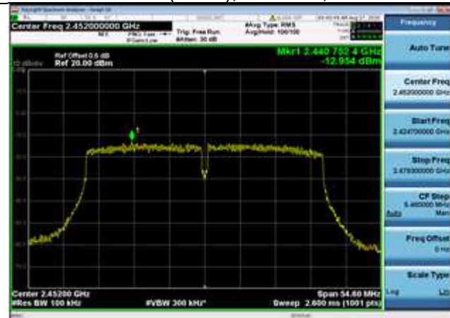
802.11n(HT40),2452MHz,Ant1
