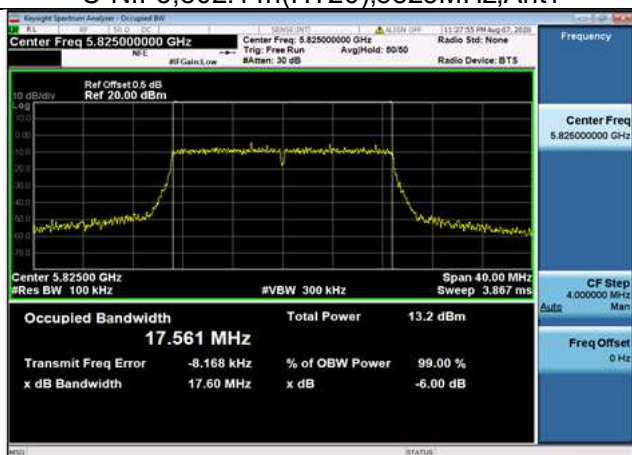
U-NII-3,802.11n(HT20),5825MHz,Ant1
