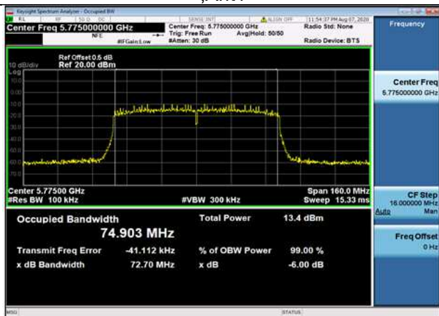
U-NII-3,802.11ac(VHT80),5775MHz Ant1
