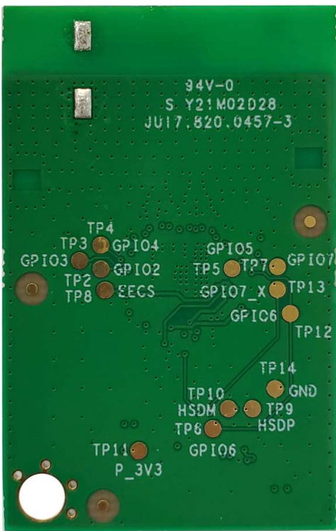
BOTTOM VIEW
