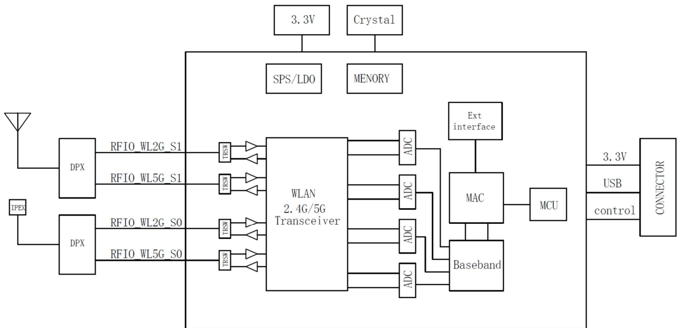
Figure 1 WF-R12C-UWD2L Block Diagram
