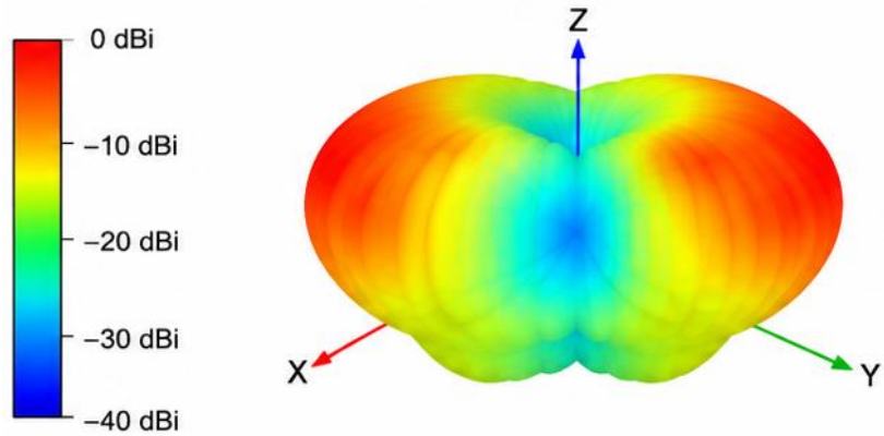
3D Radiation Pattern
