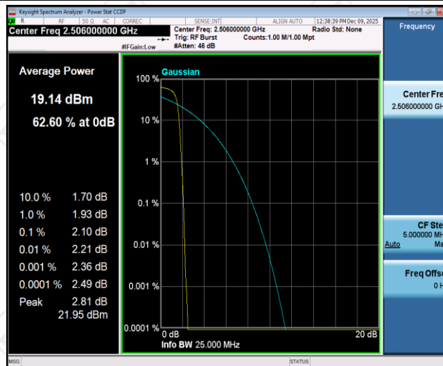
Band41-20MHz-16QAM-39750-1RB#0
