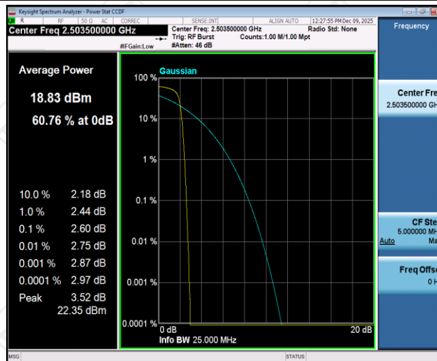
Band41-15MHz-QPSK-39725-1RB#0
