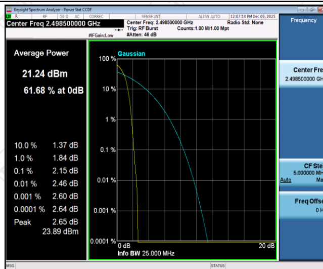
Band41-5MHz-QPSK-39675-25RB#0
