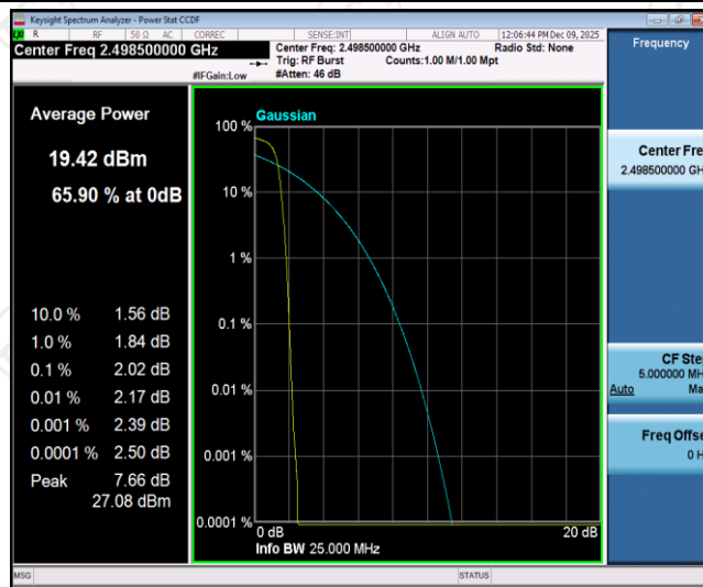
Band41-5MHz-QPSK-39675-1RB#0
