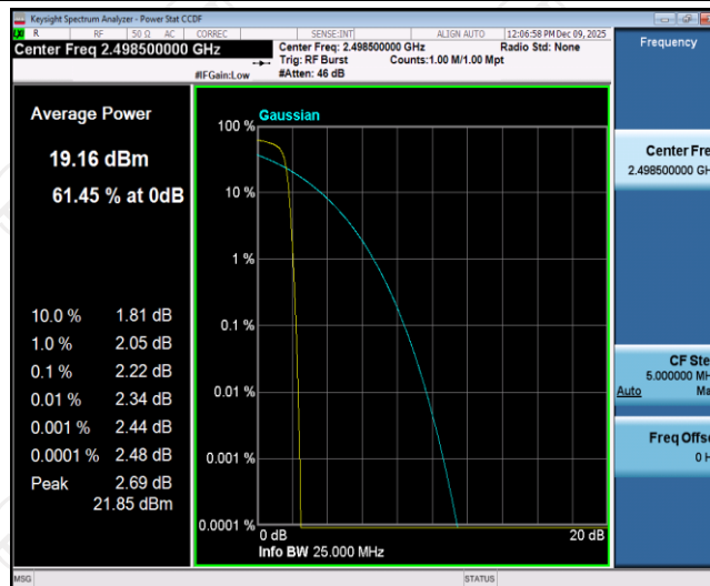
Band41-5MHz-16QAM-39675-1RB#0
