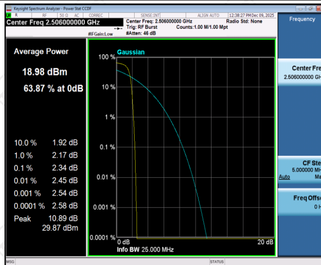
Band41-20MHz-QPSK-39750-1RB#0
