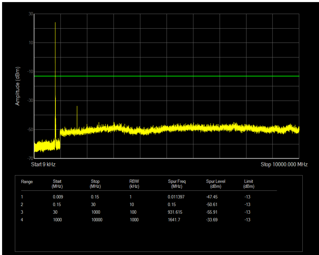
Band18 QAM16 BW=10MHz Channel=23950 RB Size=50 Position=#0
