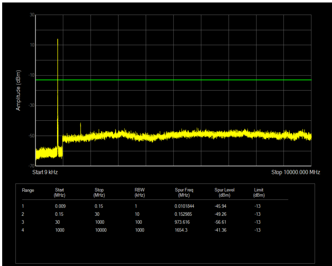
Band18 QAM16 BW=5MHz Channel=23975 RB Size=25 Position=#0
