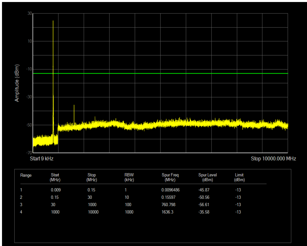
Band18 QAM16 BW=10MHz Channel=23925 RB Size=50 Position=#0
