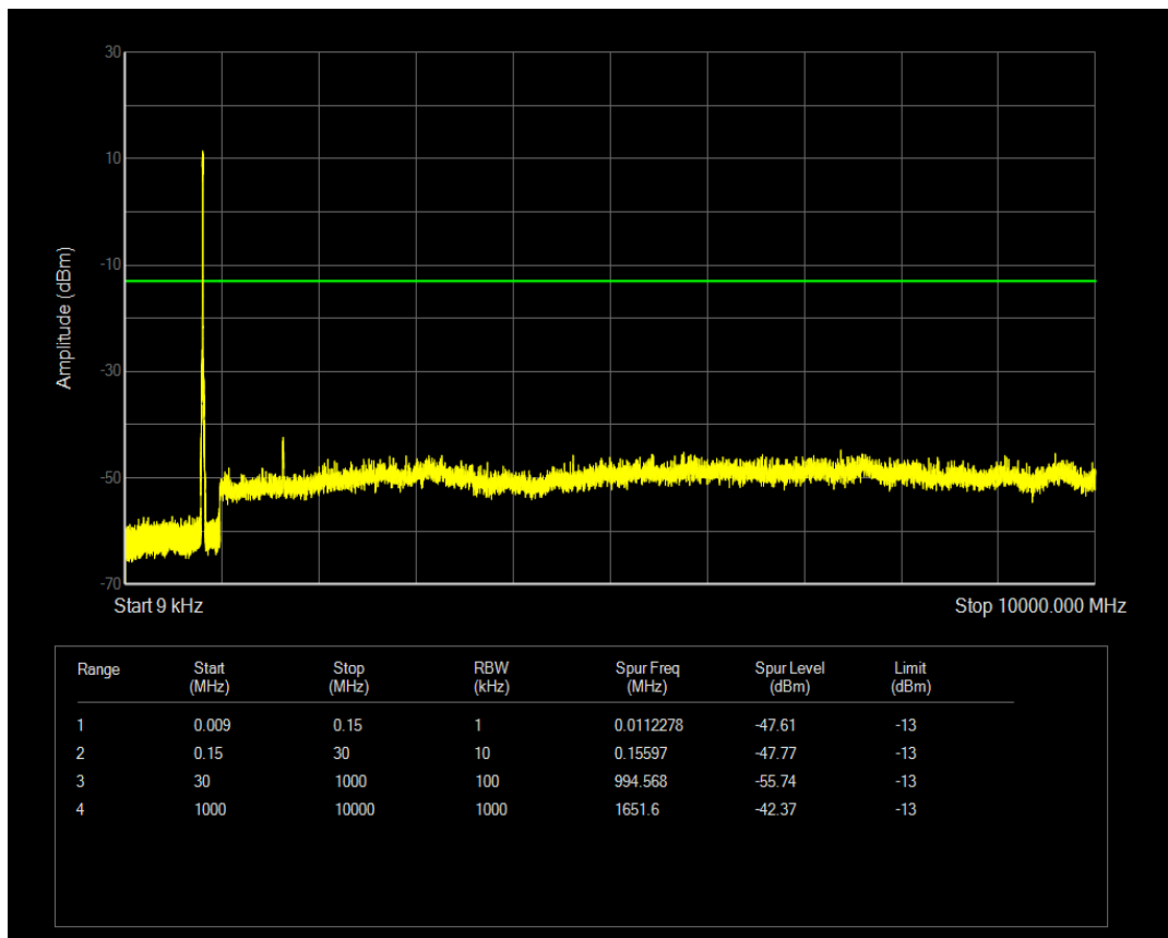
Band18 QAM16 BW=10MHz Channel=23950 RB Size=50 Position=#0
