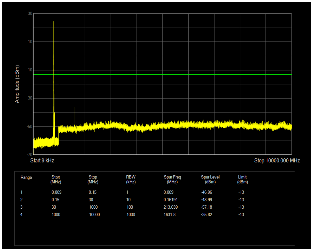
Band18 QAM16 BW=15MHz Channel=23925 RB Size=75 Position=#0
