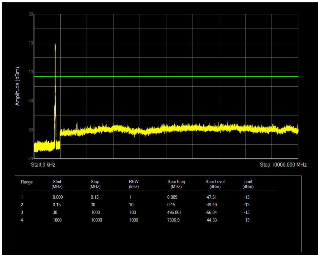
Band18 QAM16 BW=15MHz Channel=23925 RB Size=75 Position=#0
