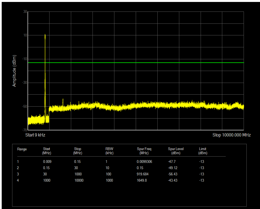
Band18 QAM16 BW=10MHz Channel=23925 RB Size=50 Position=#0
