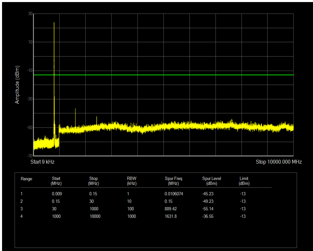
Band18 QAM16 BW=10MHz Channel=23900 RB Size=50 Position=#0
