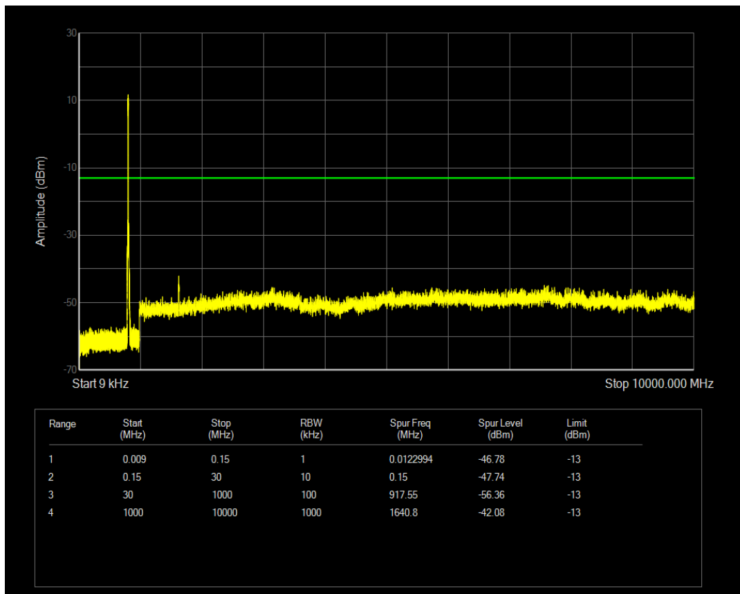
Band18 QAM16 BW=10MHz Channel=23900 RB Size=50 Position=#0
