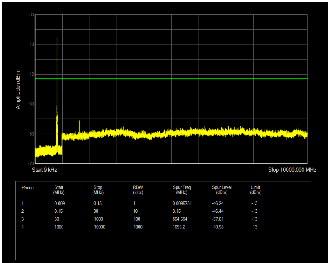
Band18 QPSK BW=5MHz Channel=23975 RB Size=25 Position=#0
