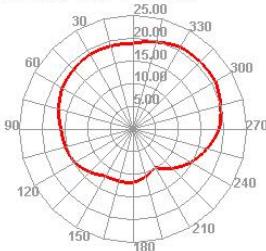
Wifi 60 TRP Phi=45
