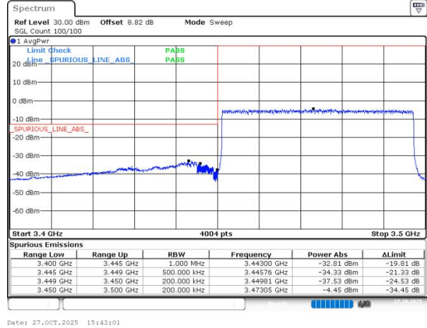
n78(3450-3550) SCS=30kHz DFT_QPSK BW=50MHz LowChannel=631668 RB=128@0
