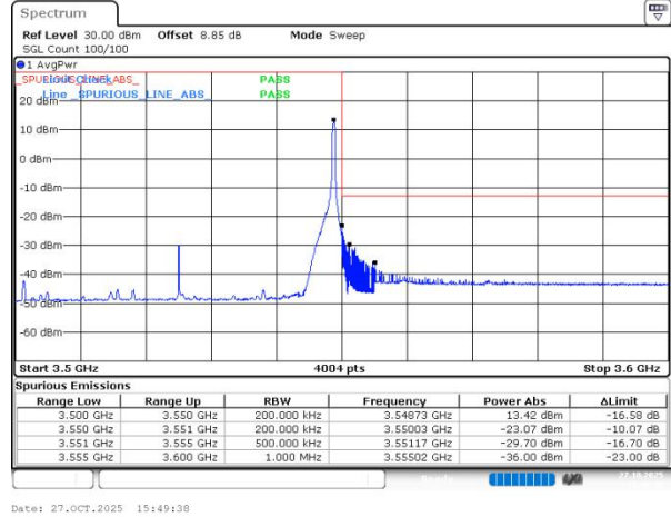
n78(3450-3550) SCS=30kHz DFT_16QAM BW=50MHz HighChannel=635000 RB=1@132
