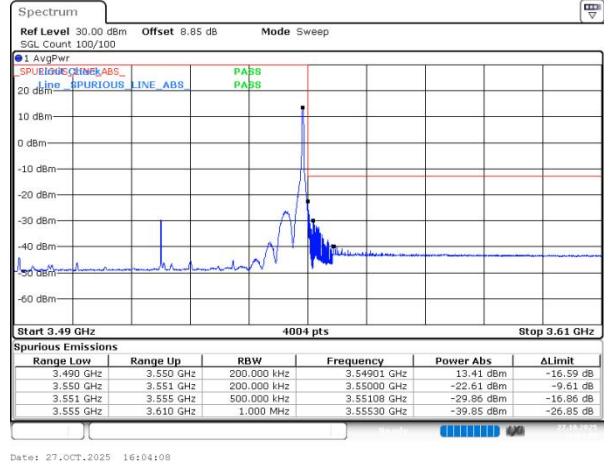
n78(3450-3550) SCS=30kHz DFT_64QAM BW=60MHz HighChannel=634666 RB=1@161
