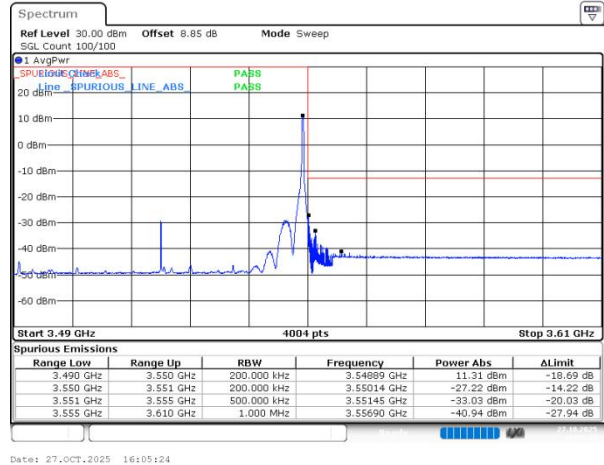
n78(3450-3550) SCS=30kHz DFT_256QAM BW=60MHz HighChannel=634666 RB=1@161
