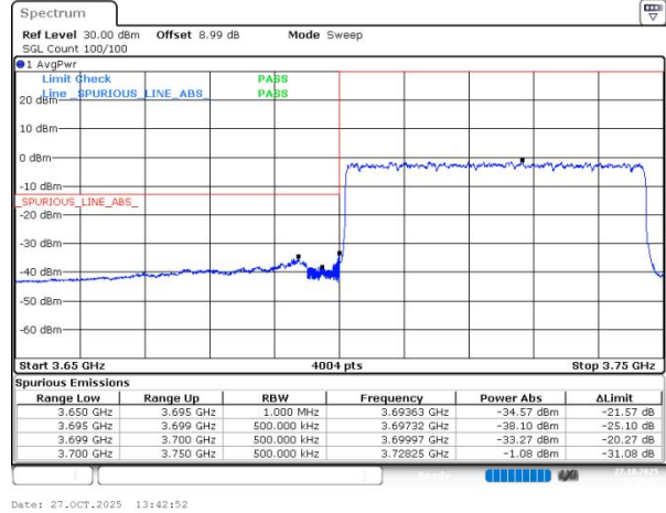
n77(3700-3980) SCS=30kHz DFT_QPSK BW=50MHz LowChannel=648334 RB=128@0
