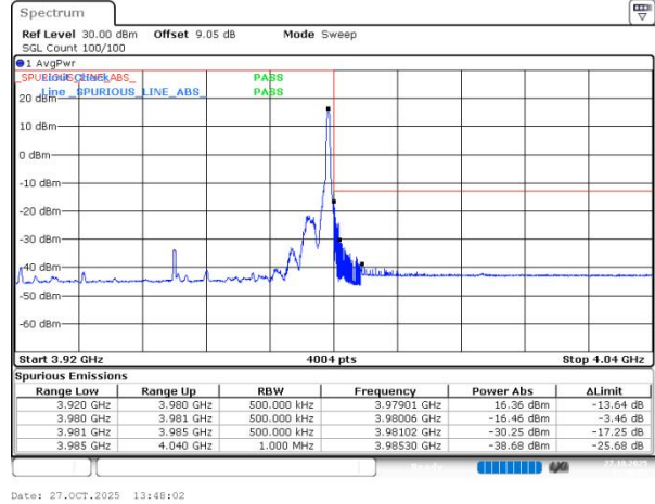
n77(3700-3980) SCS=30kHz DFT_BPSK BW=60MHz HighChannel=663332 RB=1@161
