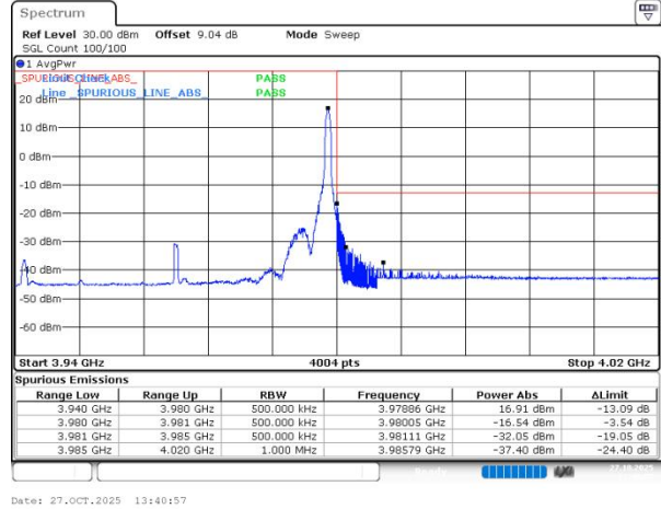
n77(3700-3980) SCS=30kHz DFT_QPSK BW=40MHz HighChannel=664000 RB=1@105
