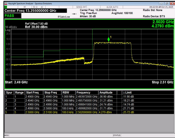
n7 SCS=15kHz DFT_64QAM BW=5MHz LowChannel=500500 RB=25@0
