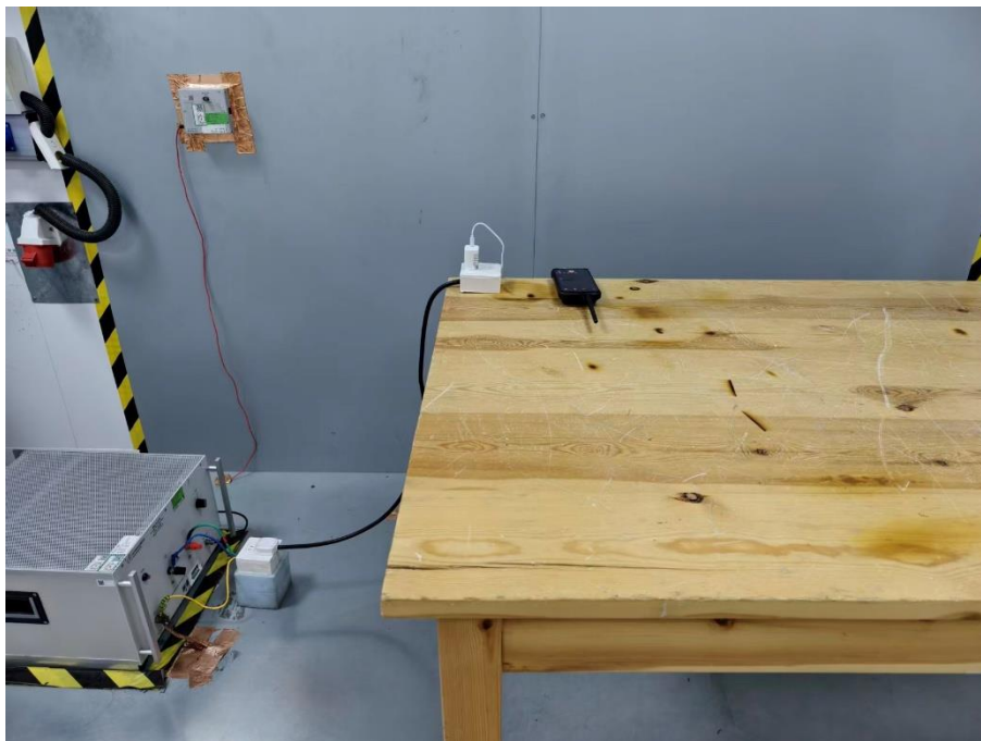
Set-up for Radiated Emission (RE), Below 1GHz
