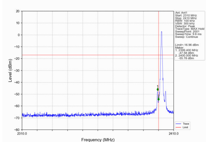
GFSK_DH5_LCH_2402MHz_Ant1_NTNV
