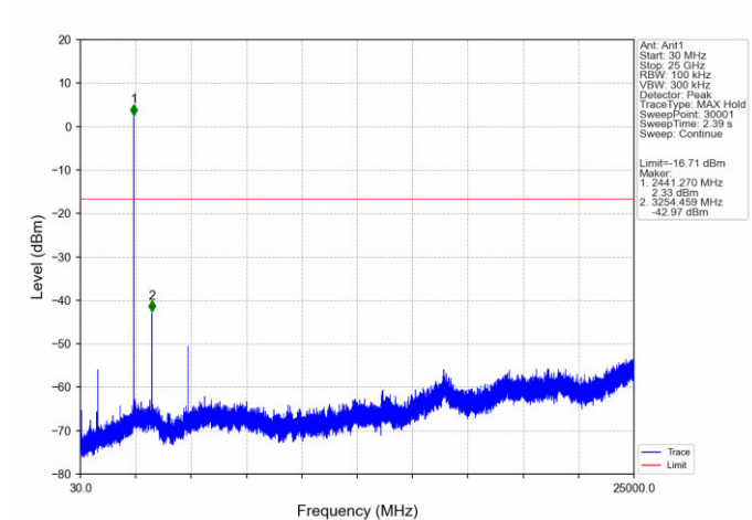
GFSK_DH5_MCH_2441MHz_Ant1_NTNV
