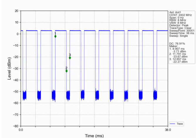
GFSK_DH5_LCH_2402MHz_Ant1_NTNV
