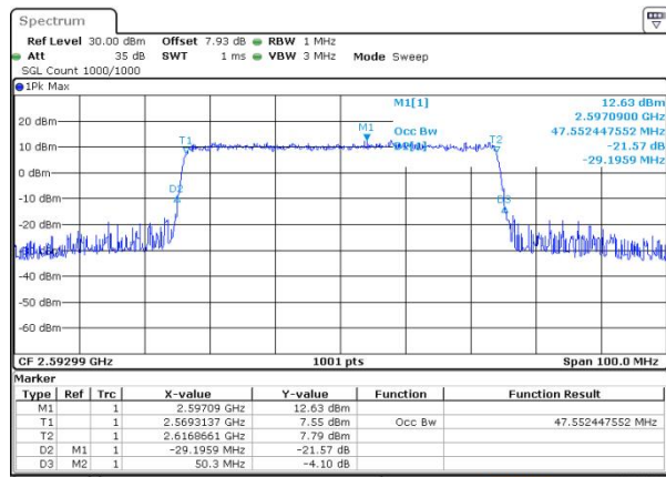
n41 SCS=30kHz CP_16QAM BW=50MHz Channel=518598 RB=133@0
