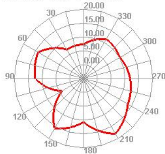
Wifi 13 TRP Phi=45
