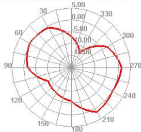
Bluetooth 0 TRP Phi=45
