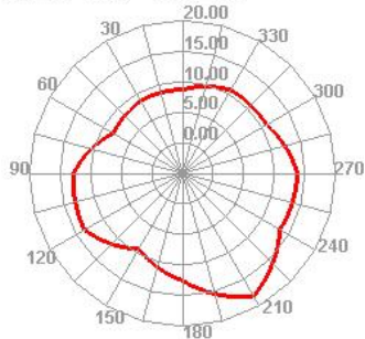
Wifi 1 TRP Phi=45
