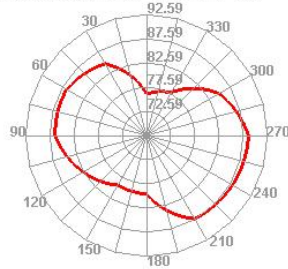
Bluetooth 78 TIS Phi=45
