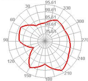
Wifi 13 TIS Phi=45
