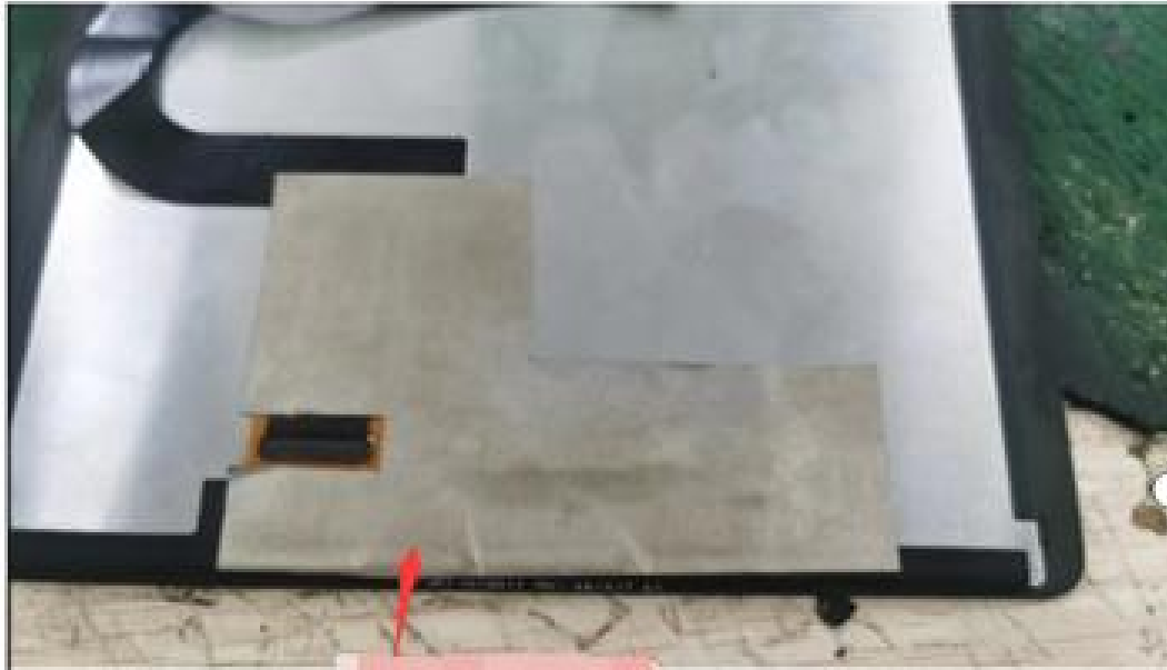
Shielding of screen cables with conductive cloth
