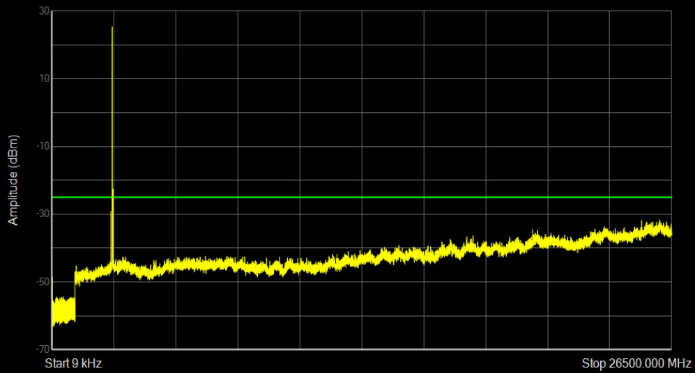
Band41 16QAM BW=5MHz Channel=40640 RB Size=1 Position=#0
