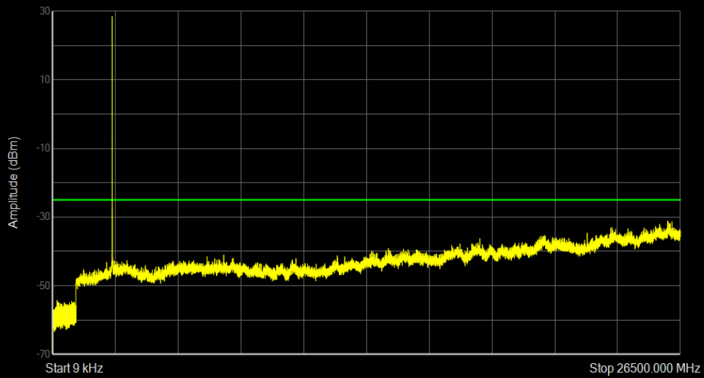
Band7 QPSK BW=5MHz Channel=21100 RB Size=1 Position=#0
