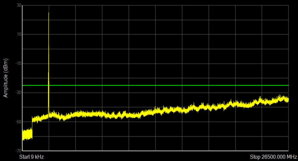
Band41 QPSK BW=20MHz Channel=41090 RB Size=1 Position=#0
