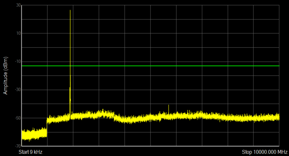
Band25 16QAM BW=10MHz Channel=26640 RB Size=1 Position=#0
