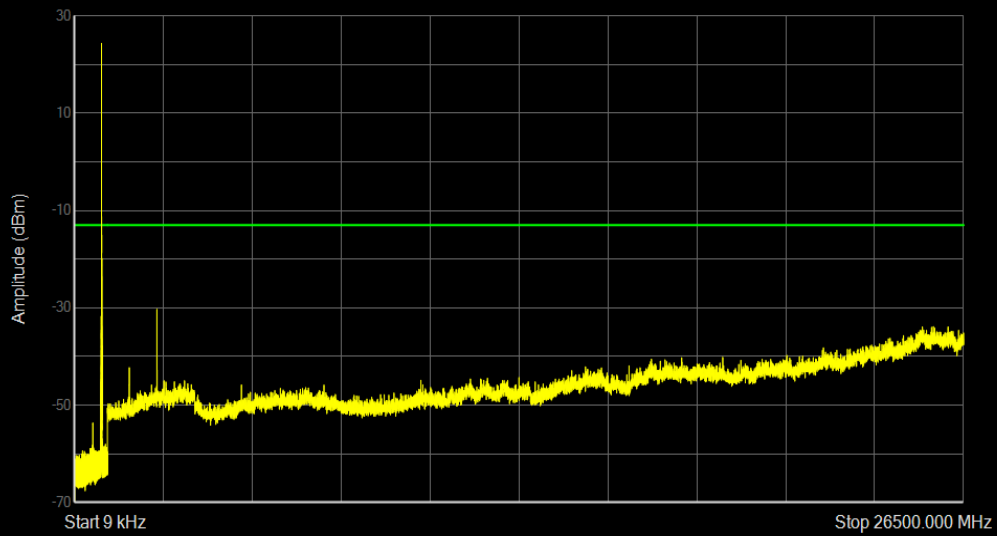
Band5 16QAM BW=10MHz Channel=20450 RB Size=1 Position=#0
