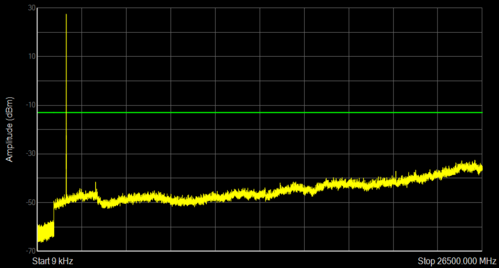
Band66 16QAM BW=5MHz Channel=132322 RB Size=1 Position=#0
