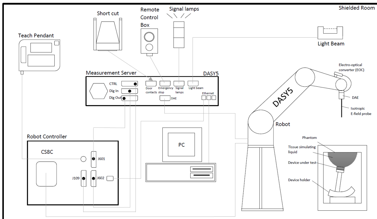
Figure 3 Schematic Laboratory Picture
