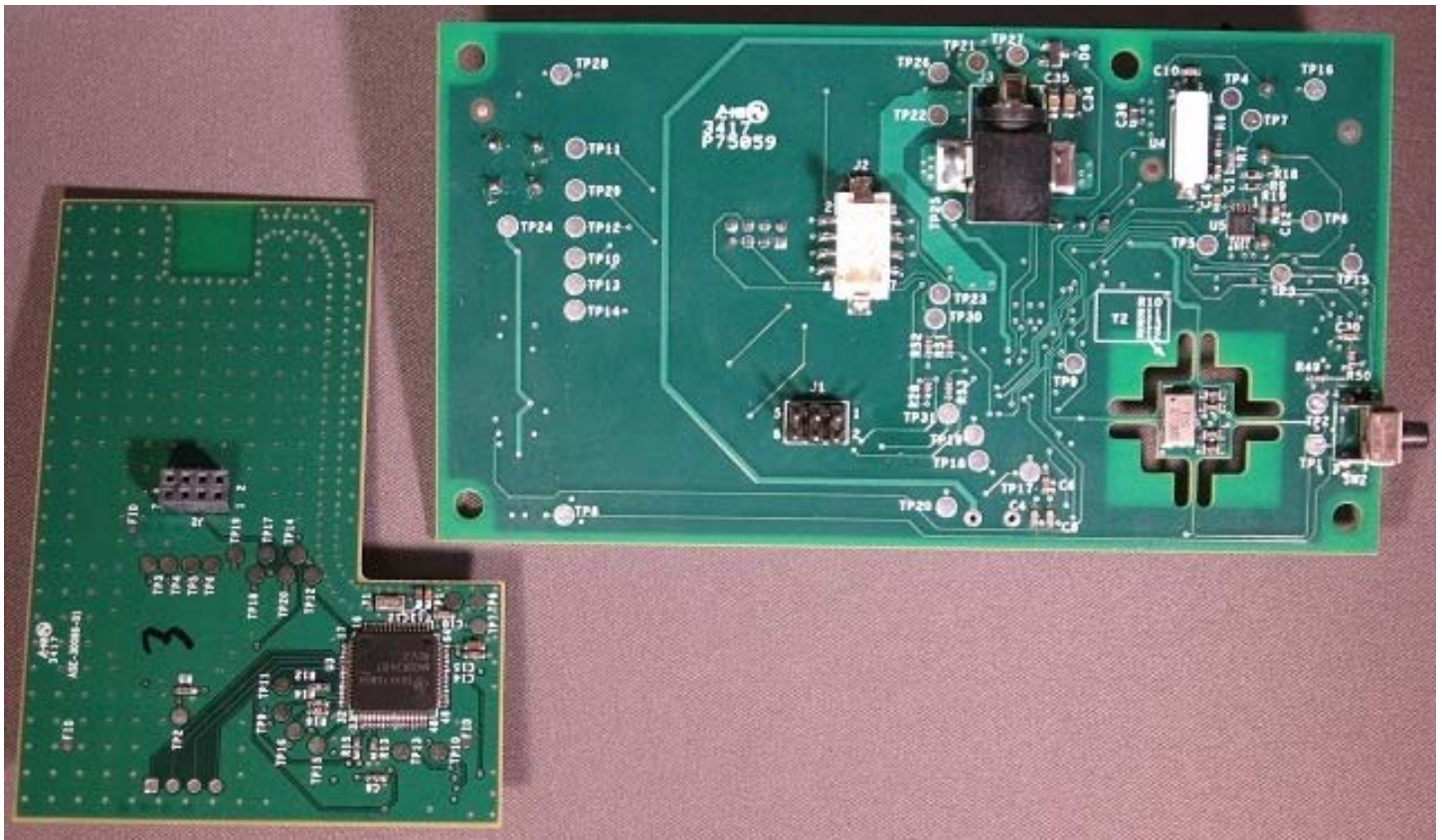
Bottom View of Boards
