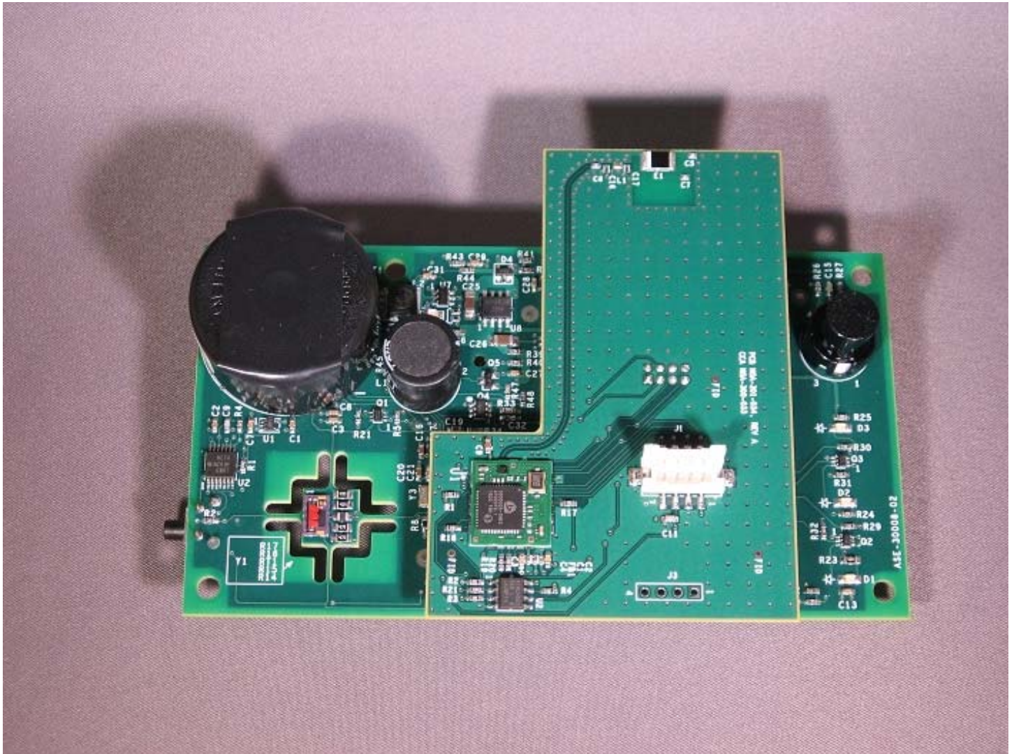
Assembled Main and Daughter (RF) Boards
