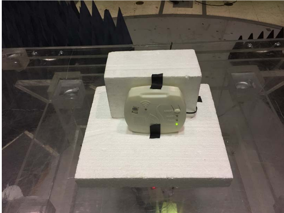
Radiated Emissions; Power, Spurious and Bandwidth; Front
