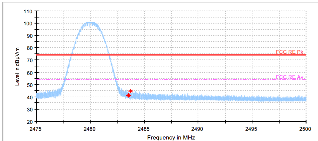
Left, BLE 500kbps, Highest Channel (2 480 MHz)_Peak
