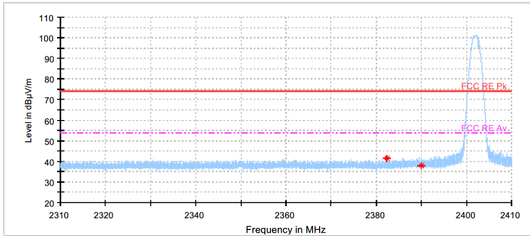
Left, BLE 500kbps, Lowest Channel (2 402 MHz)_Peak
