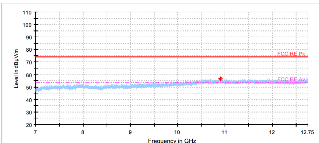
Left, BLE 500kbps, Highest Channel (2 480 MHz) : 7 GHz to 12.75 GHz_Average
