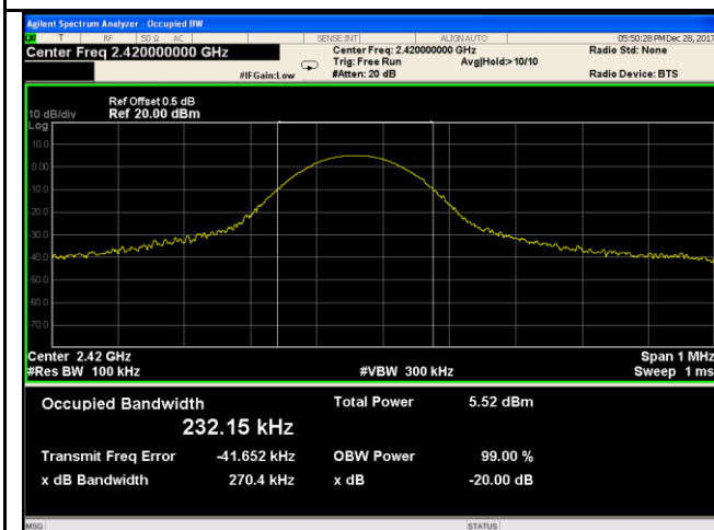
20dB Bandwidth - High CH 2420
