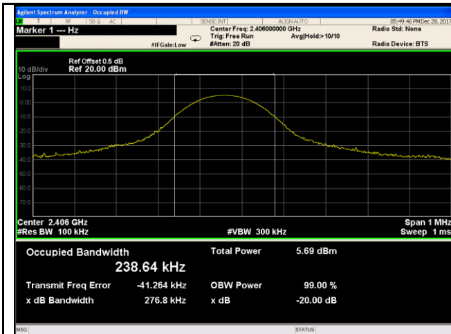
20dB Bandwidth - Low CH 2406
