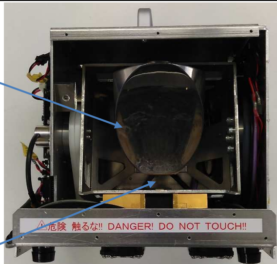
Front side ( radome, cover & radio wave absorber removed)
