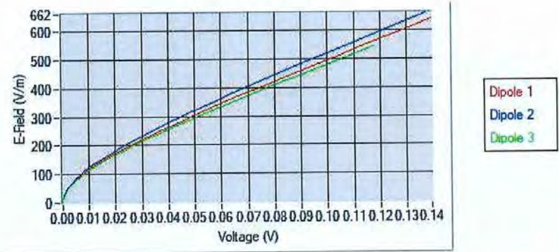
Calibration curves
