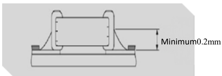
The optimal solder fillet amounts for re-flow soldering
