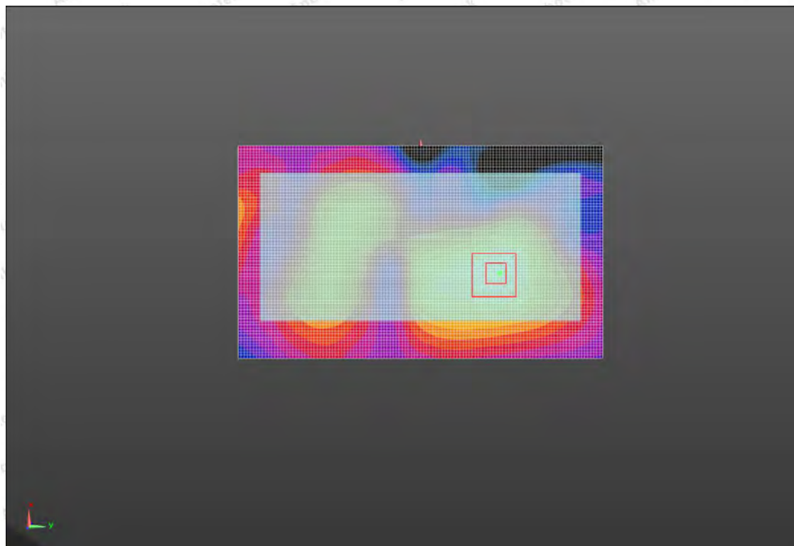
Figure 13: WLAN 2.4G_Rear side_0mm
