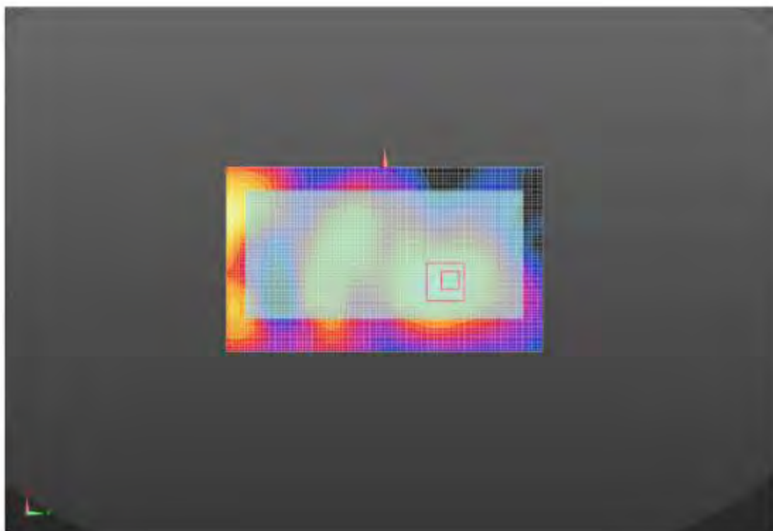
Figure 10: LTE Band 41_QPSK_Rear side
