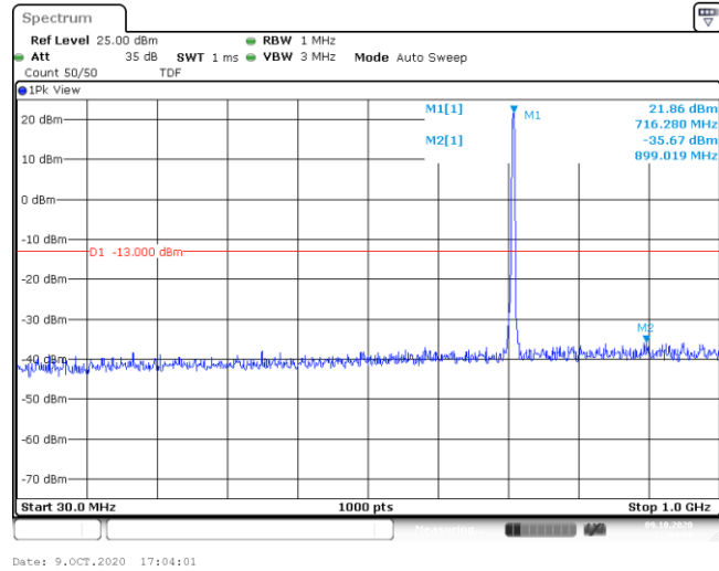
Band12-3MHz-16QAM-23165-15RB#0-Range1:30~1000MHz--35.67-PASS
