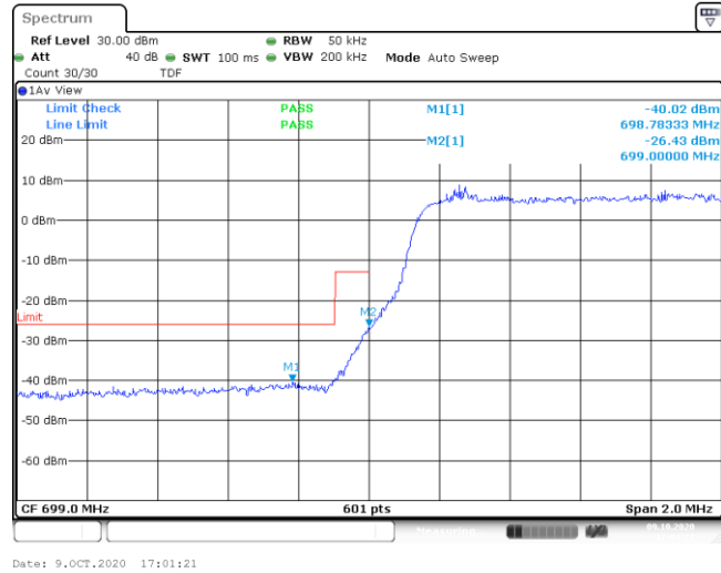
Band12-3MHz-QPSK-23025-15RB#0--40.02,-26.43-PASS
