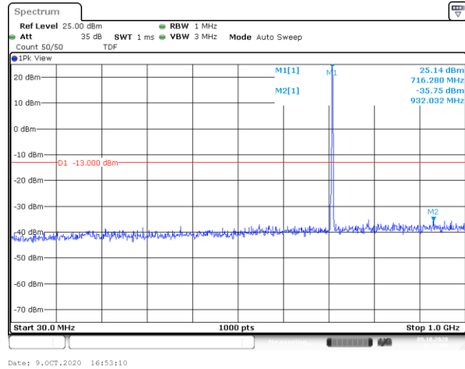
Band12-1.4MHz-16QAM-23173-6RB#0-Range1:30~1000MHz--35.75-PASS
