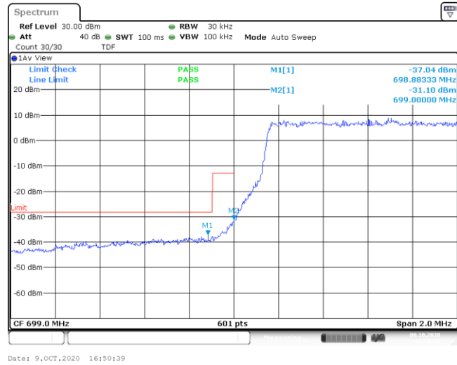
Band12-1.4MHz-16QAM-23017-6RB#0--37.04,-31.10-PASS
