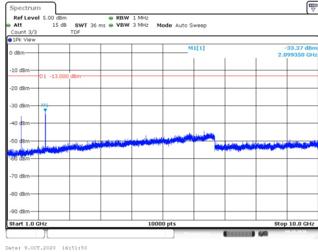
Band12-1.4MHz-16QAM-23017-6RB#0-Range2:1000~10000MHz--33.37-PASS
