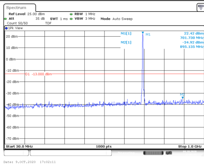
Band12-3MHz-QPSK-23025-15RB#0-Range1:30~1000MHz--34.92-PASS
