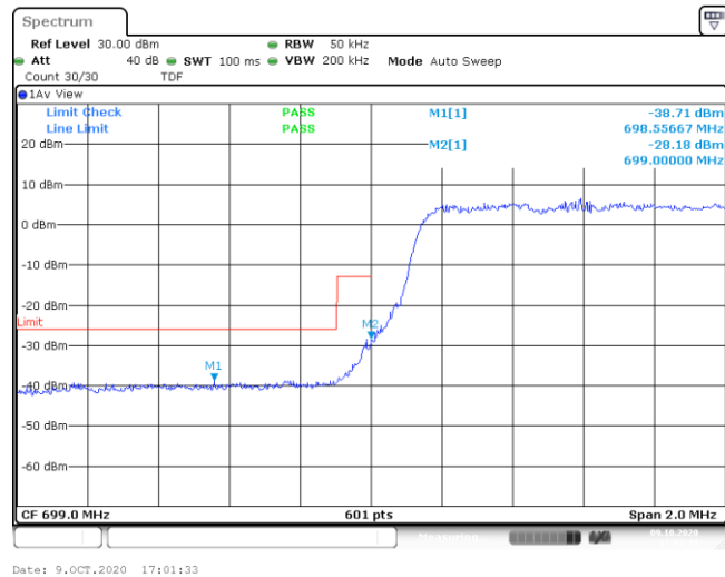
Band12-3MHz-16QAM-23025-15RB#0--38.71,-28.18-PASS
