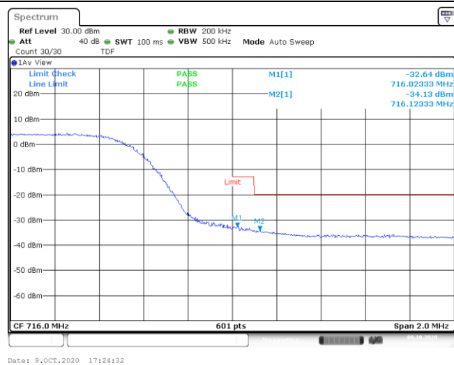
Band12-10MHz-16QAM-23130-50RB#0--32.64,-34.13-PASS
