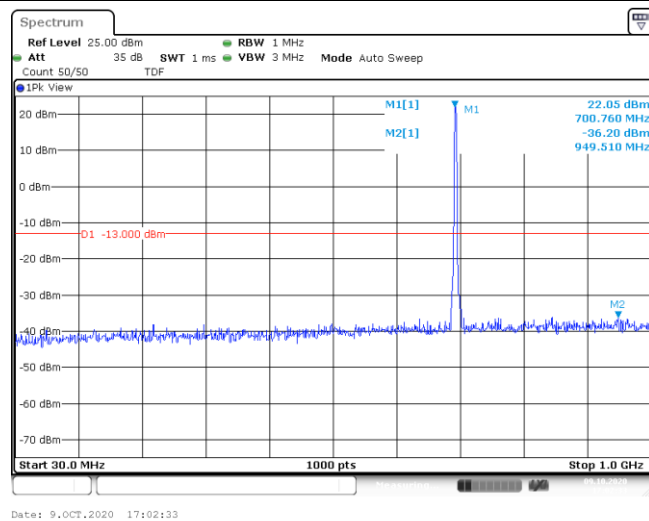
Band12-3MHz-16QAM-23025-15RB#0-Range1:30~1000MHz--36.2-PASS
