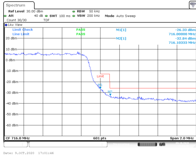
Band12-3MHz-QPSK-23165-15RB#0--26.33,-32.84-PASS
