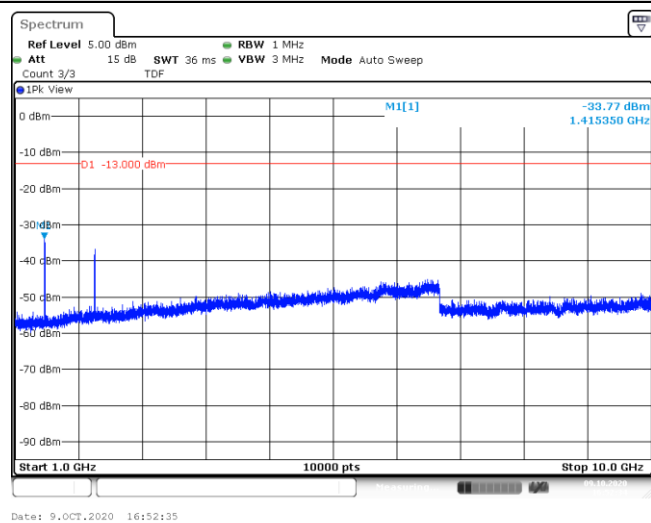
Band12-1.4MHz-16QAM-23095-6RB#0-Range2:1000~10000MHz--33.77-PASS
