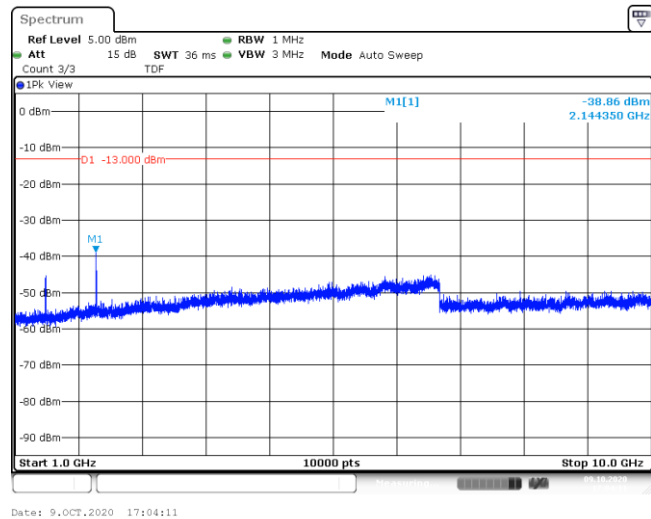
Band12-3MHz-16QAM-23165-15RB#0-Range2:1000~10000MHz--38.86-PASS
