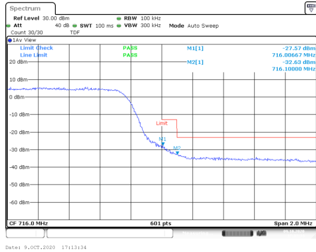
Band12-5MHz-16QAM-23155-25RB#0--27.57,-32.63-PASS
