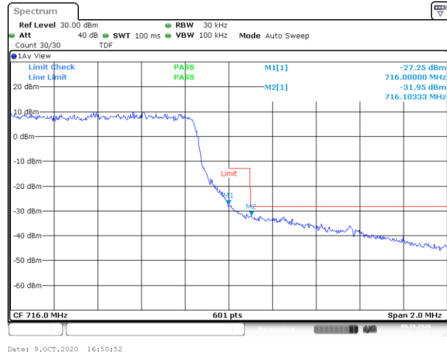
Band12-1.4MHz-QPSK-23173-6RB#0--27.25,-31.95-PASS
