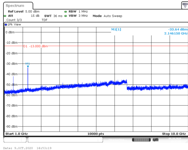
Band12-1.4MHz-16QAM-23173-6RB#0-Range2:1000~10000MHz--33.64-PASS
