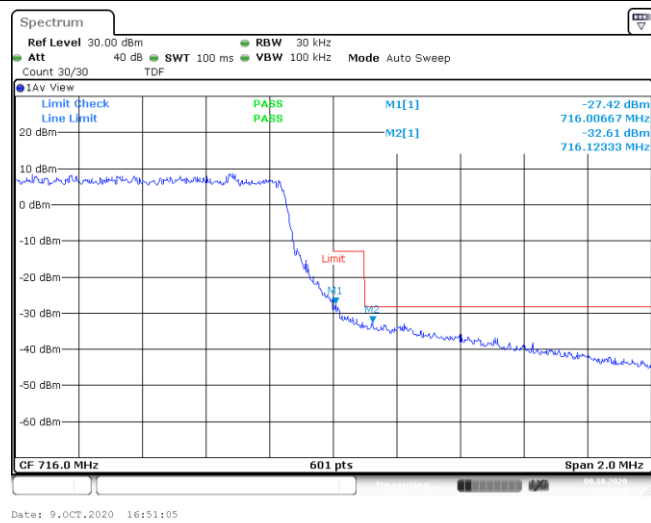
Band12-1.4MHz-16QAM-23173-6RB#0--27.42,-32.61-PASS
