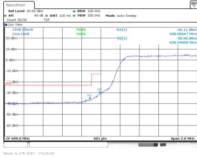
Band12-5MHz-16QAM-23035-25RB#0--36.11,-30.68-PASS
