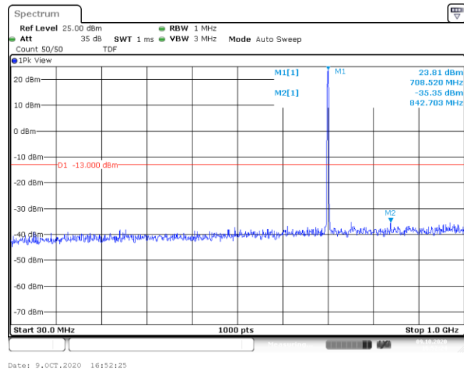
Band12-1.4MHz-16QAM-23095-6RB#0-Range1:30~1000MHz--35.35-PASS
