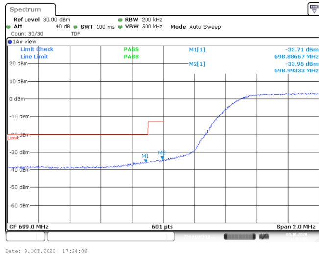
Band12-10MHz-16QAM-23060-50RB#0--35.71,-33.95-PASS
