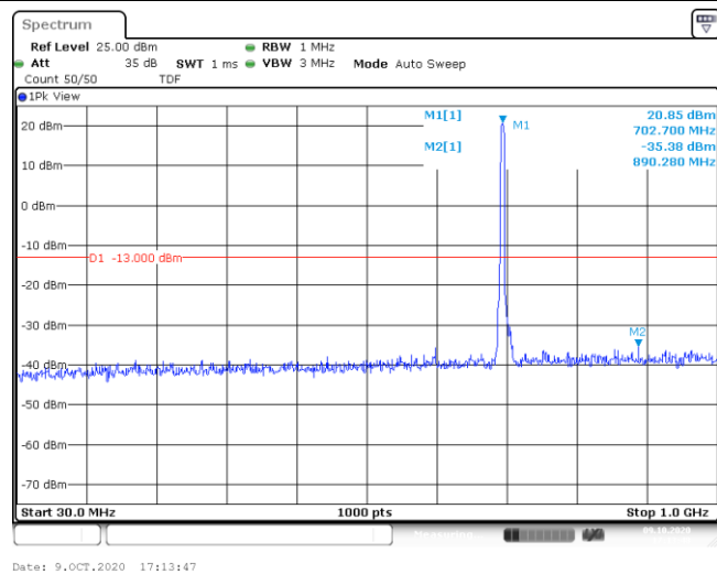
Band12-5MHz-QPSK-23035-25RB#0-Range1:30~1000MHz--35.38-PASS
