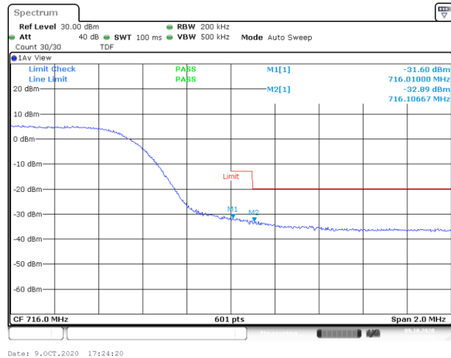
Band12-10MHz-QPSK-23130-50RB#0--31.60,-32.89-PASS
