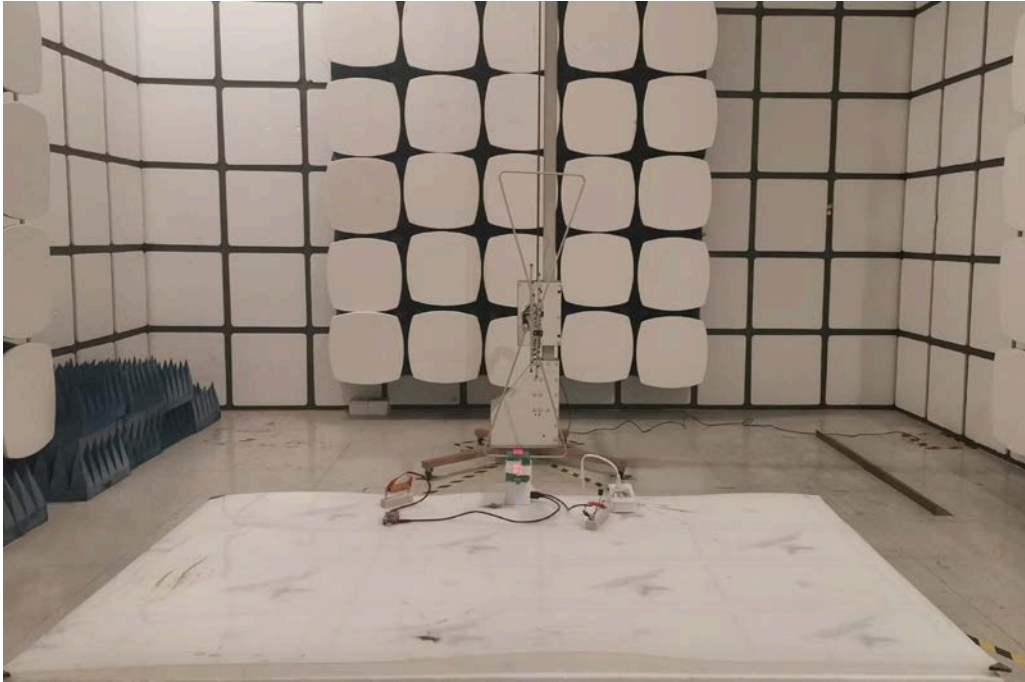
Spurious Emission Test Setup (Between 30MHz – 1GHz)
