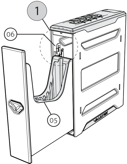
05. Pistol Holster with Spare Magazine Slot 06. Mounting Plate Release Clip
