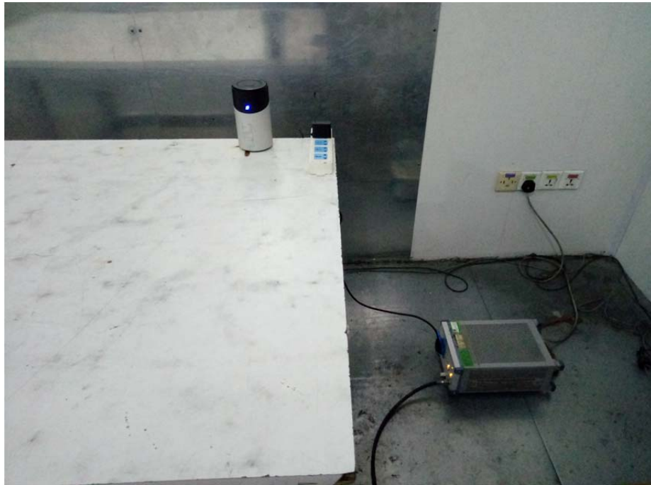
Conducted Emission
