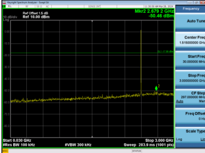
CH19 – 10th Harmonic of the fundamental frequency
