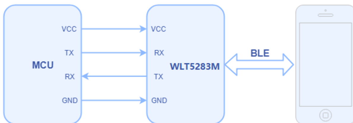
Figure 4-2: UART communication
